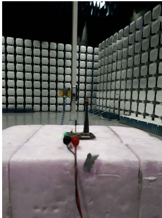
Radiated Emissions, 1 GHz – 10 GHz, as seen from EUT
