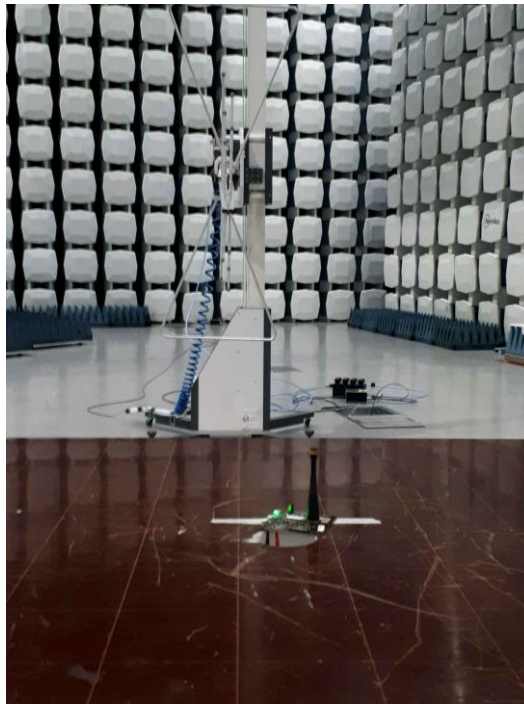
Radiated Emissions, 30 - 1000 MHz, as seen from EUT
