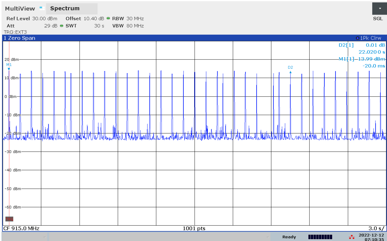
915 MHz: RF Burst
