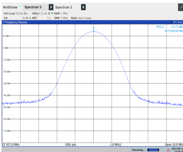
Conducted Peak Power, 927 MHz, FSK
