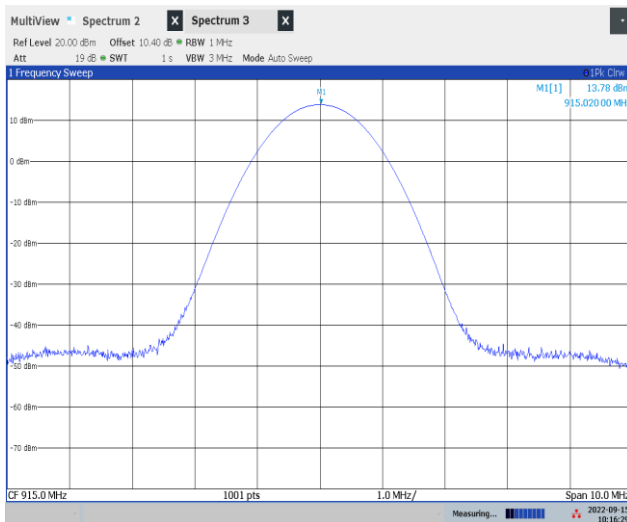
Conducted Peak Power, 915 MHz, FSK
