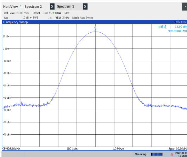
Conducted Peak Power, 903 MHz, FSK
