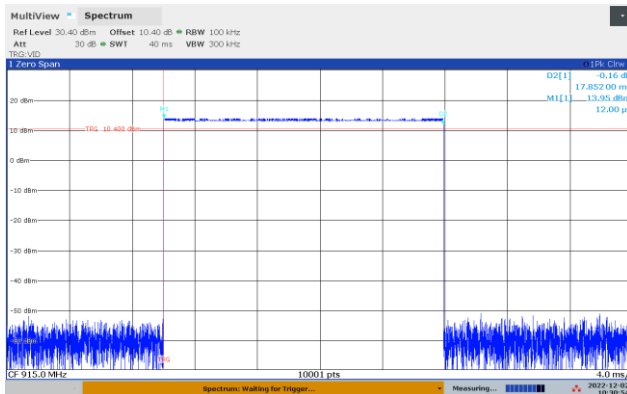
915 MHz: RF Burst
