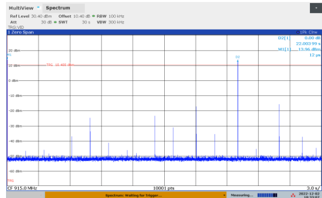
915 MHz: Frame
