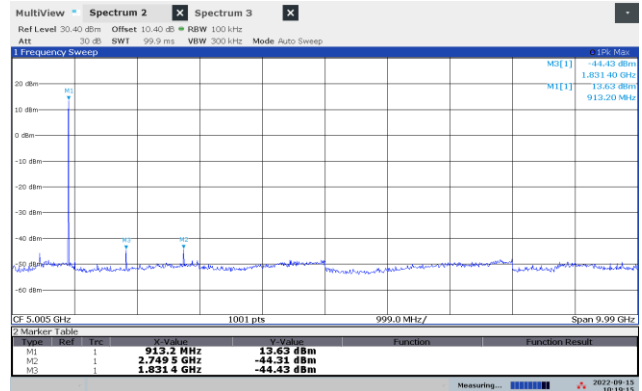
915 MHz: 10-10000 MHz
