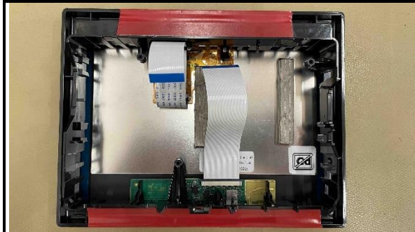
Figure 1-15: SC3L RadioBoard frontside
