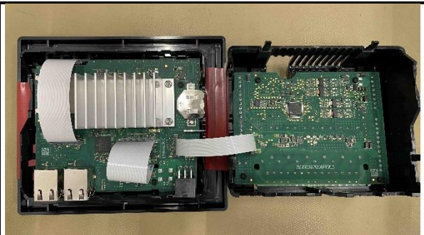
Figure 1-2: SC3S backside opened
