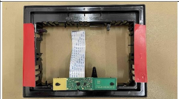
Figure 1-12: SC3M RadioBoard backside
