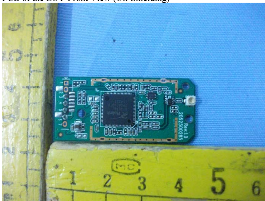
PCB of the EUT-Front View (Un-Shielding)
