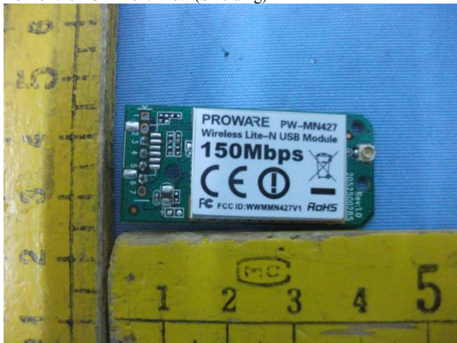
Figure 7 PCB of the EUT-Front View (Shielding)
