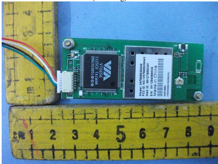
Figure 12 PCB of the EUT-Front View (Shielding)
