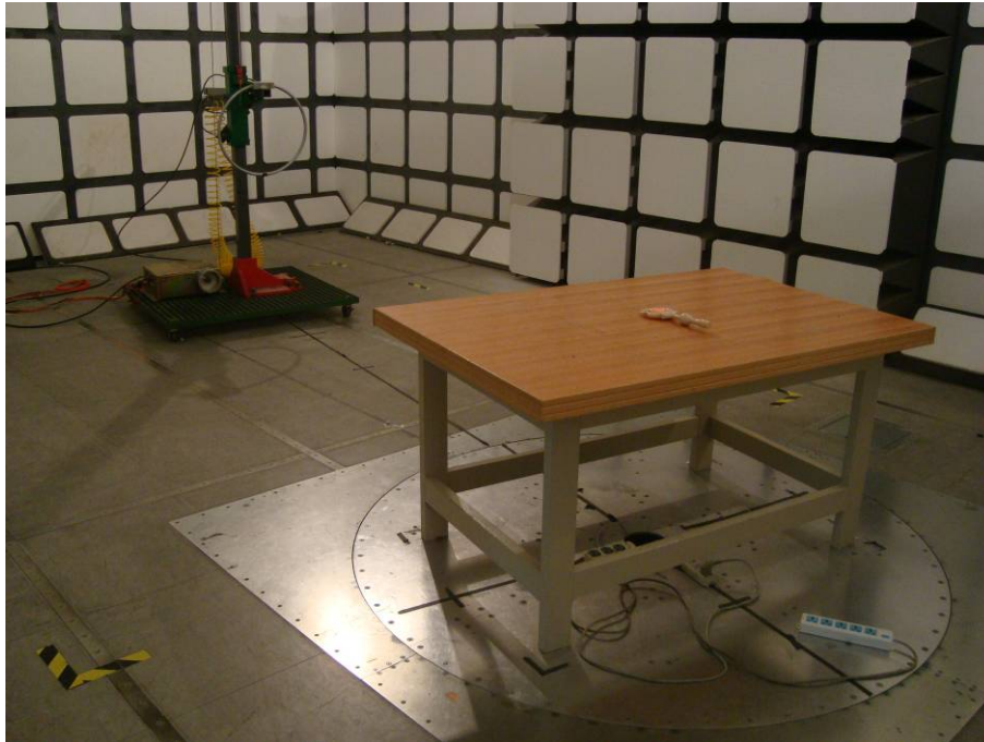
Radiated Emissions - Stand View (fundamental)
