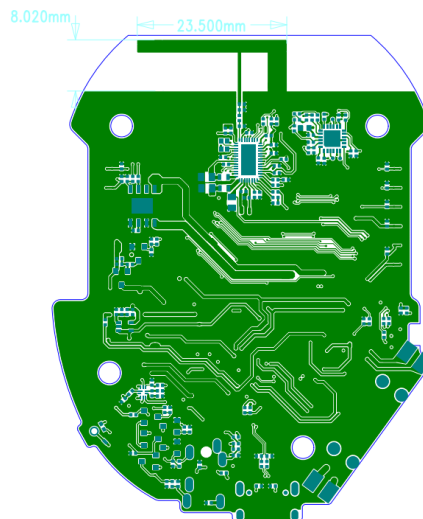
Antenna Dimensions
