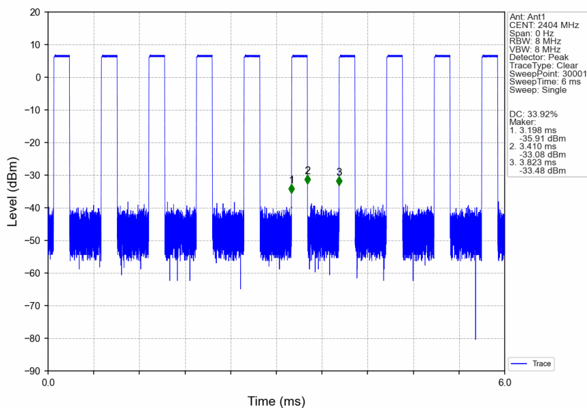
2M_LCH_2404MHz_Ant1_NTNV
