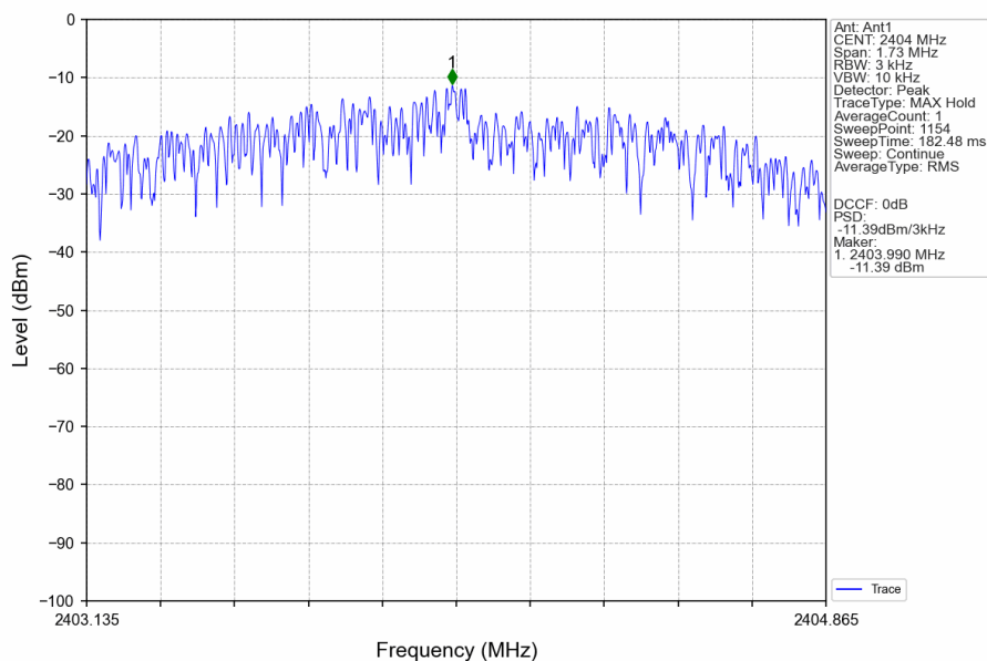
2M_LCH_2404MHz_Ant1_NTNV
