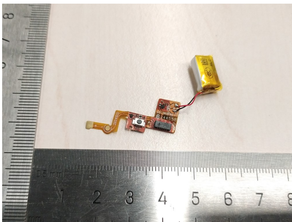
Fig. 12. Battery board view -1 (for right channel)
