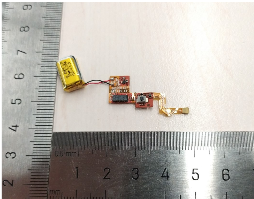
Fig. 4. Battery board view -1 (Left hannel)
