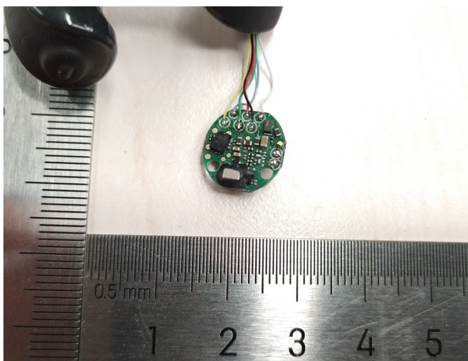
Fig. 8. Maiboard view -2 (Left hannel)
