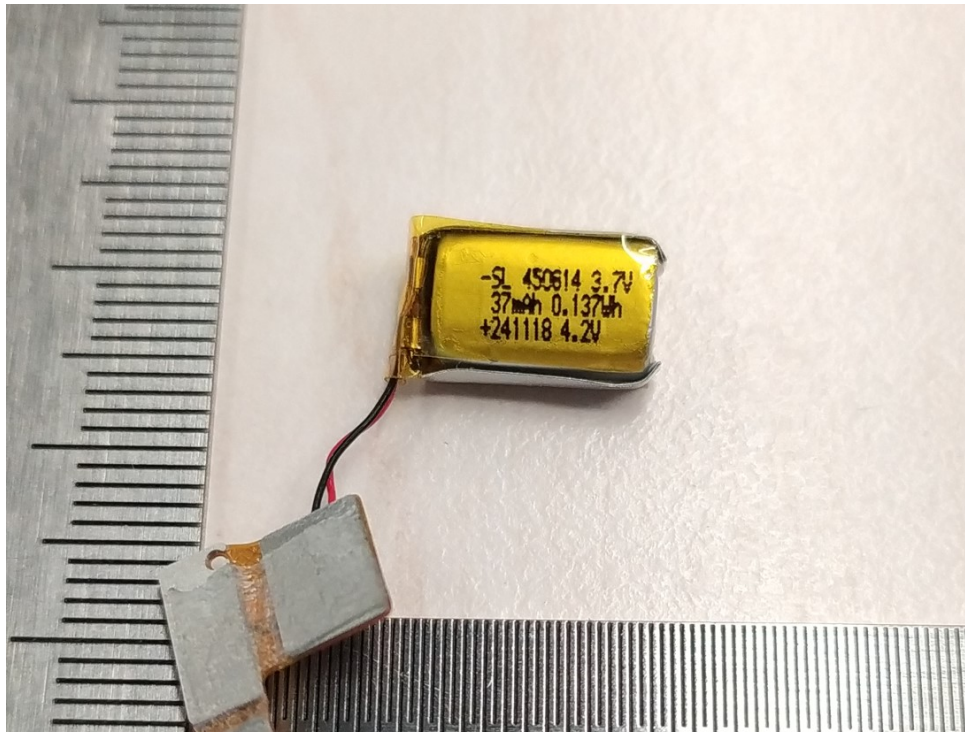
Fig. 17. Battery for both earbuds
