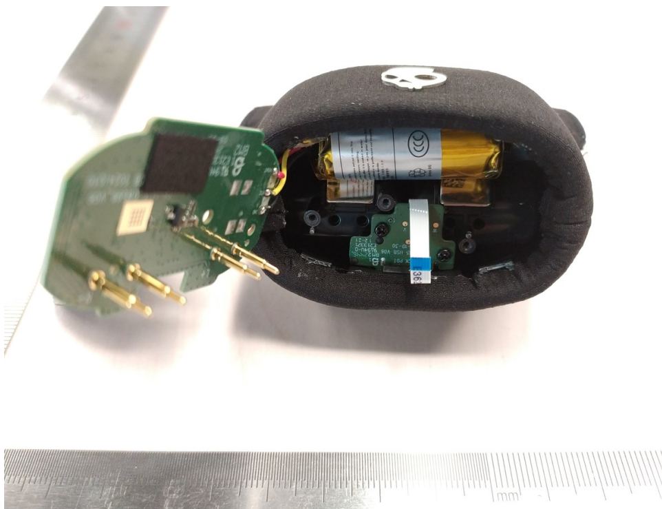
Fig. 4. Internal view -4
