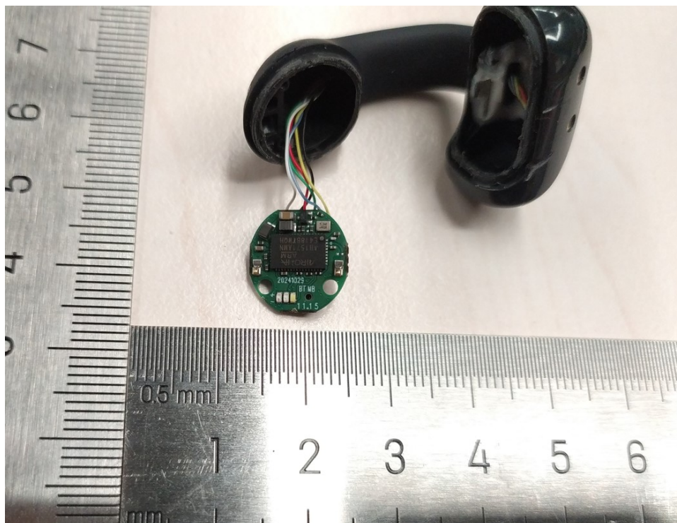
Fig. 7. Mainboard view -1 (Left hannel)
