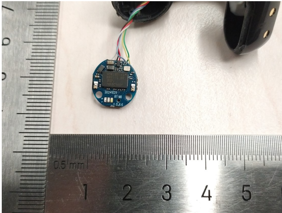
Fig. 15. Mainboard view -1 (for right channel)
