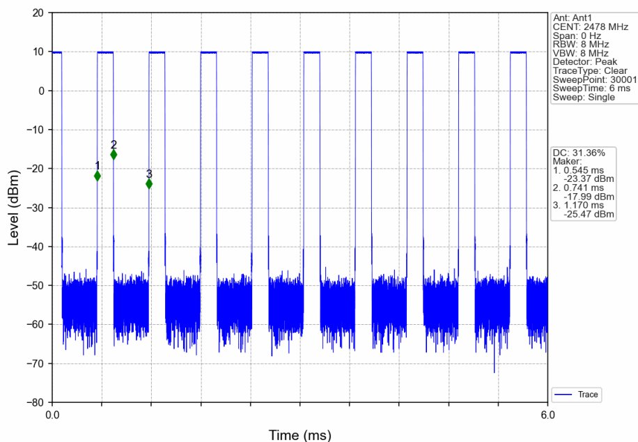
BLE-2M_HCH_2478MHz_Ant1_NTNV
