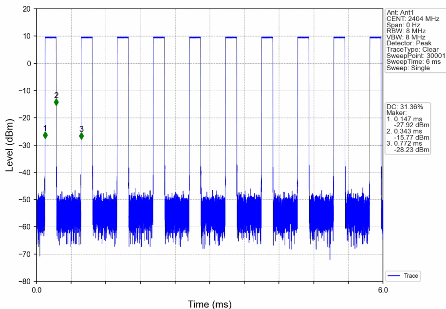
BLE-2M_LCH_2404MHz_Ant1_NTNV
