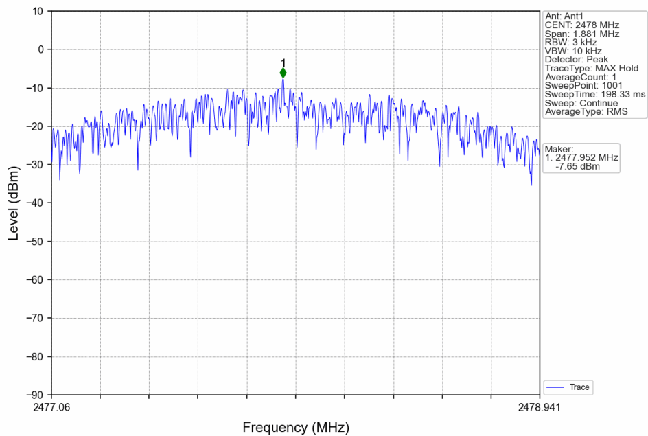
BLE-2M_HCH_2478MHz_Ant1_NTNV
