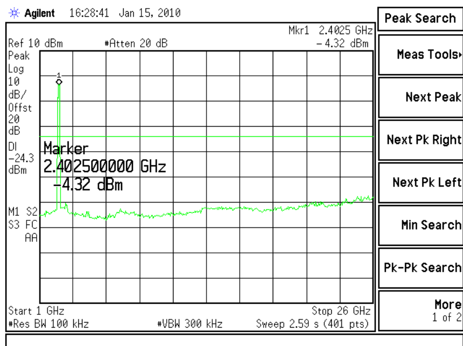
(Plot A.2: Channel = 0, 1GHz to 26GHz)
