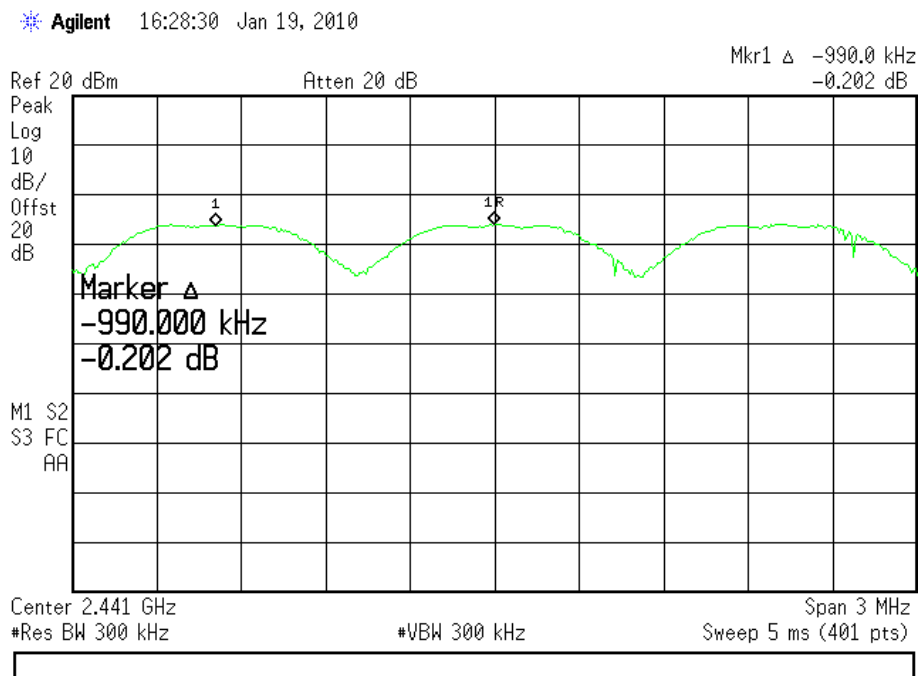
(Plot A: Carried Frequency Separation)
