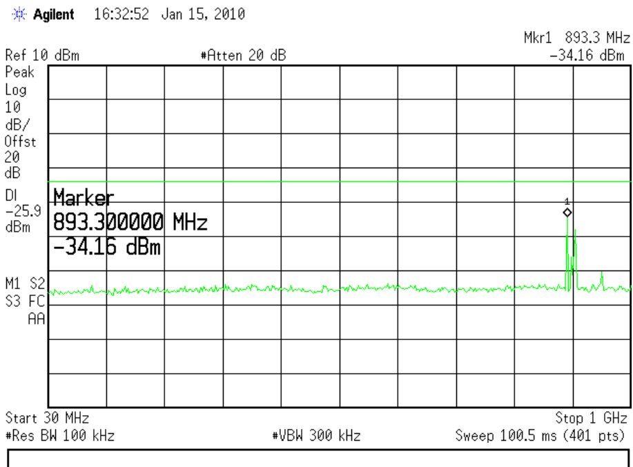
(Plot B.1: Channel = 39, 30MHz to 1GHz)
