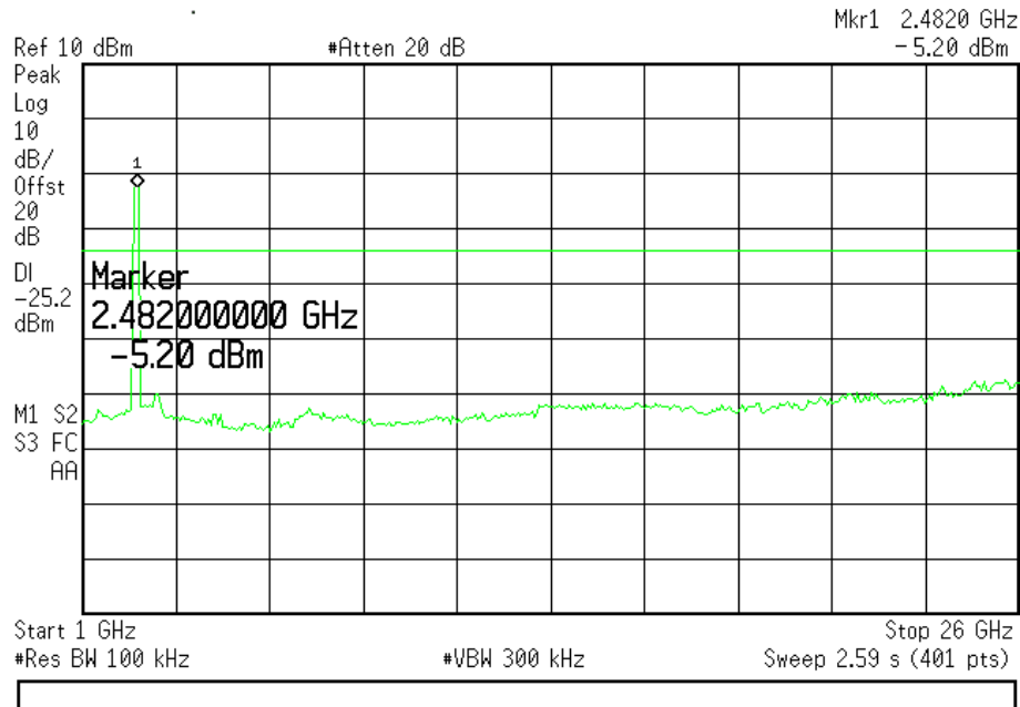
(Plot C.2: Channel = 78, 1GHz to 26GHz)
