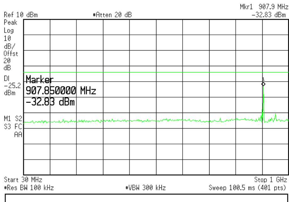
(Plot C.1: Channel = 78, 30MHz to 1GHz)
