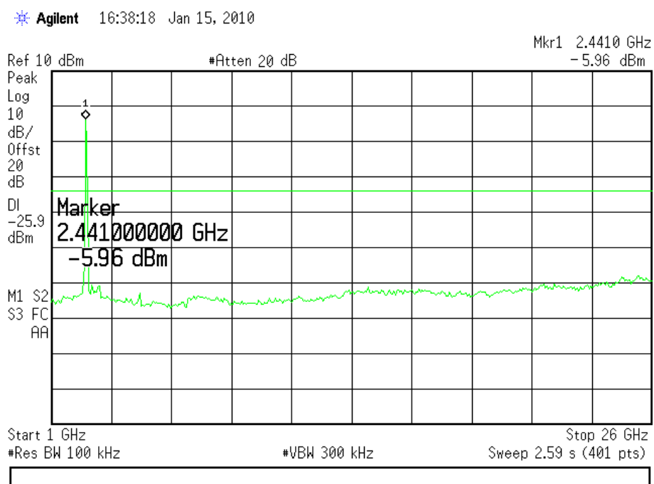
(Plot B.2: Channel = 39, 1GHz to 26GHz)
