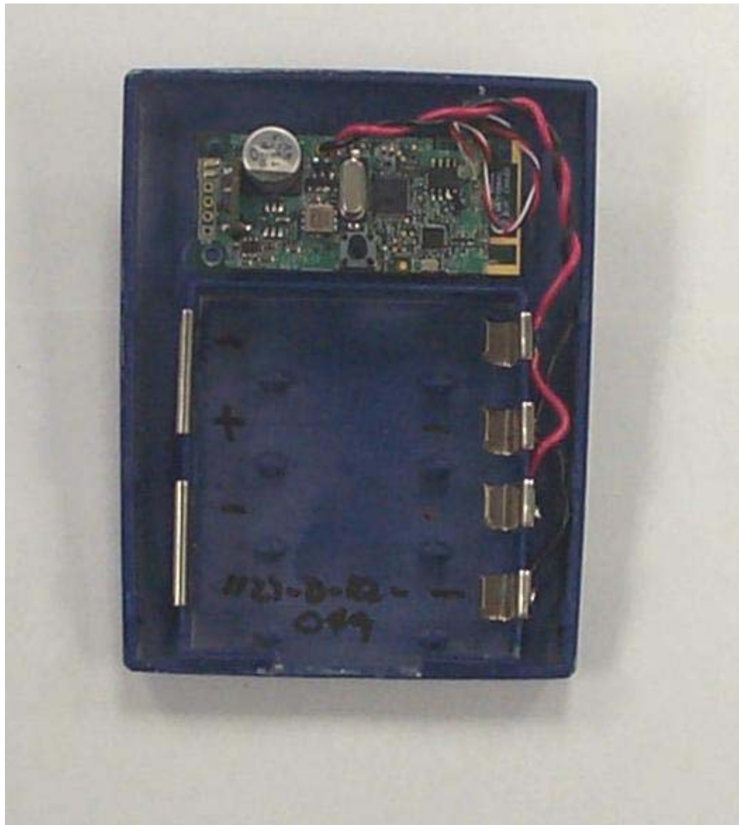
Top of Unit: Upper Cover removed
