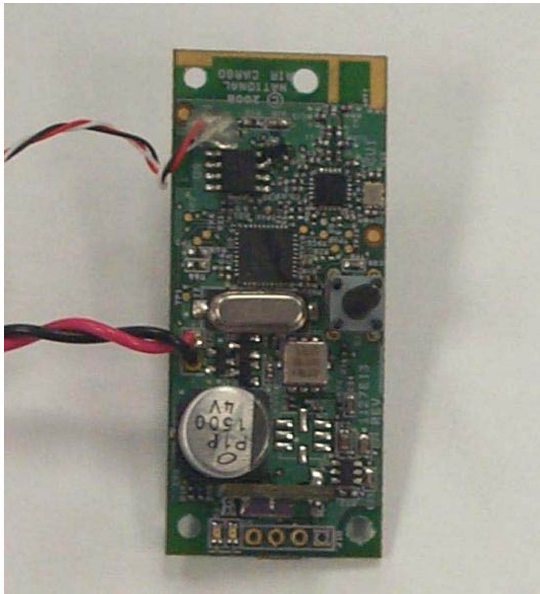
Component Side Sensor Board 1840-01-300
