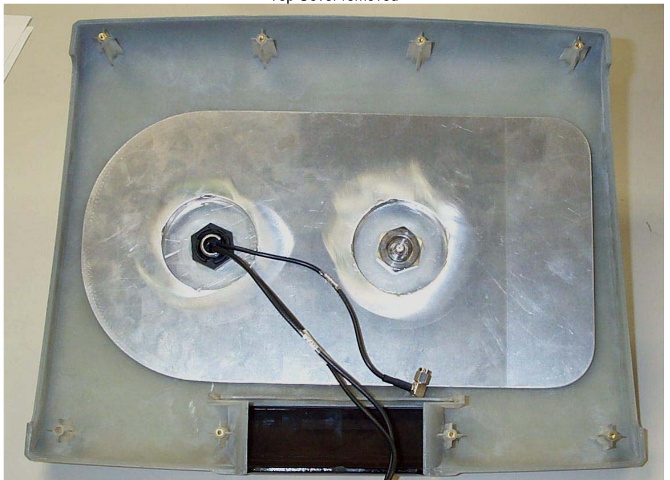
Inside of Top Cover
