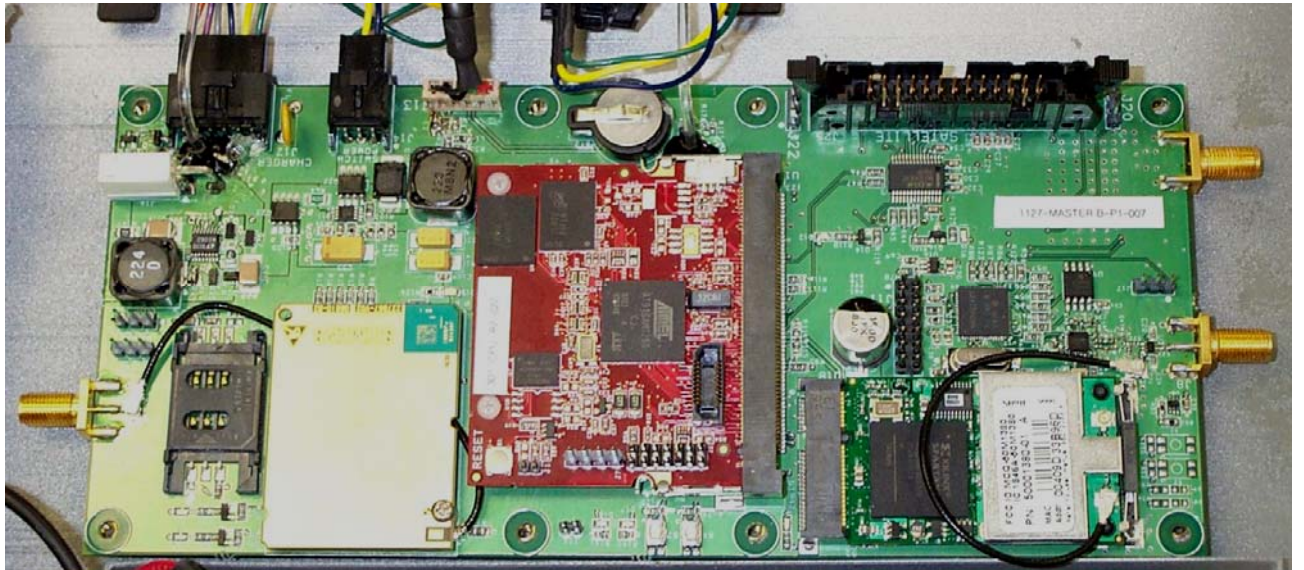
Component Side of Main Board
