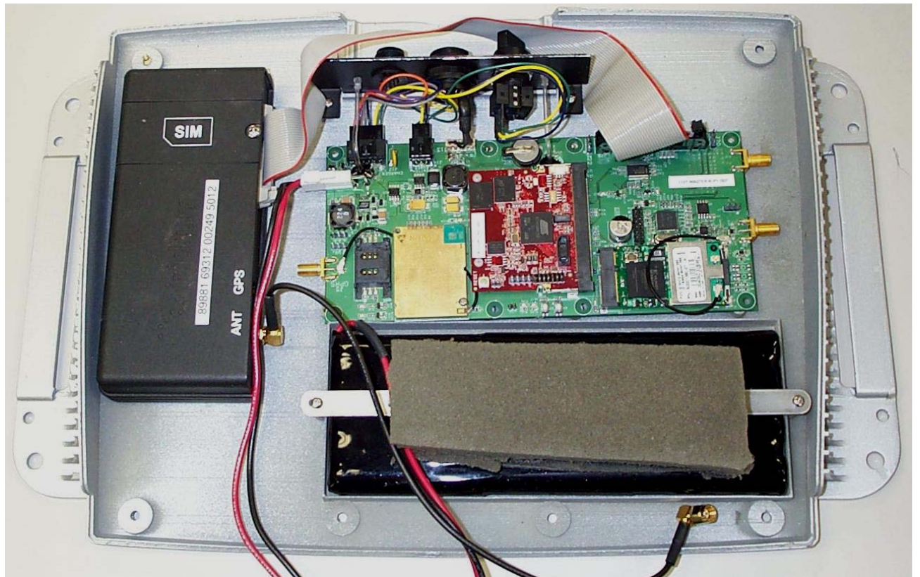
Top Cover removed
