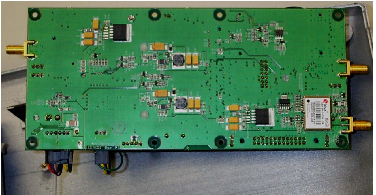
Foil Side of Main Board
