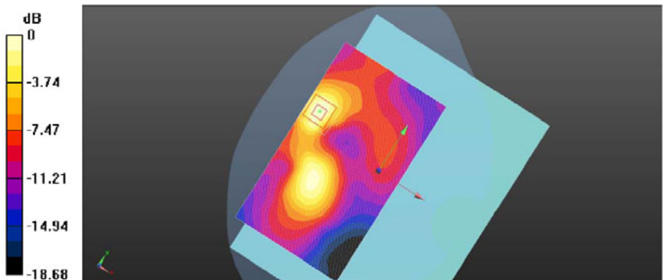
Plot 9: Body Top Side (GSM1900 GPRS 4TS Middle Channel)
