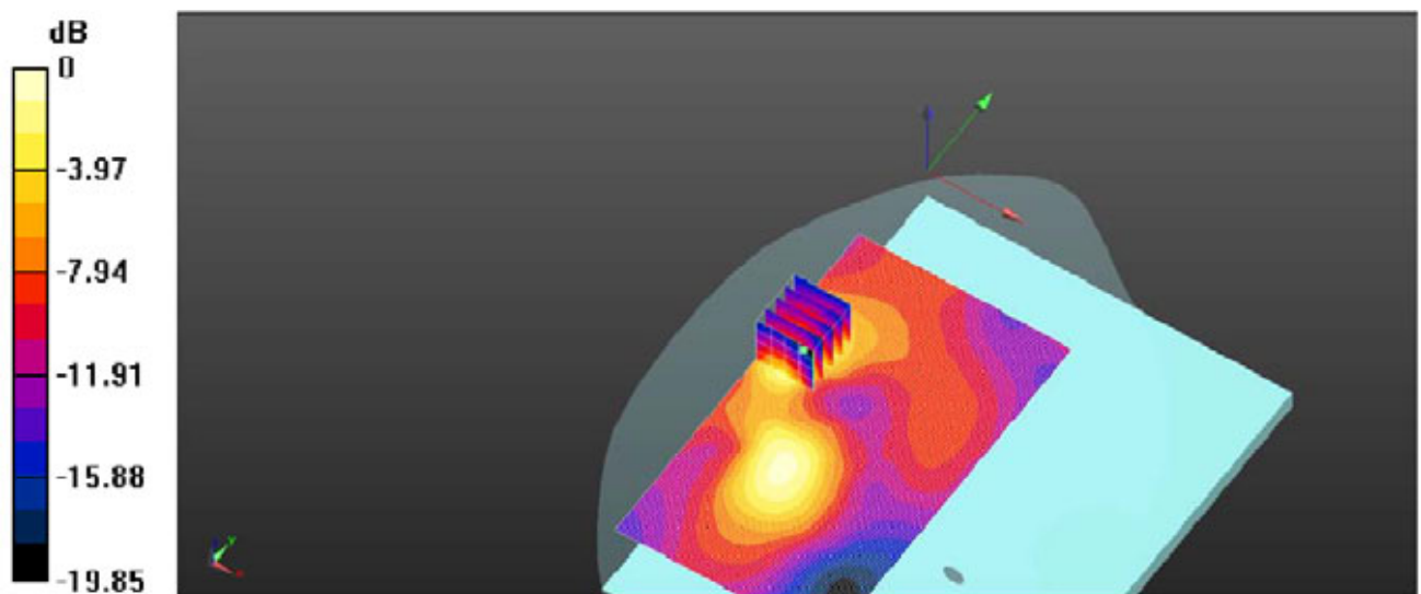
Plot 5: Body Rear Side (GSM850 EGPRS 4TS Middle Channel)
