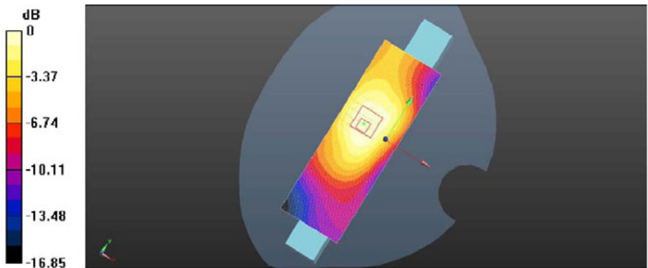
Plot 4: Body Top Side (GSM850 GPRS 4TS Middle Channel)
