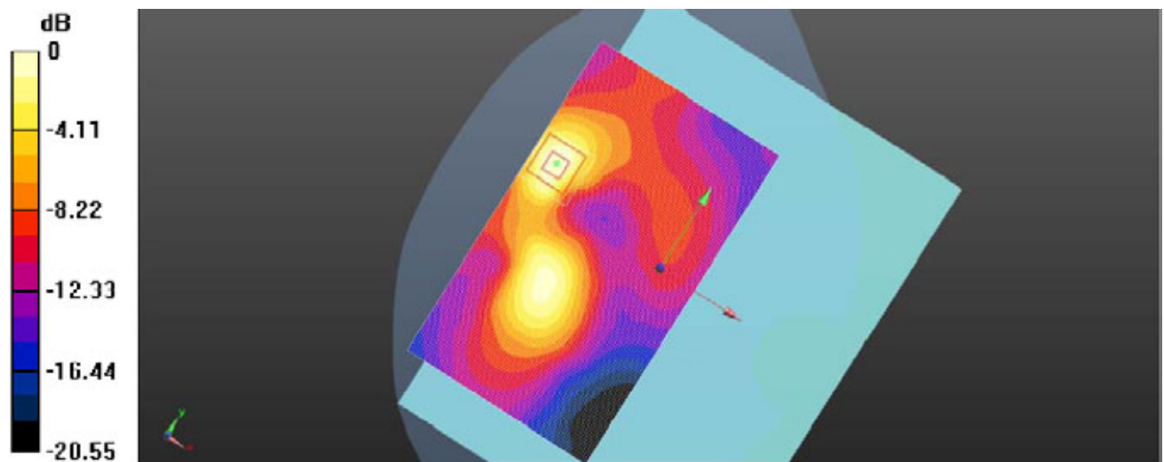
Plot 10: Body Rear Side (GSM1900 EGPRS 4TS Middle Channel)
