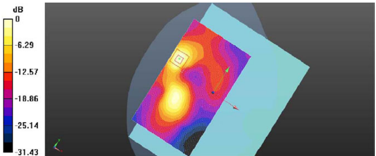
Plot 15: Body Rear Side (WCDMA Band V RMC Middle Channel)
