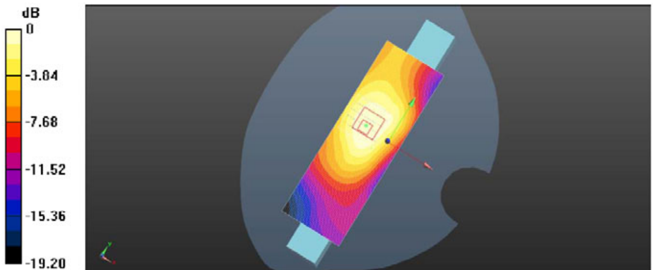
Plot 7: Body Left Side (GSM1900 GPRS 4TS Middle Channel)
