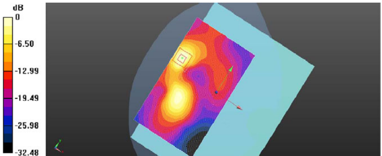
Plot 19: Body- worn Rear Side-802.11b-Channel 6-2437MHz(1Mbps)
