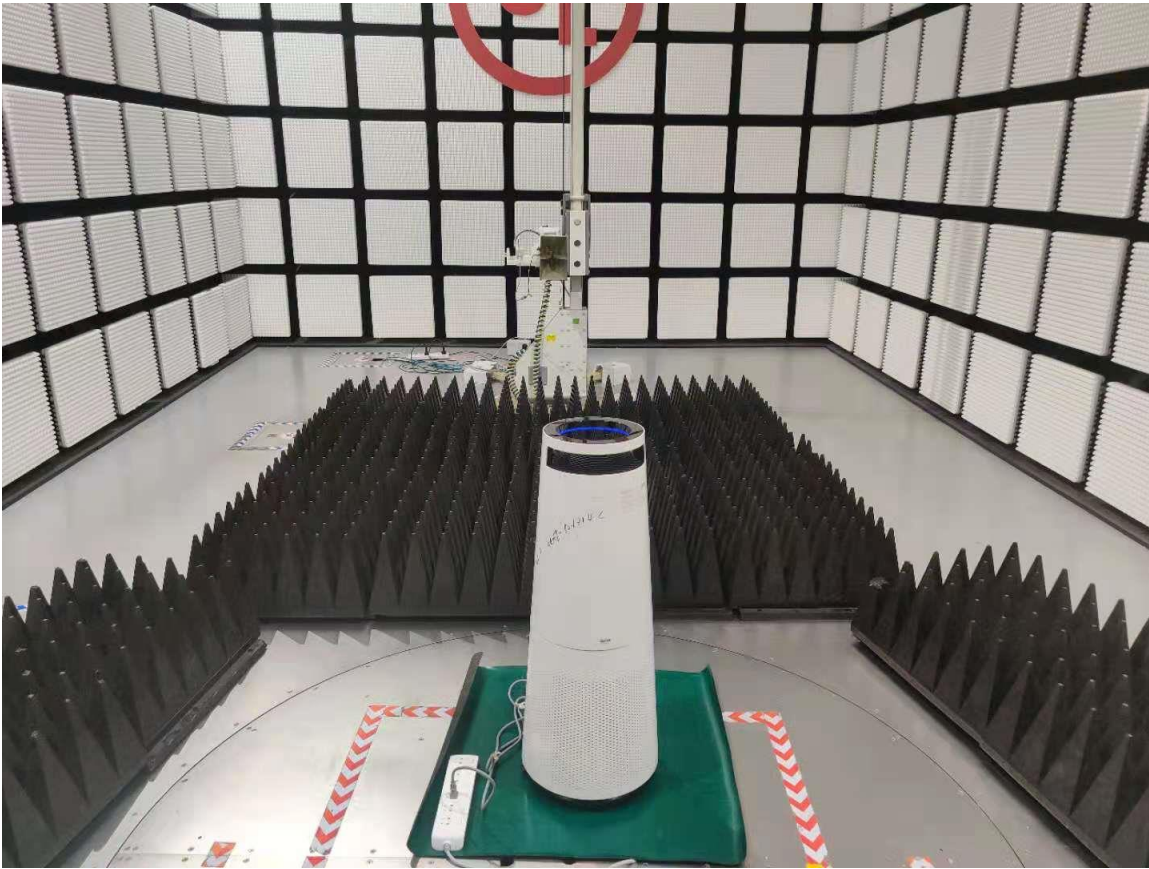
Radiated Disturbance Setup (Above 1GHz)
