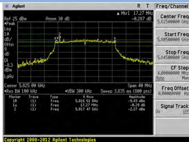
802.11ac20 Band IV HIGH CHANNEL
