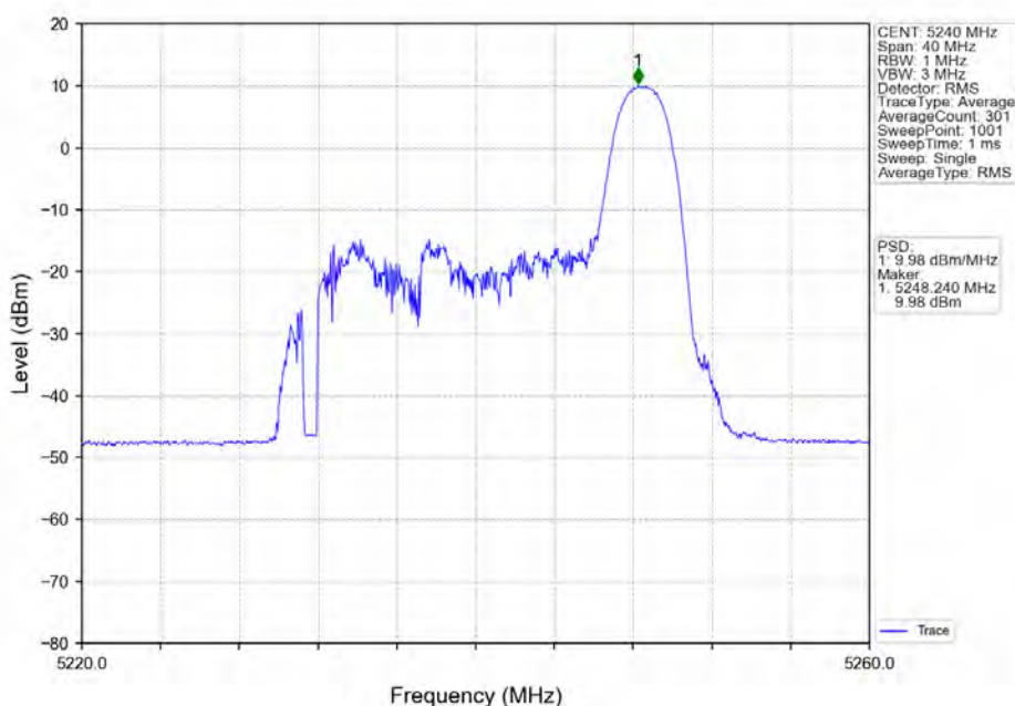
802.11ax(HE20)_HCH_5240MHz_RU26_Right_Ant2_NTNV
