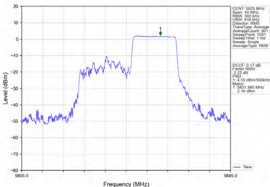
802.11ax(HE20)_HCH_5825MHz_RU106_Right_Ant1_NTNV
