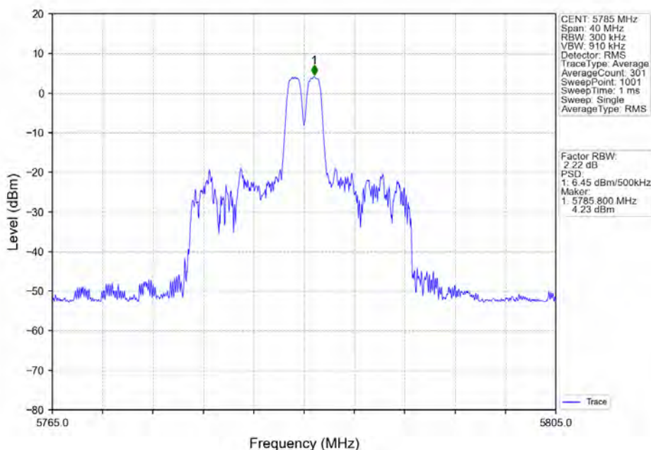
802.11ax(HE20)_MCH_5785MHz_RU26_Mid_Ant1_NTNV
