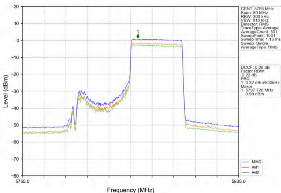
802.11ax(HE40)_HCH_5795MHz_RU242_Right_MIMO_NTNV
