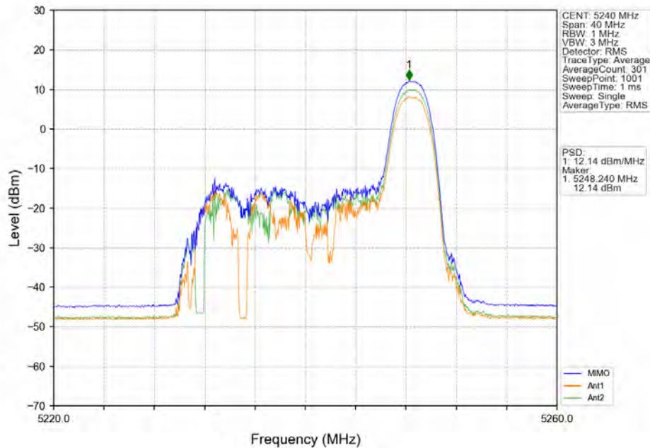
802.11ax(HE20) HCH_5240MHz_RU26_Right_MIMO_NTNV
