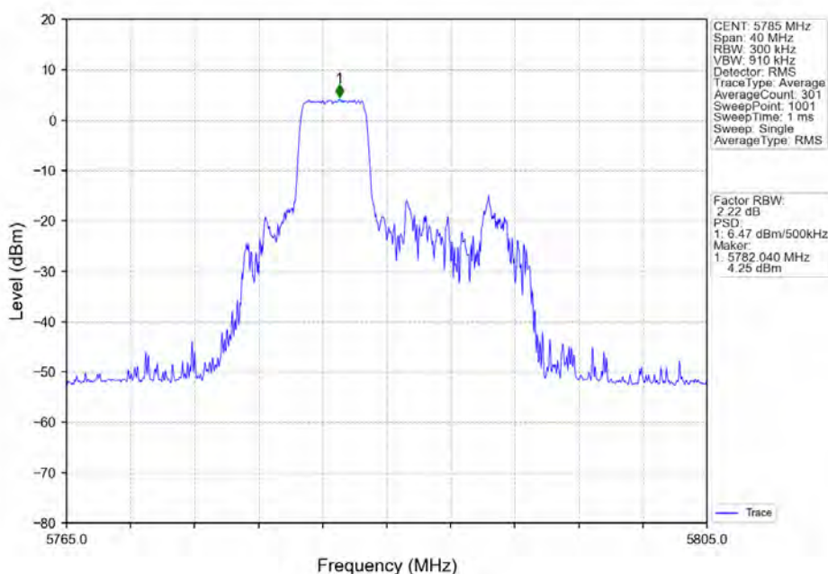
802.11ax(HE20)_MCH_5785MHz_RU52_Mid_Ant1_NTNV
