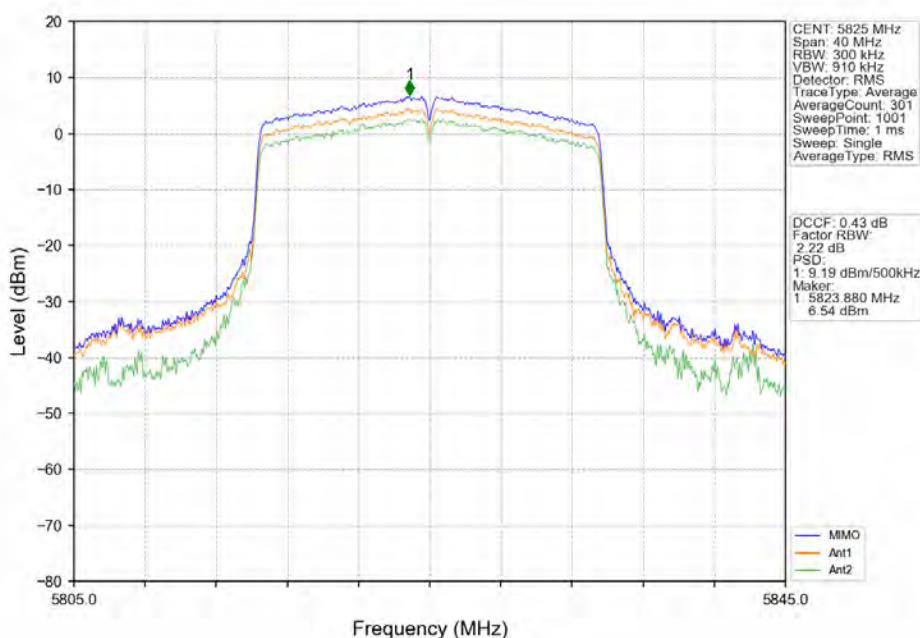
802.11ax(HE20)_HCH_5825MHz_RU242_Left_MIMO_NTNV
