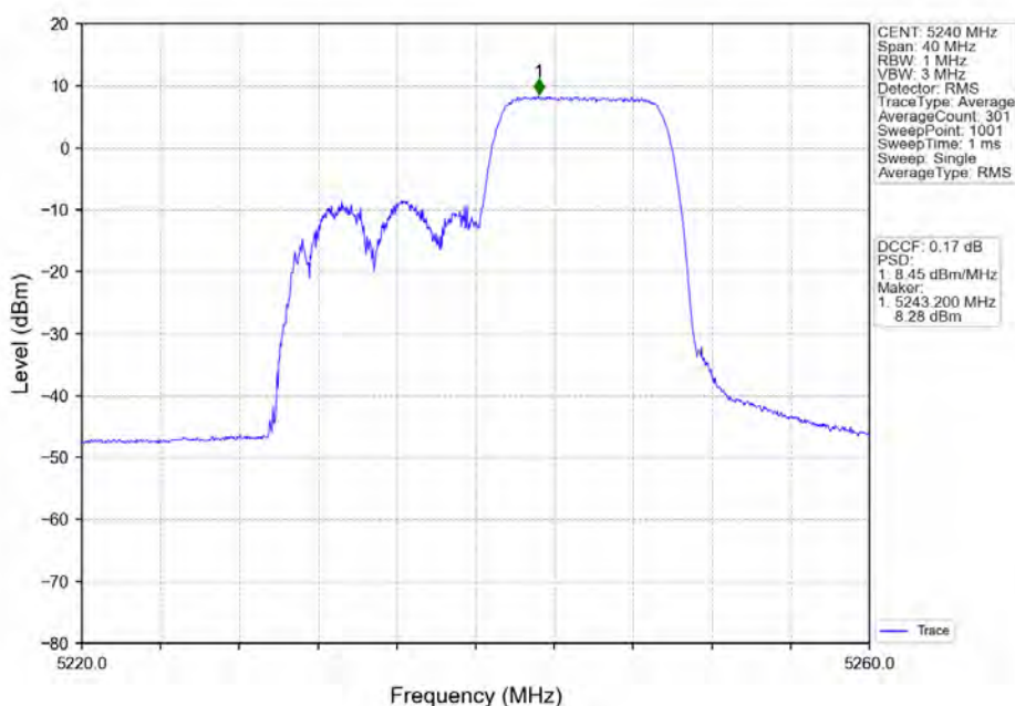
802.11ax(HE20)_HCH_5240MHz_RU106_Right_Ant1_NTNV
