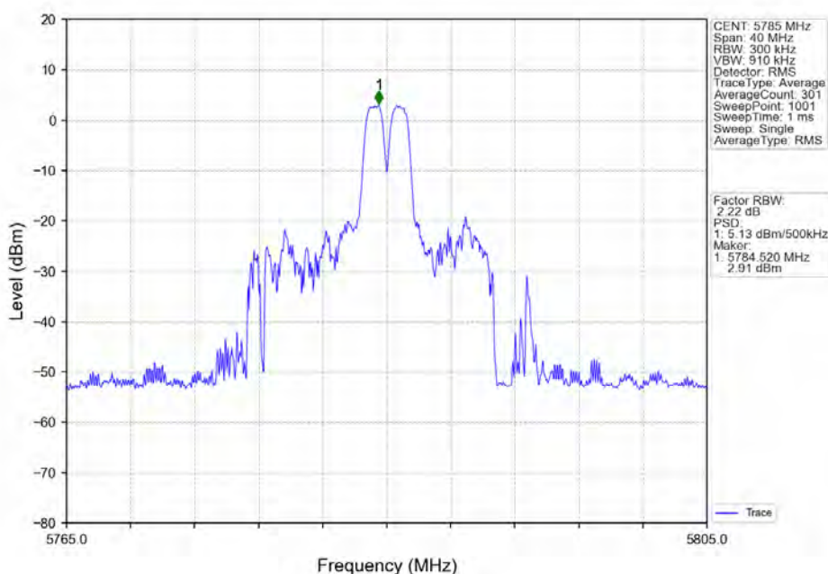
802.11ax(HE20)_MCH_5785MHz_RU26_Mid_Ant2_NTNV
