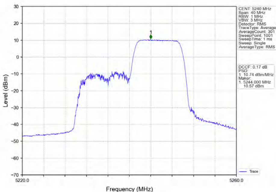
802.11ax(HE20)_HCH_5240MHz_RU106_Right_Ant2_NTNV
