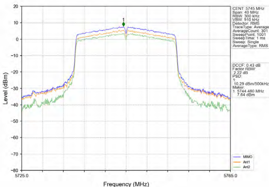
802.11ax(HE20)_LCH_5745MHz_RU242_Left_MIMO_NTNV
