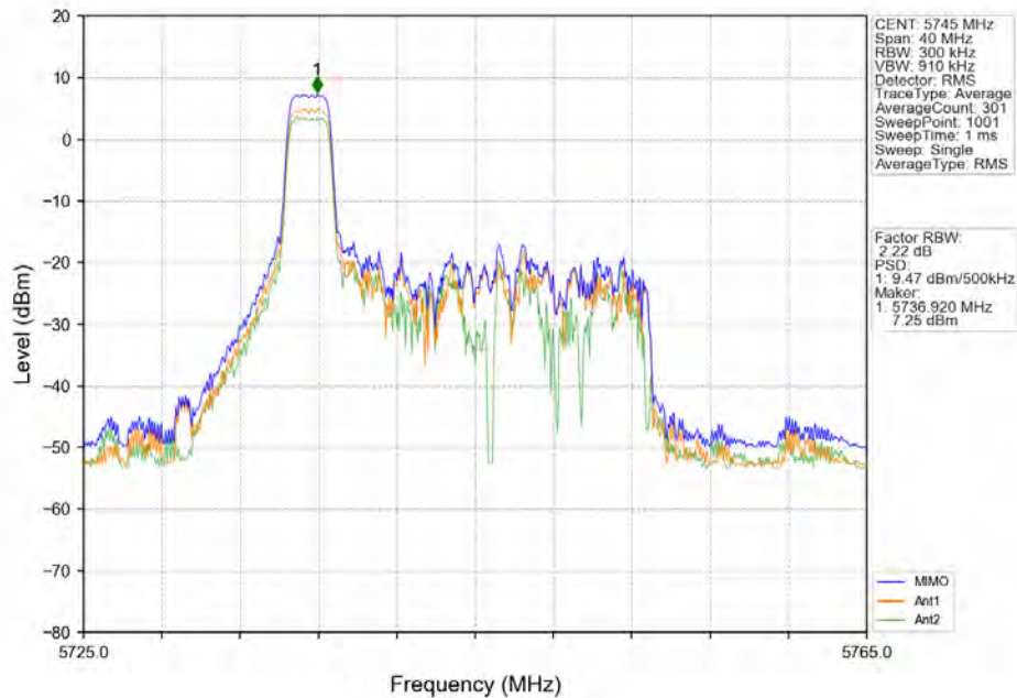
802.11ax(HE20)_LCH_5745MHz_RU26_Left MIMO_NTNV
