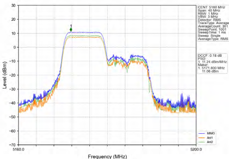
802.11ax(HE20)_LCH_5180MHz_RU106_Left_MIMO_NTNV
