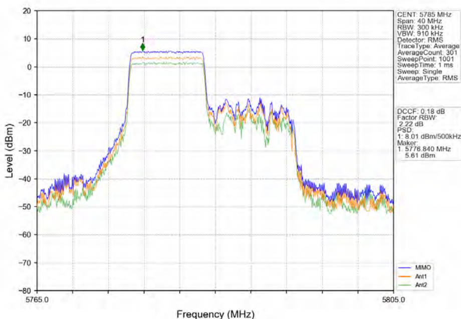
802.11ax(HE20)_MCH_5785MHz_RU106_Left_MIMO_NTNV
