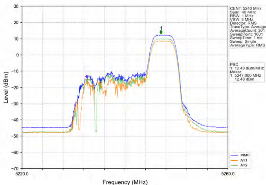
802.11ax(HE20) HCH_5240MHz_RU52_Right_MIMO_NTNV
