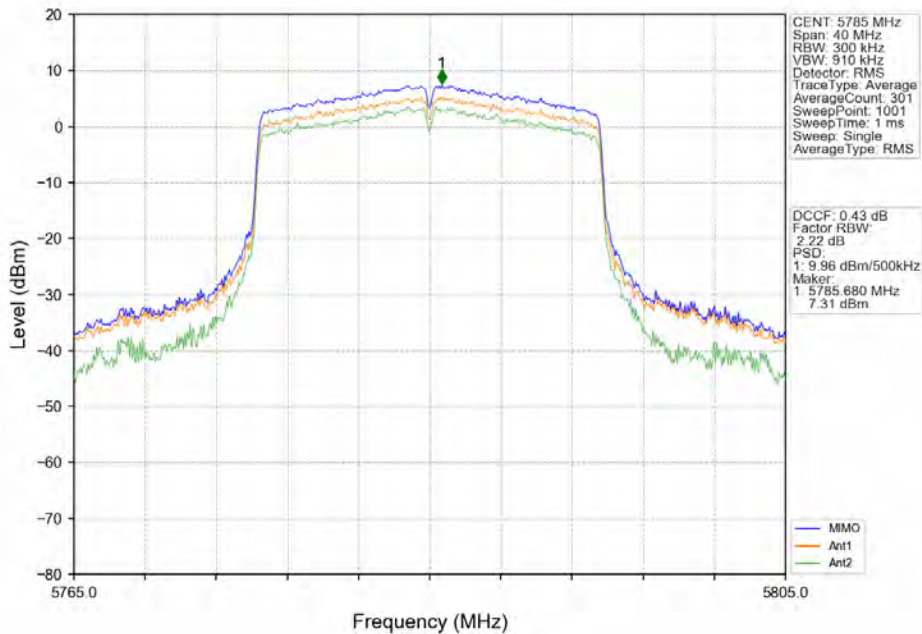
802.11ax(HE20)_MCH_5785MHz_RU242_Left_MIMO_NTNV
