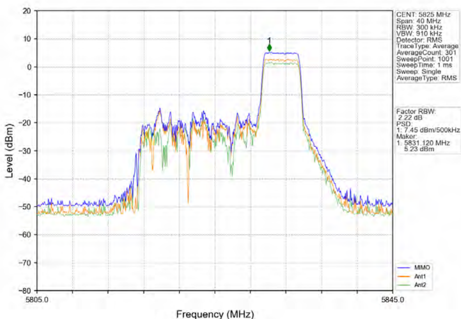
802.11ax(HE20) HCH_5825MHz_RU52_Right_MIMO_NTNV
