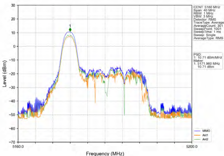
802.11ax(HE20)_LCH_5180MHz_RU26_Left MIMO_NTNV
