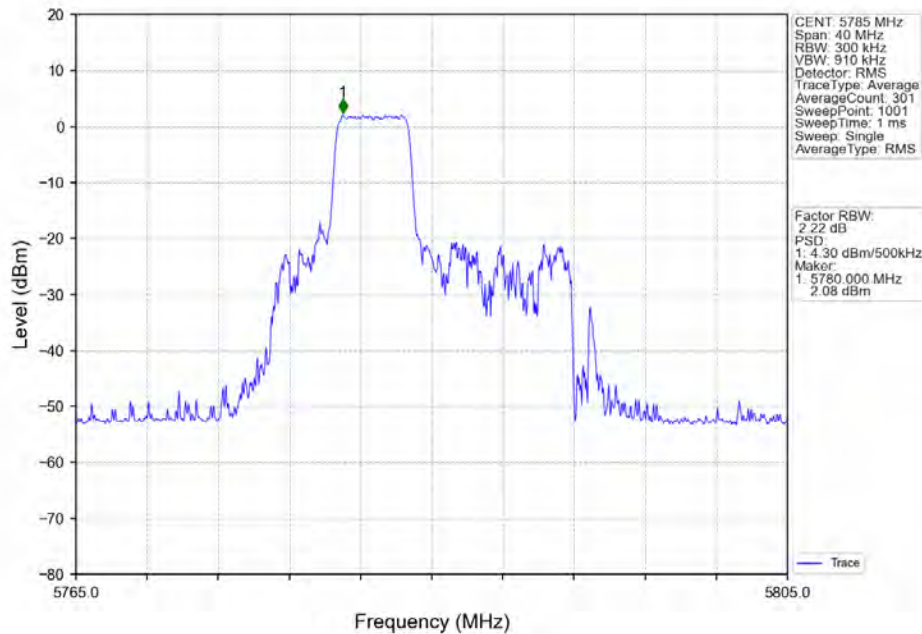
802.11ax(HE20)_MCH_5785MHz_RU52_Mid_Ant2_NTNV
