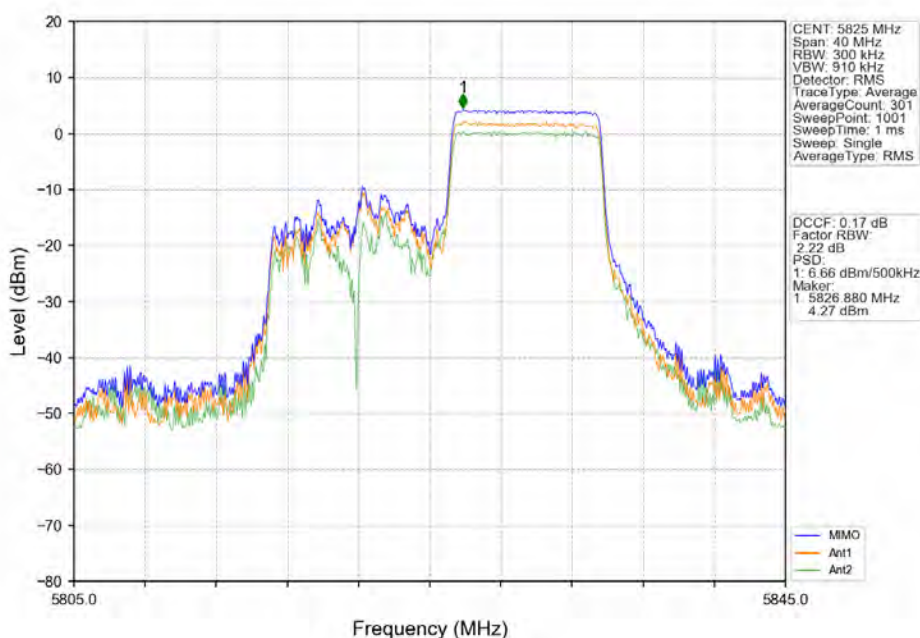
802.11ax(HE20)_HCH_5825MHz_RU106_Right_MIMO_NTNV
