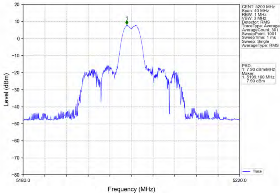
802.11ax(HE20)_MCH_5200MHz_RU26_Mid_Ant2_NTNV
