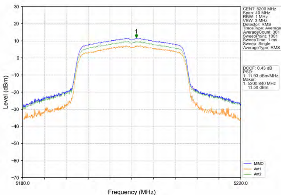
802.11ax(HE20)_MCH_5200MHz_RU242_Left_MIMO_NTNV
