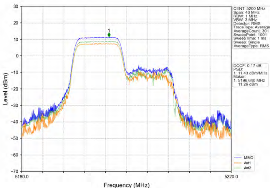
802.11ax(HE20)_MCH_5200MHz_RU106_Left_MIMO_NTNV
