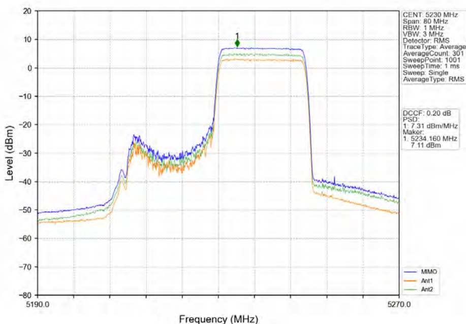
802.11ax(HE40)_HCH_5230MHz_RU242_Right_MIMO_NTNV
