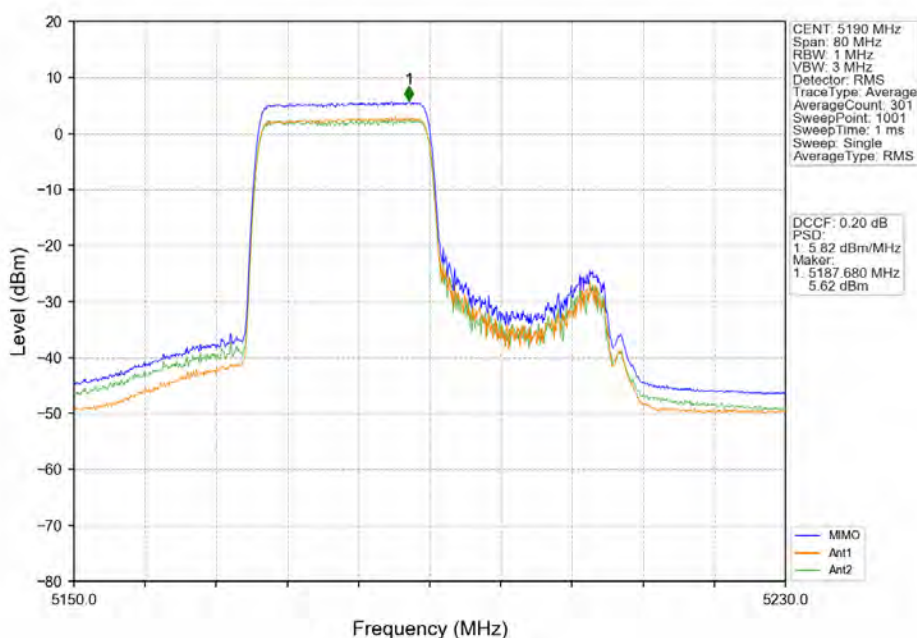
802.11ax(HE40) LCH_5190MHz_RU242_Left_MIMO_NTNV
