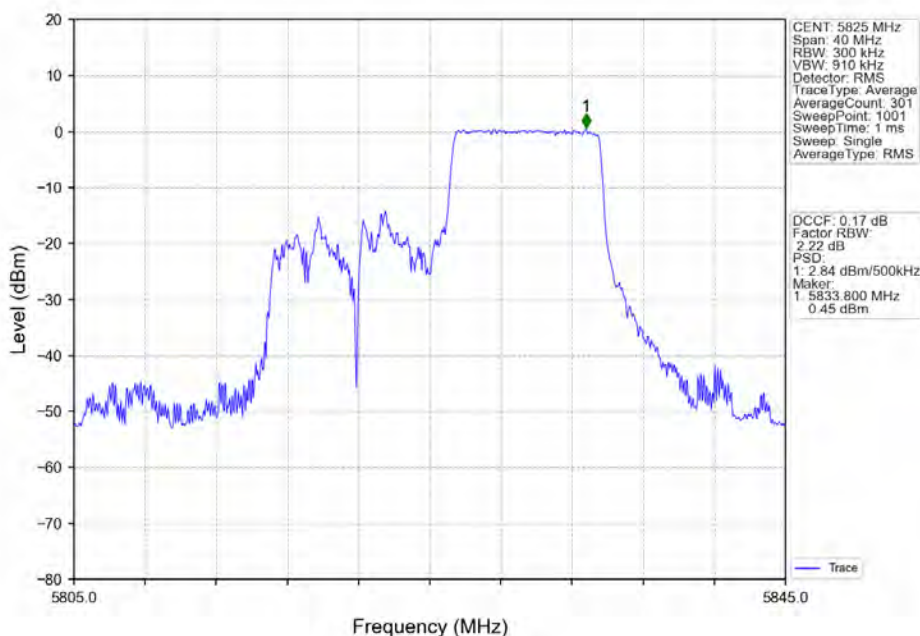
802.11ax(HE20)_HCH_5825MHz_RU106_Right_Ant2_NTNV
