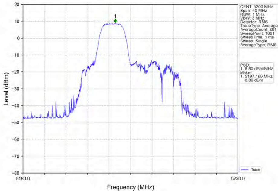
802.11ax(HE20)_MCH_5200MHz_RU52_Mid_Ant2_NTNV
