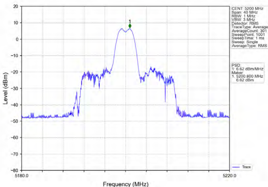
802.11ax(HE20)_MCH_5200MHz_RU26_Mid_Ant1_NTNV
