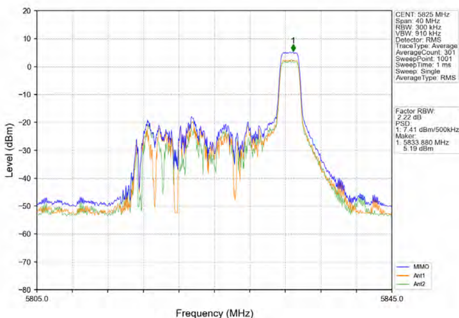
802.11ax(HE20) HCH_5825MHz_RU26_Right_MIMO_NTNV
