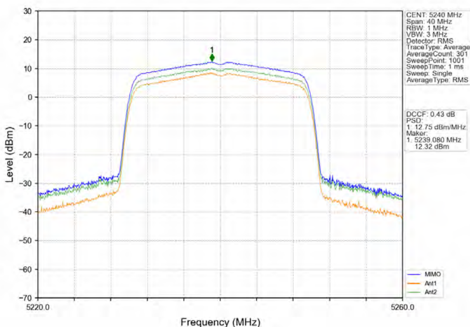
802.11ax(HE20)_HCH_5240MHz_RU242_Left_MIMO_NTNV
