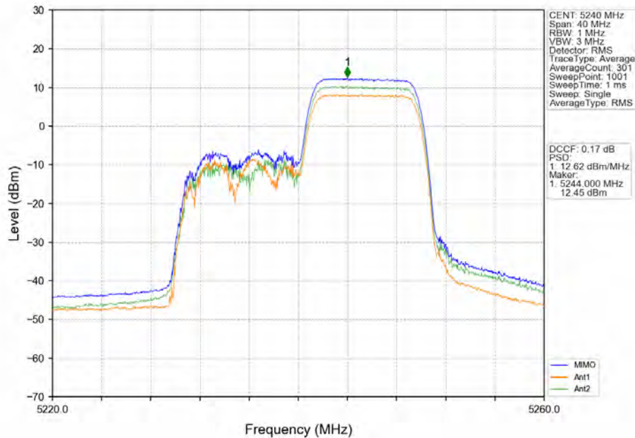
802.11ax(HE20)_HCH_5240MHz_RU106_Right_MIMO_NTNV
