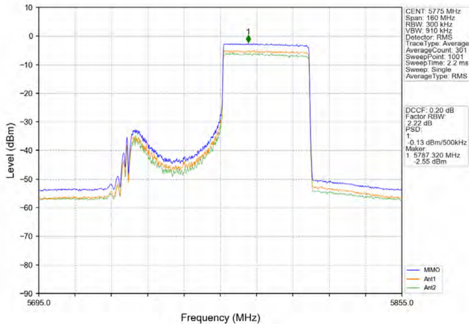
802.11ax(HE80)_MCH_5775MHz_RU484_Right_MIMO_NTNV
