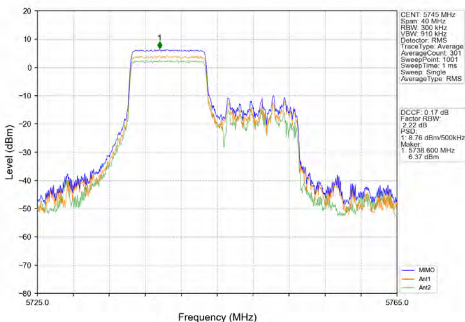
802.11ax(HE20)_LCH_5745MHz_RU106_Left_MIMO_NTNV
