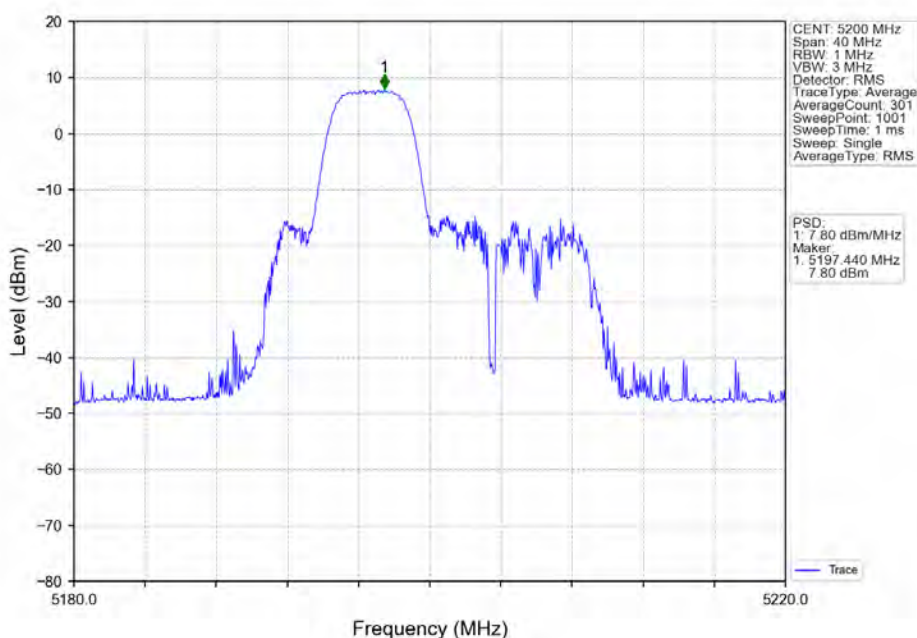
802.11ax(HE20)_MCH_5200MHz_RU52_Mid_Ant1_NTNV
