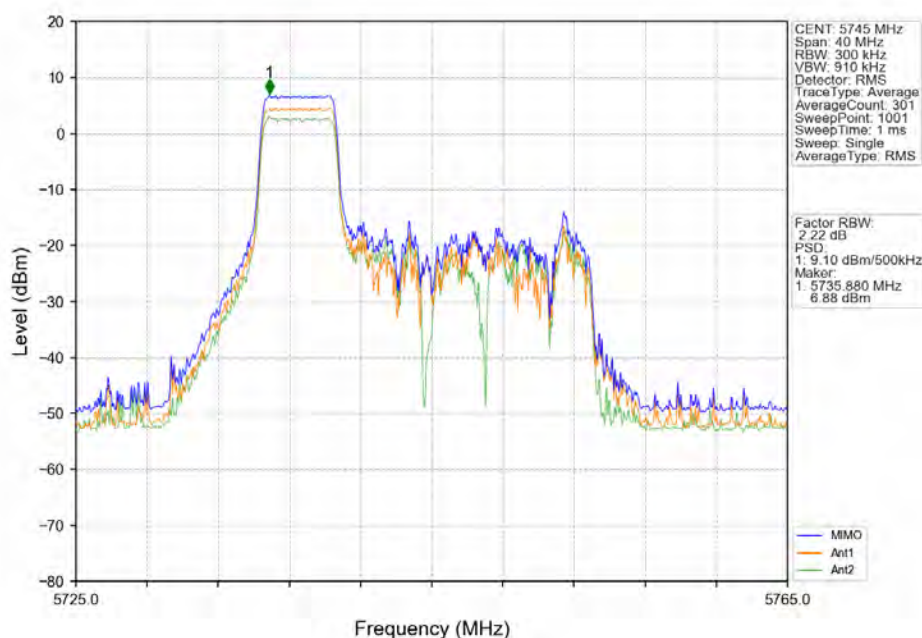
802.11ax(HE20)_LCH_5745MHz_RU52_Left MIMO_NTNV
