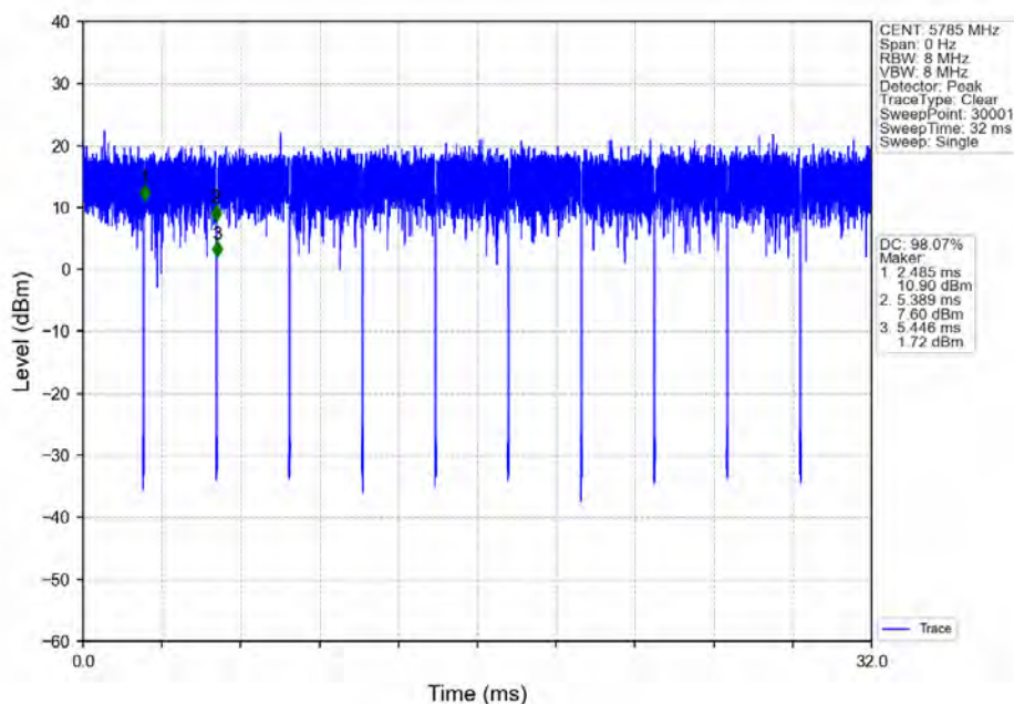
802.11ax(HE20)_MCH_5785MHz_RU26_Mid_Ant2_NTNV
