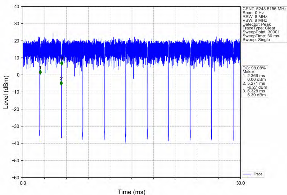
802.11ax(HE20)_HCH_5240MHz_RU26_Right_Ant2_NTNV
