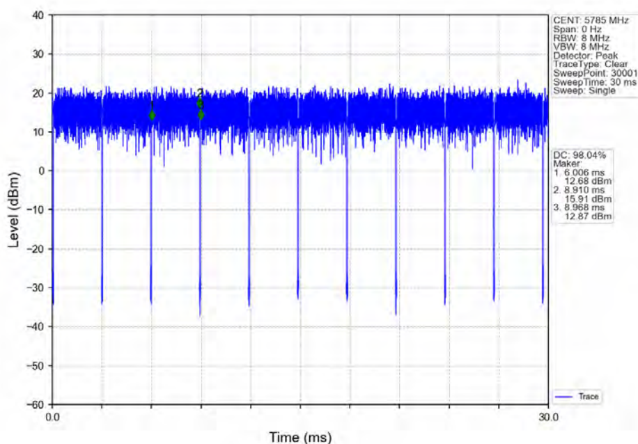
802.11ax(HE20)_MCH_5785MHz_RU26_Mid_Ant1_NTNV
