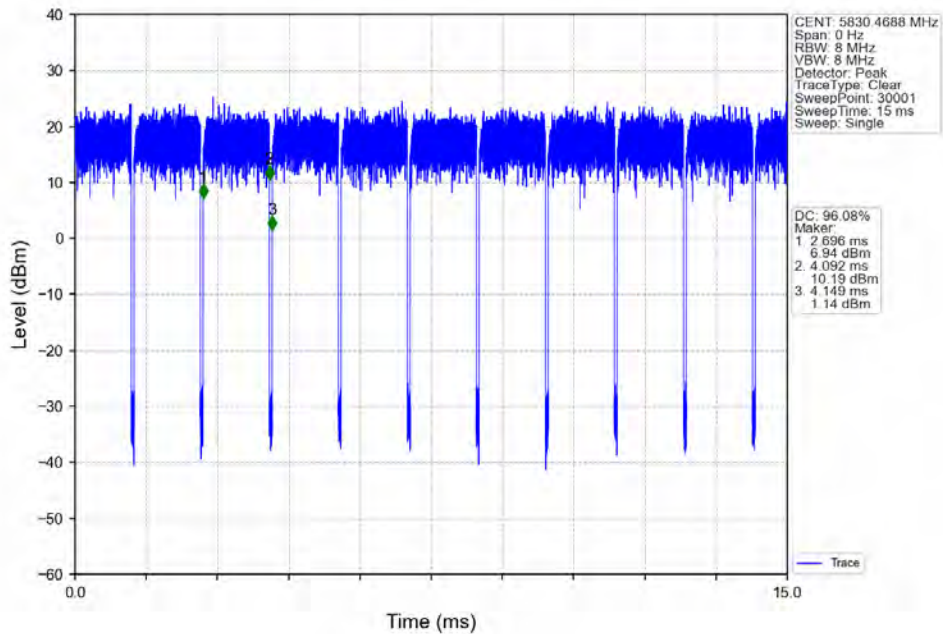
802.11ax(HE20)_HCH_5825MHz_RU106_Right_Ant2_NTNV
