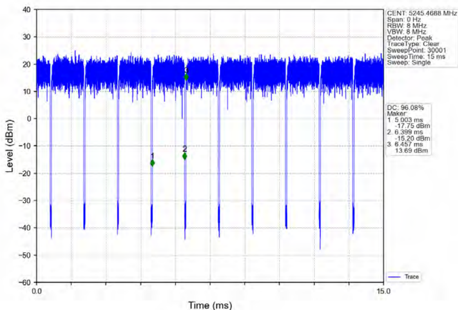
802.11ax(HE20)_HCH_5240MHz_RU106_Right_Ant1_NTNV
