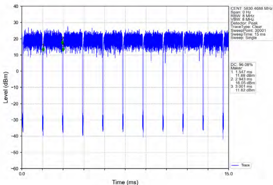
802.11ax(HE20)_HCH_5825MHz_RU106_Right_Ant1_NTNV
