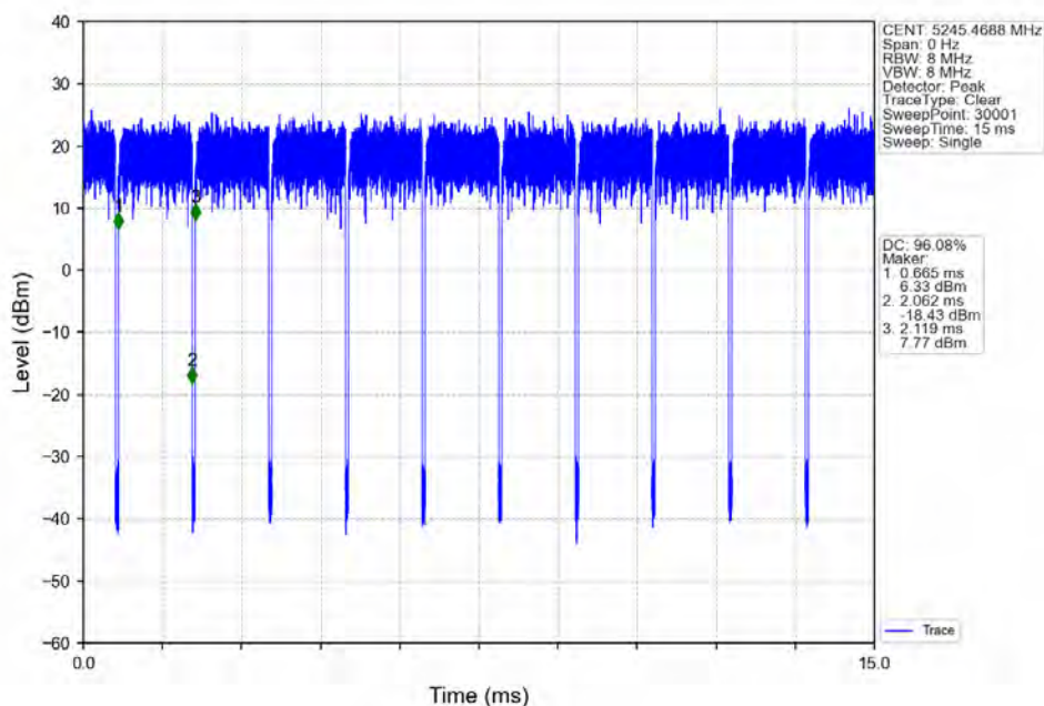
802.11ax(HE20)_HCH_5240MHz_RU106_Right_Ant2_NTNV
