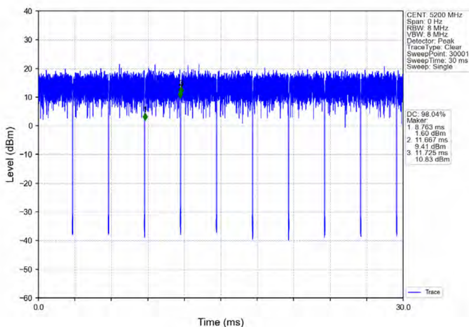
802.11ax(HE20)_MCH_5200MHz_RU26_Mid_Ant2_NTNV
