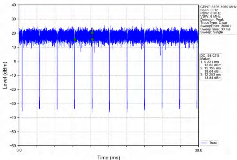
802.11ax(HE20)_MCH_5200MHz_RU52_Mid_Ant2_NTNV
