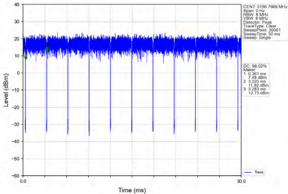
802.11ax(HE20)_MCH_5200MHz_RU52_Mid_Ant1_NTNV
