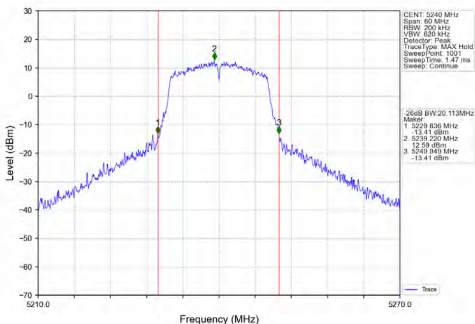
802.11a_HCH_5240MHz_Ant1_NTNV
