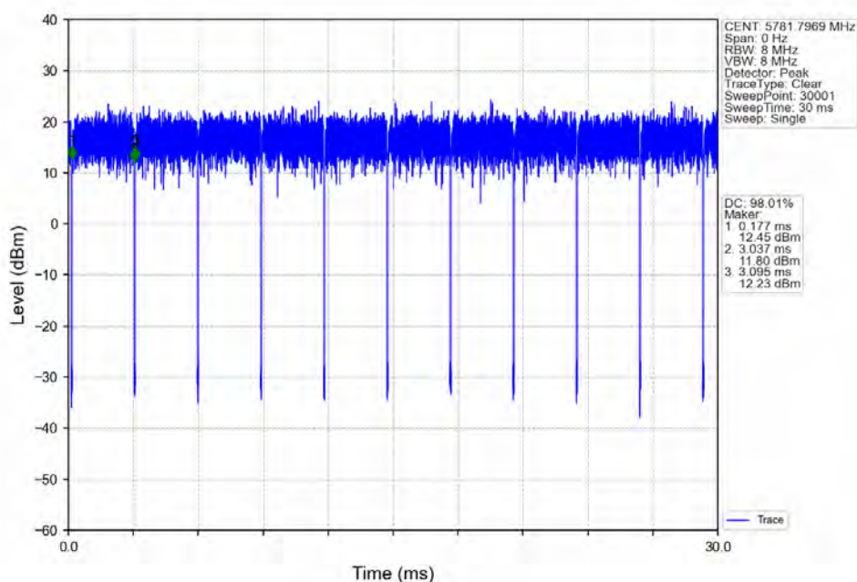
802.11ax(HE20)_MCH_5785MHz_RU52_Mid_Ant2_NTNV
