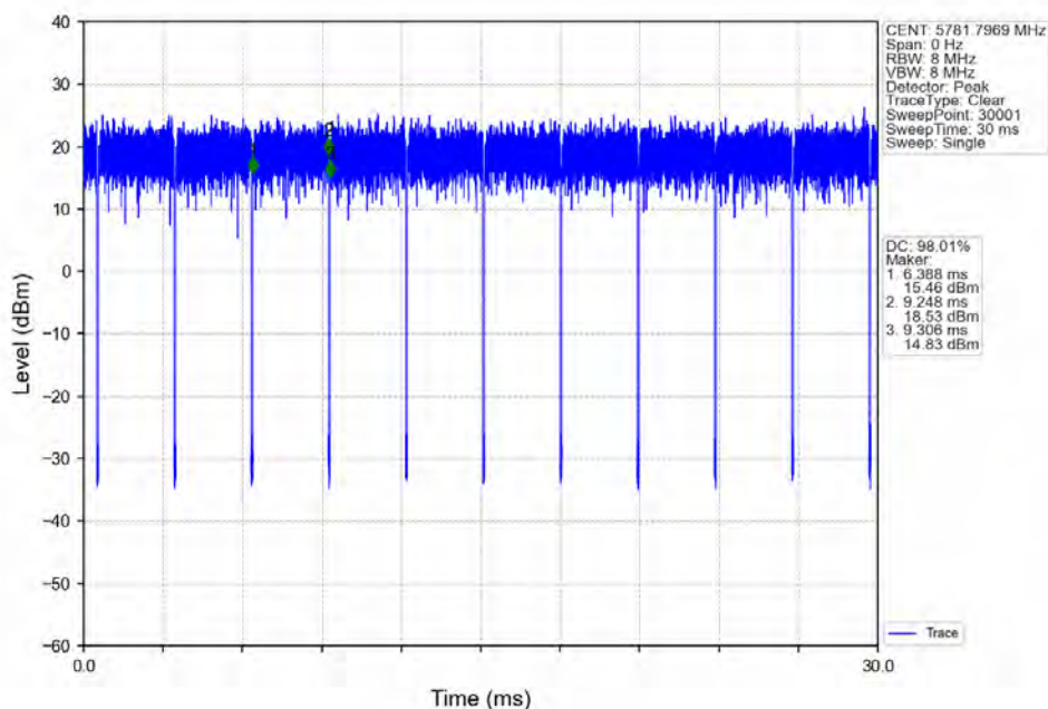
802.11ax(HE20)_MCH_5785MHz_RU52_Mid_Ant1_NTNV
