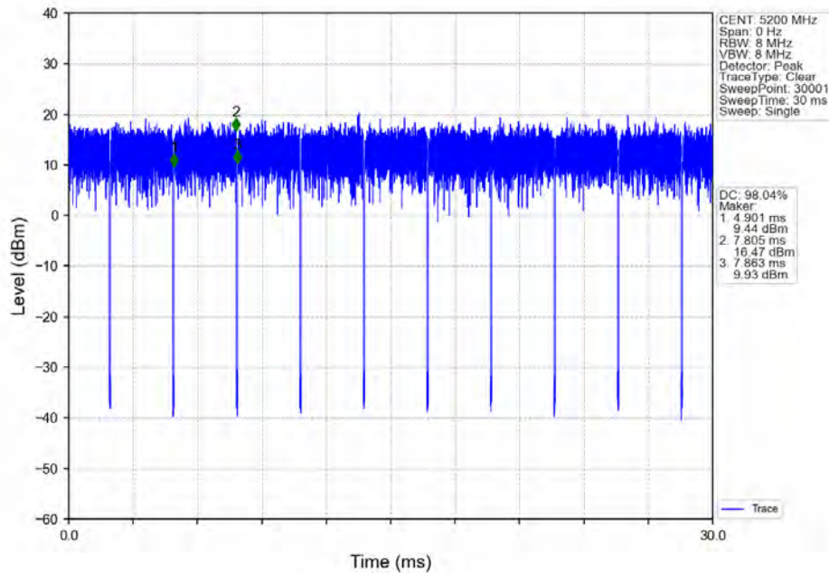
802.11ax(HE20)_MCH_5200MHz_RU26_Mid_Ant1_NTNV
