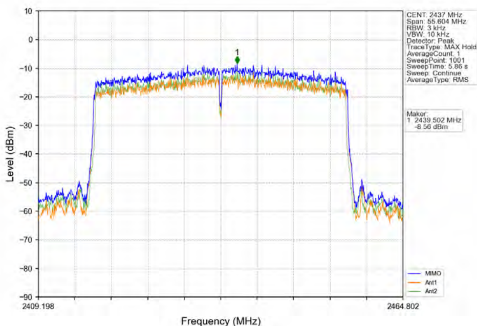
802.11ax(HE40)_MCH_2437MHz_RU484_Left_MIMO_NTNV
