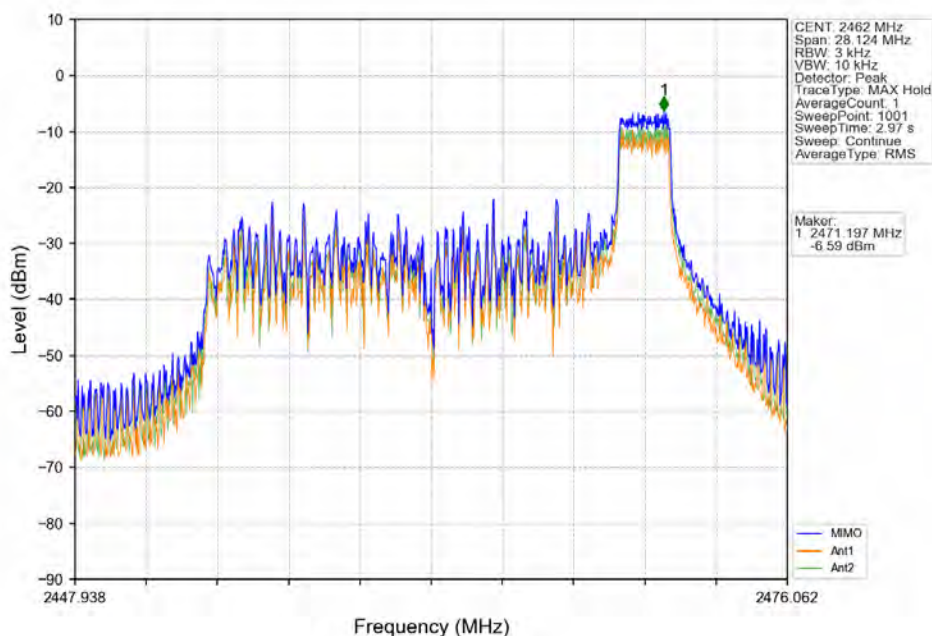
802.11ax(HE20)_HCH_2462MHz_RU26_Right_MIMO_NTNV
