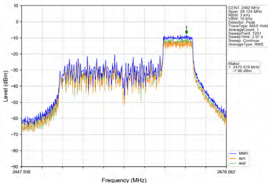
802.11ax(HE20)_HCH_2462MHz_RU52_Right_MIMO_NTNV
