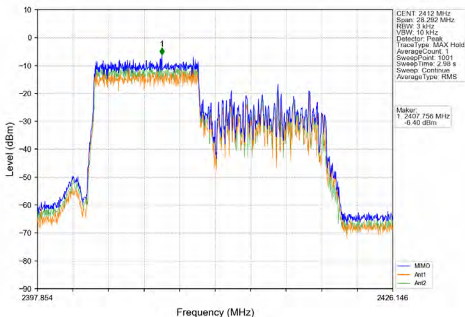
802.11ax(HE20)_LCH_2412MHz_RU106_Left_MIMO_NTNV
