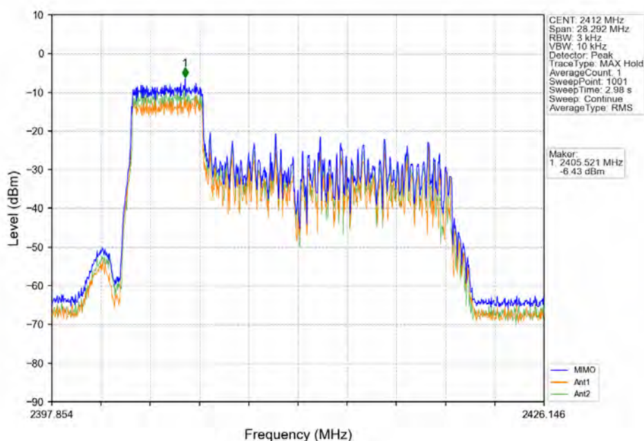
802.11ax(HE20)_LCH_2412MHz_RU52_Left MIMO_NTNV
