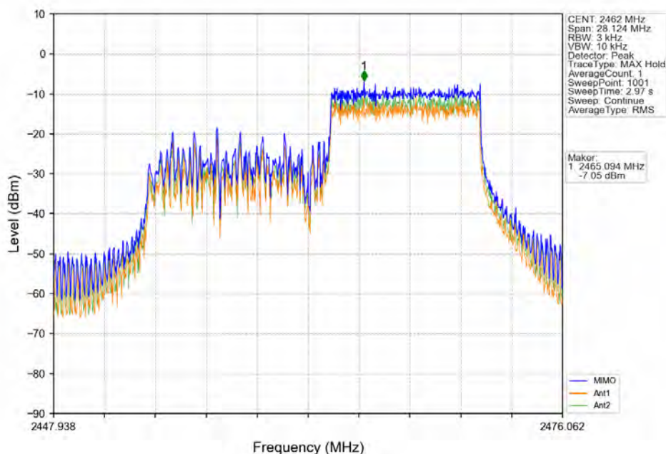
802.11ax(HE20)_HCH_2462MHz_RU106_Right_MIMO_NTNV
