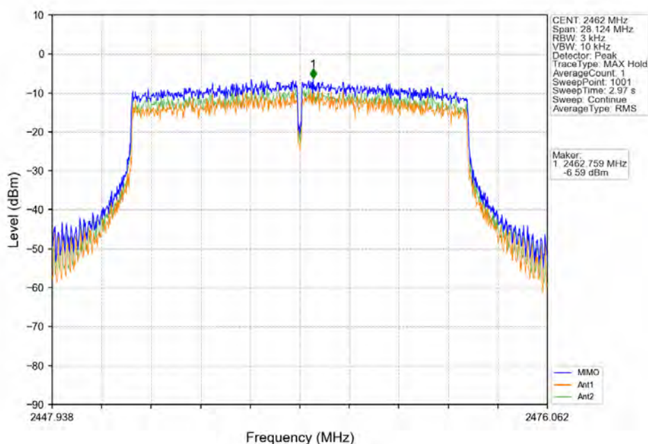
802.11ax(HE20)_HCH_2462MHz_RU242_Left_MIMO_NTNV
