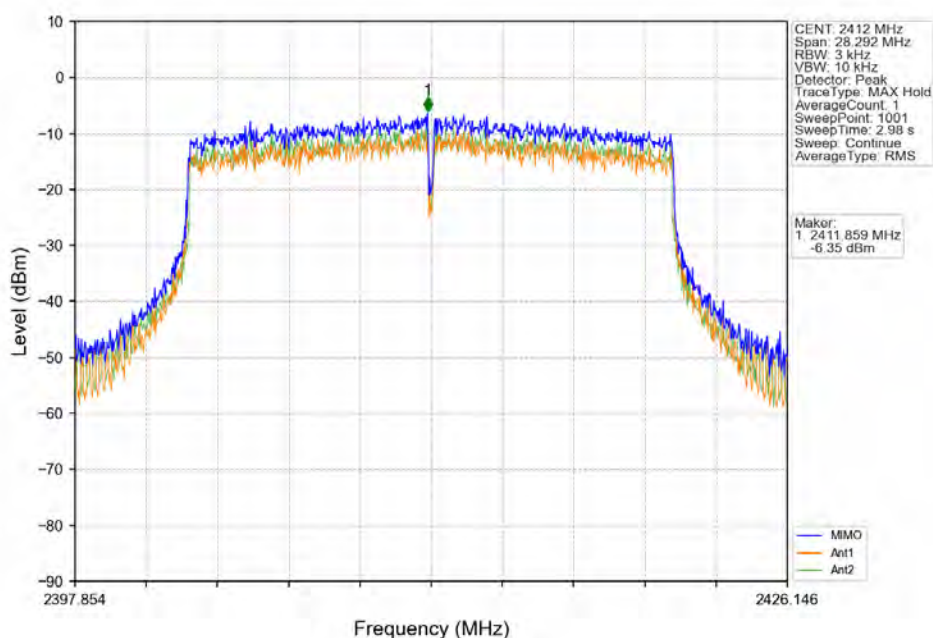
802.11ax(HE20)_LCH_2412MHz_RU242_Left_MIMO_NTNV
