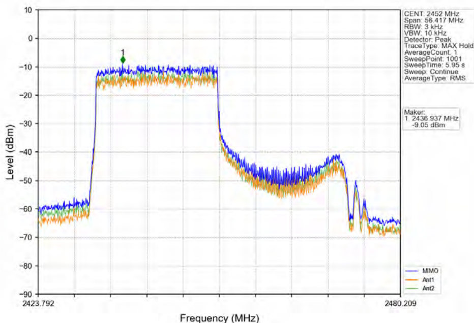
802.11ax(HE40)_HCH_2452MHz_RU242_Right_MIMO_NTNV
