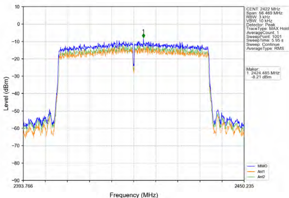
802.11ax(HE40) LCH_2422MHz_RU484_Left_MIMO_NTNV
