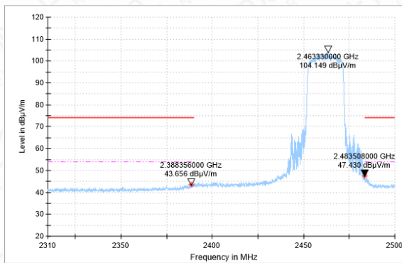
BANDEGE-11AX(40M)-CH3-AV
