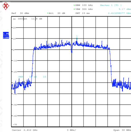
11AX20MIMO-Ant1-2412-0~Reference-PASS
