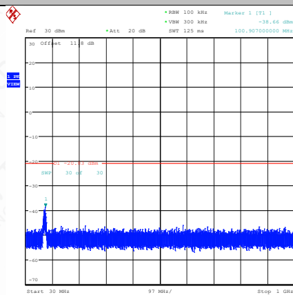
11AX20MIMO-Ant1-2412-30~1000-PASS
