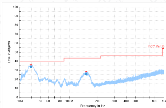
RSE-11N-CH11-30MHz-1GHz
