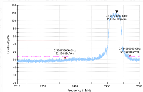
BANDEGE-11N-CH11-PK
