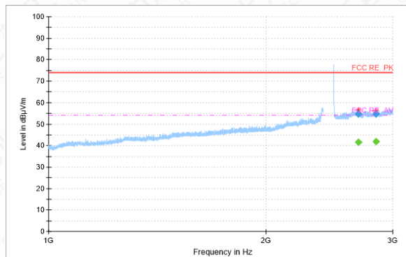
RSE-11N-CH11-1GHz-3GHz
