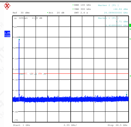
11AX40MIMO-Ant2-2422-1000~26500-PASS
