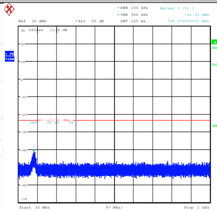
11AX40MIMO-Ant1-2422-30~1000-PASS
