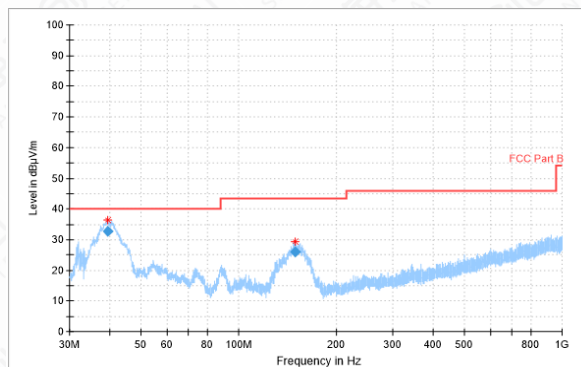
RSE-11N-CH6-30MHz-1GHz
