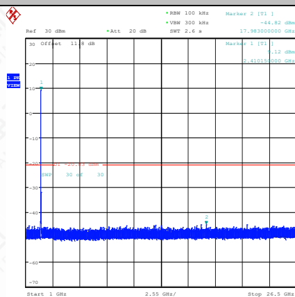
11AX20MIMO-Ant1-2412-1000~26500-PASS
