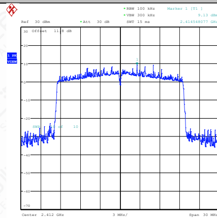
11AX20MIMO-Ant2-2412-0~Reference-PASS
