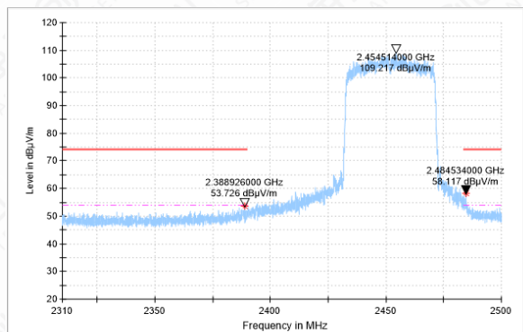
BADEGE-11AX(40M)-CH9-PK
