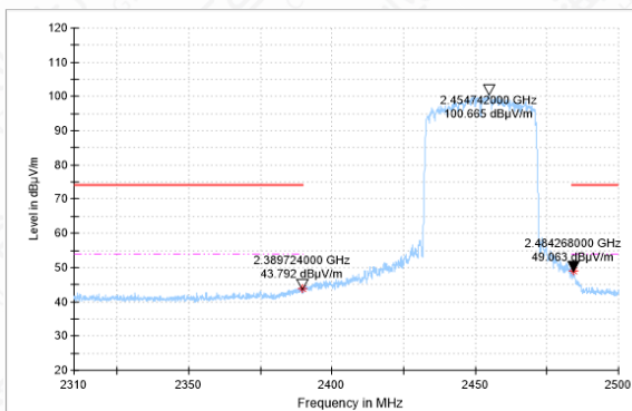
BADEGE-11AX(40M)-CH9-AV
