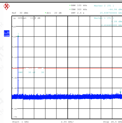
11AX20MIMO-Ant2-2412-1000~26500-PASS
