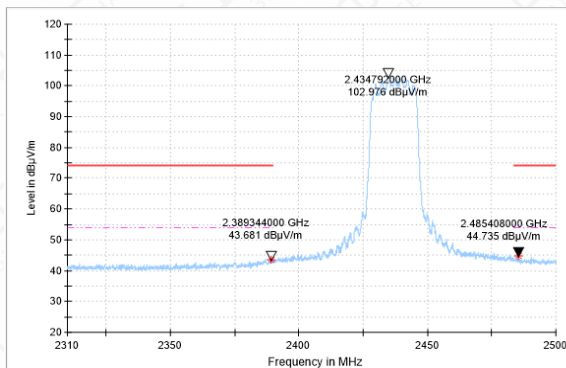
BANDEDGE-11N-CH6-AV
