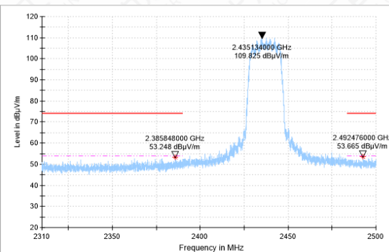
BANDEDGE-11N-CH6-PK
