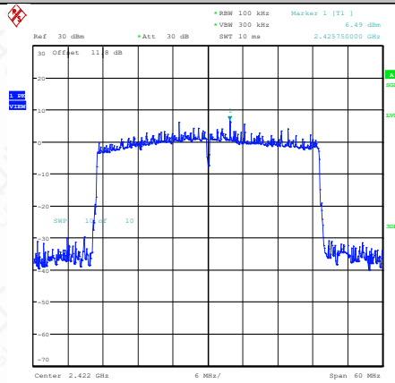
11AX40MIMO-Ant1-2422-0~Reference-PASS
