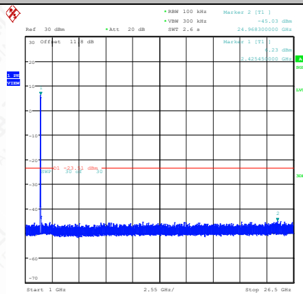
11AX40MIMO-Ant1-2422-1000~26500-PASS
