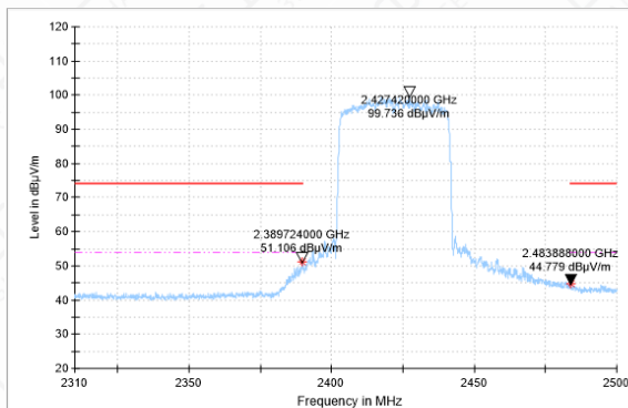
BANDEGE-11AX(40M)-CH3-AV
