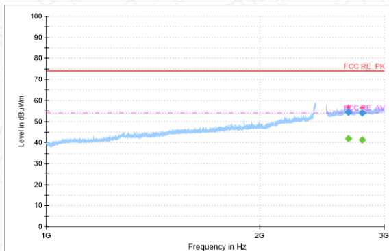
RSE-11N-CH6-1GHz-3GHz
