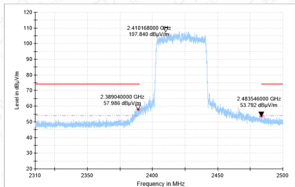
BANDEGE-11AX(40M)-CH3-PK
