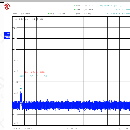
11AX20MIMO-Ant2-2412-30~1000-PASS
