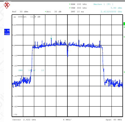
11AX40MIMO-Ant2-2422-0~Reference-PASS
