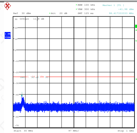
11AX40MIMO-Ant2-2422-30~1000-PASS
