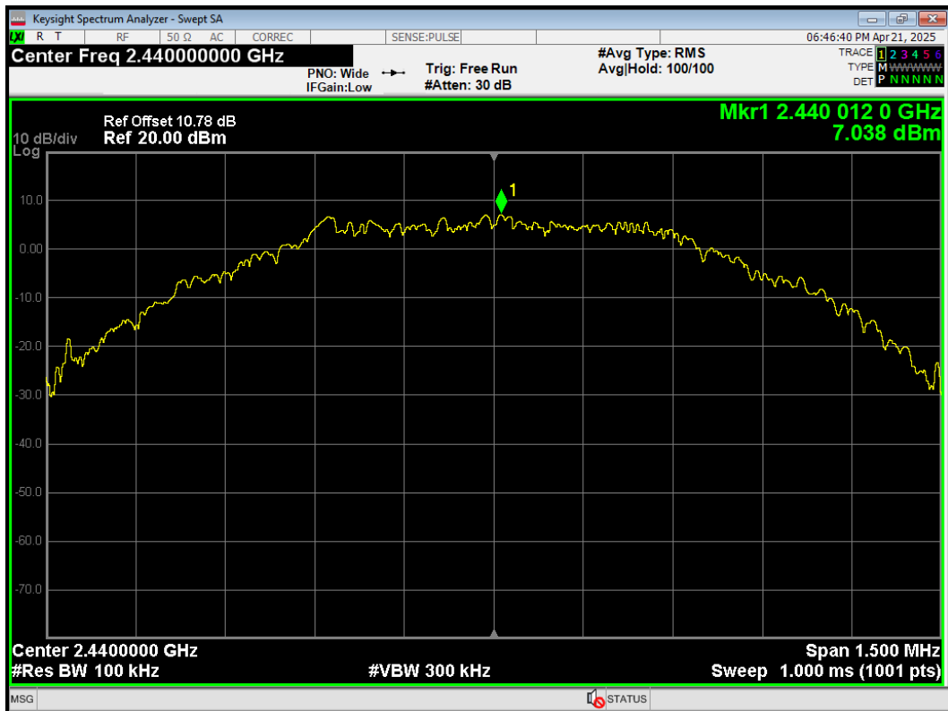
Tx. Spurious S=2 2440MHz Emission
