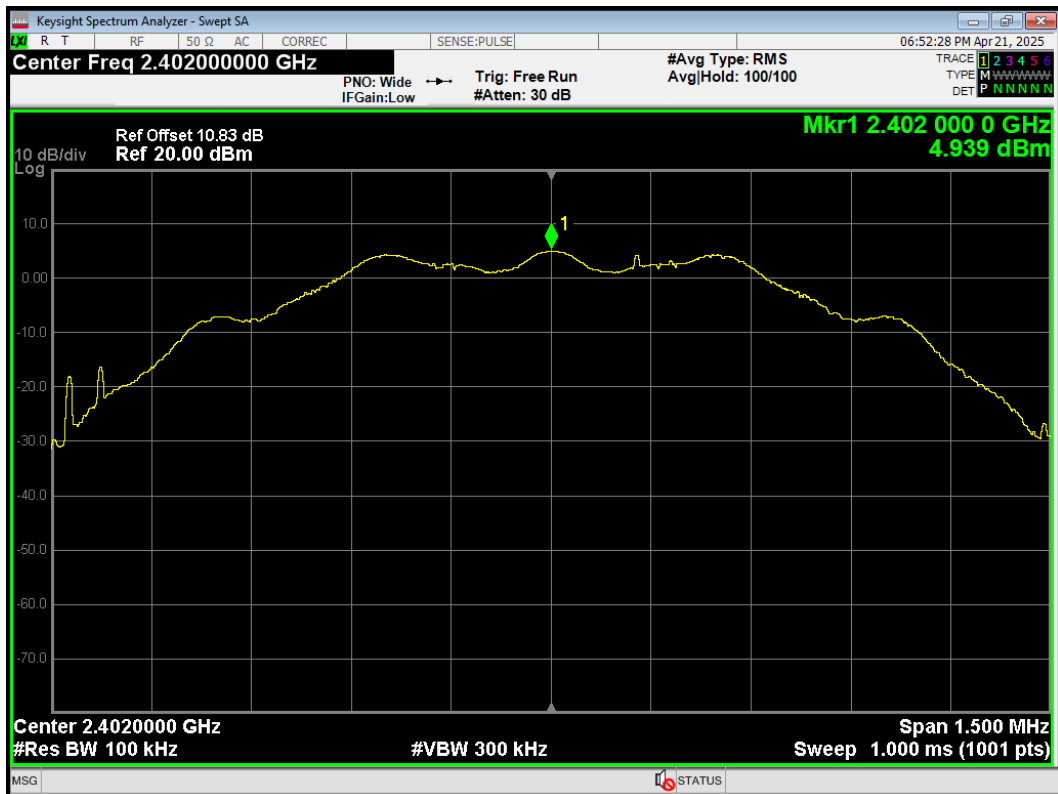
Tx. Spurious S=8 2402MHz Emission
