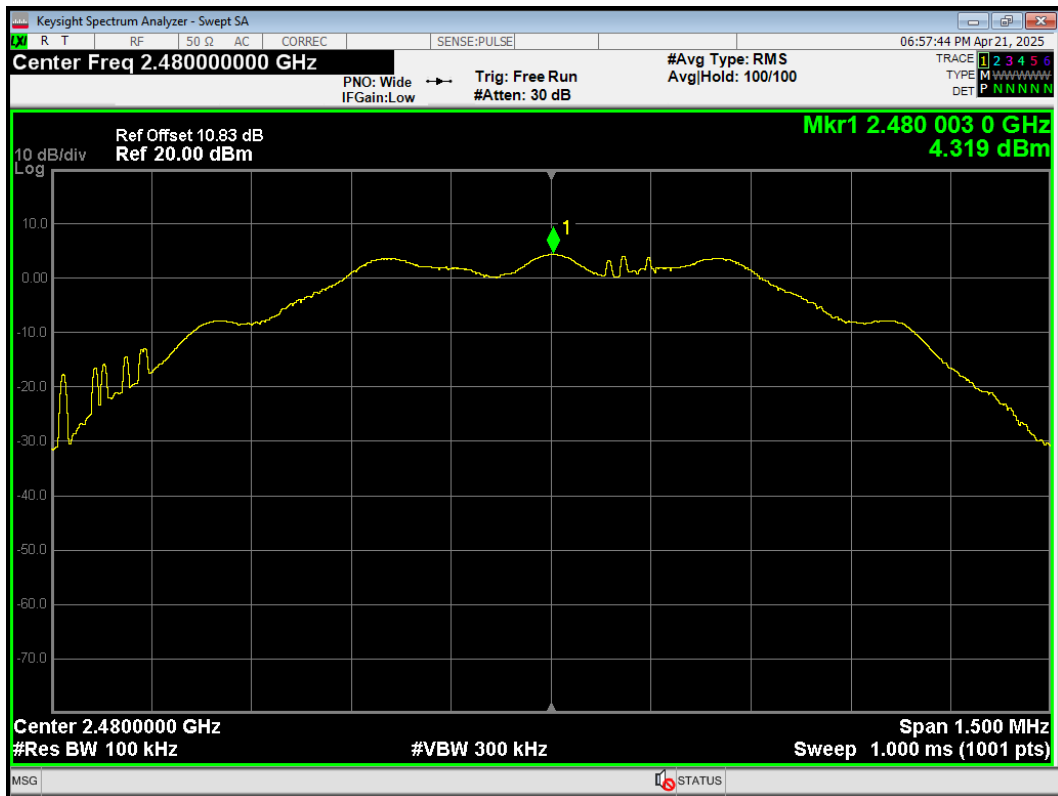
Tx. Spurious S=8 2480MHz Emission
