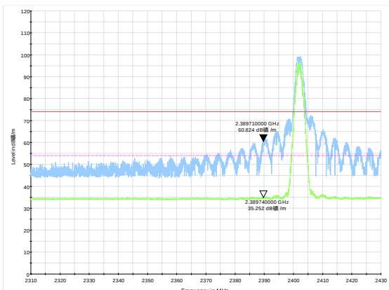
Bluetooth LE (1M) Channel 0 Peak+ Average
