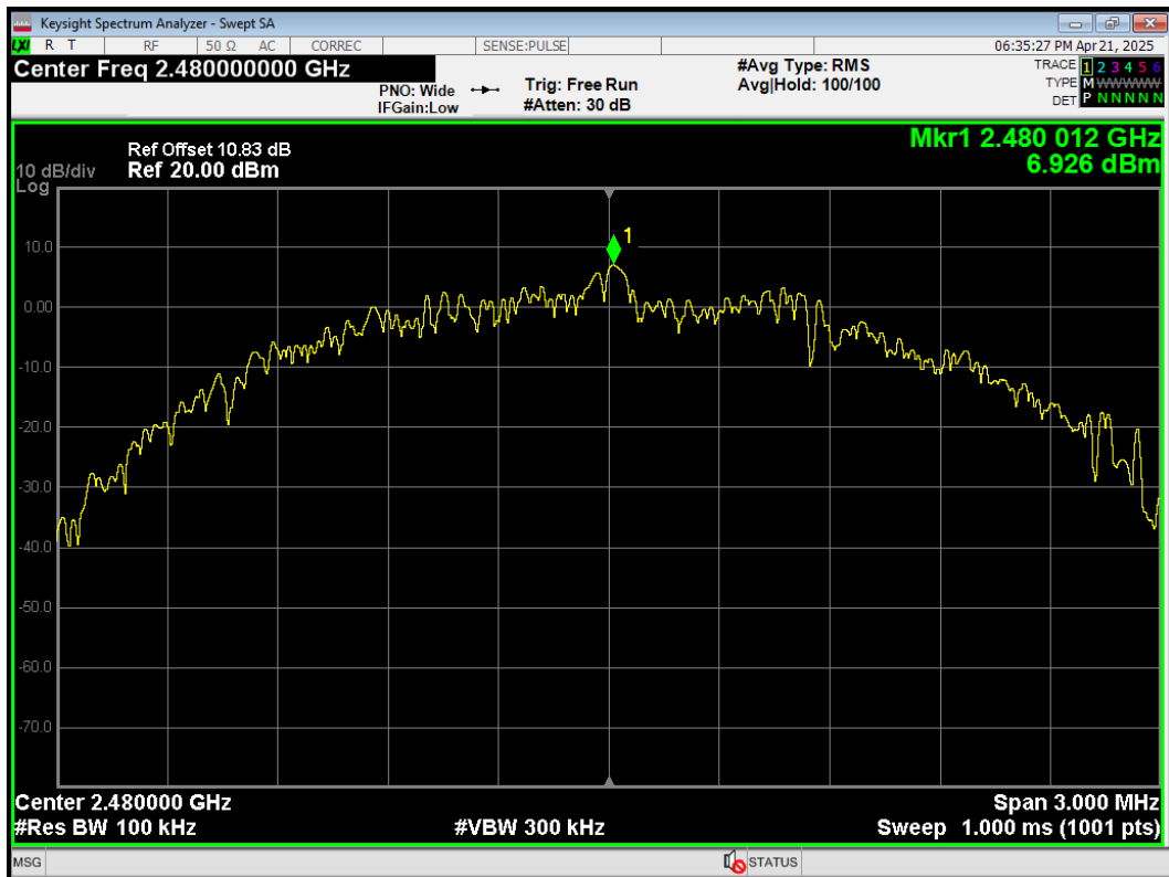
Tx. Spurious BLE (2M) 2480MHz Emission
