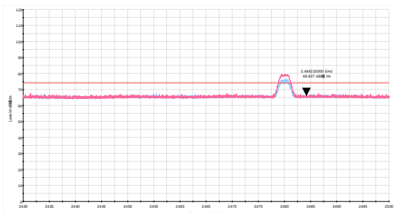
Bluetooth LE (2M) Channel 39 Peak
