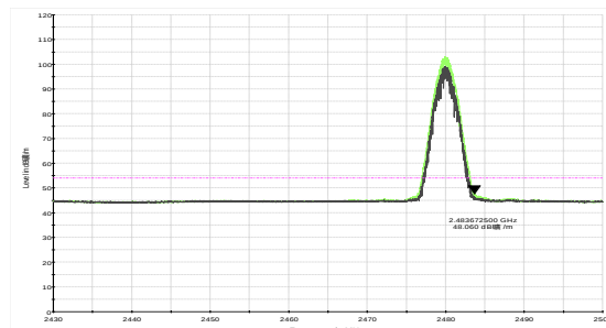
Bluetooth LE (2M) Channel 39 Average
