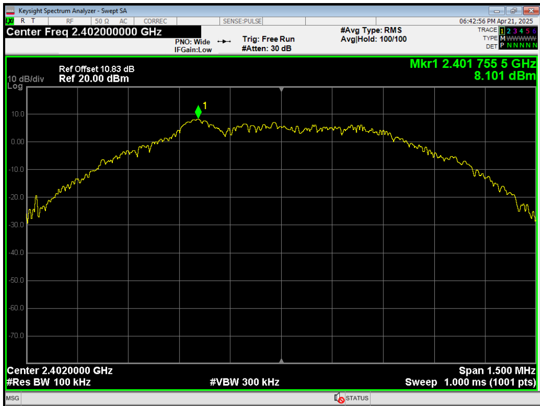
Tx. Spurious S=2 2402MHz Emission
