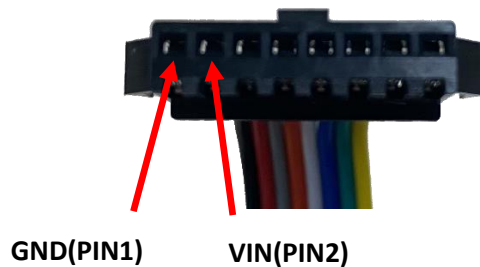
(Picture 4: Power Connection)
