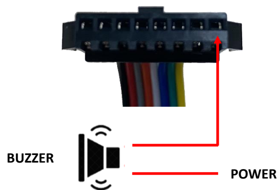
(Picture 6: Typical Connection with Buzzer as Digital Output)
