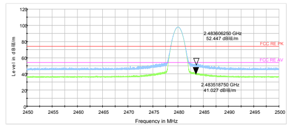
Bluetooth LE Channel 39 Peak & Average
