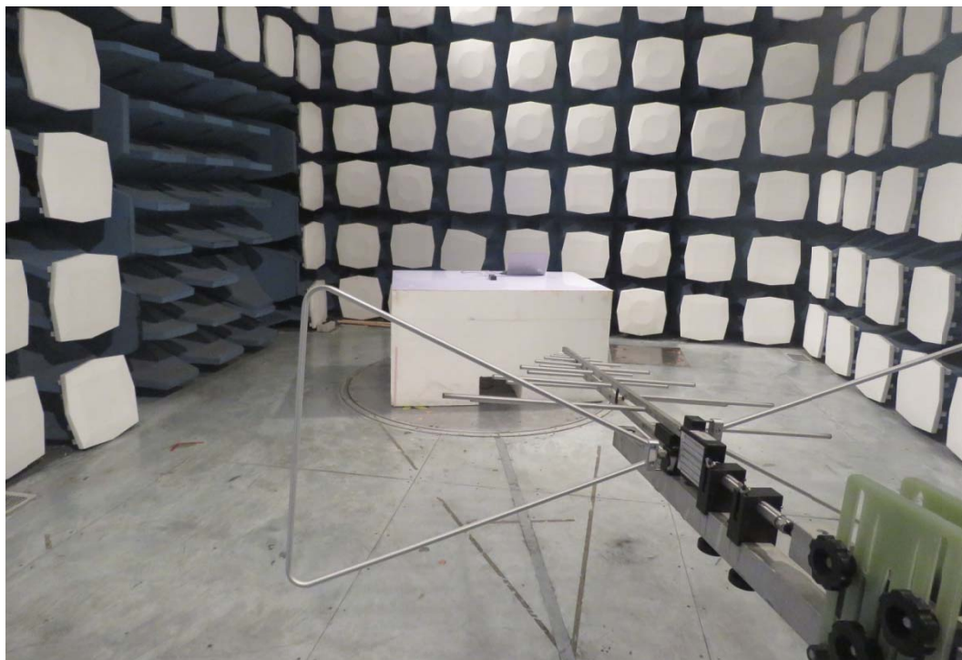
30MHz-1GHz
