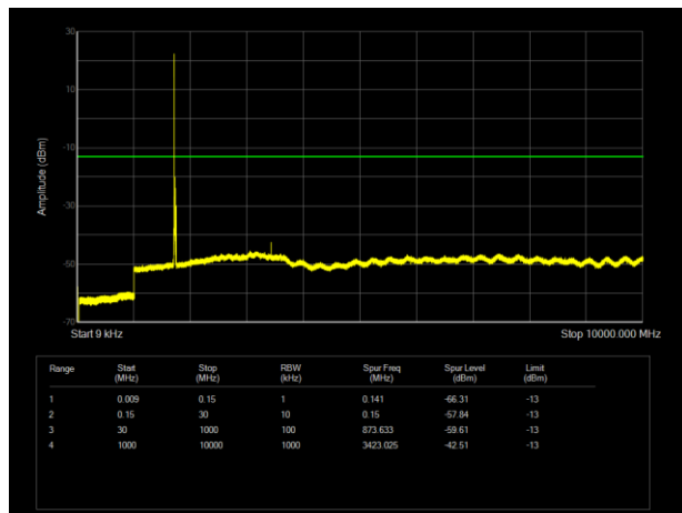
LTE Band 66 20MHz CH-Middle 9kHz ~10GHz
