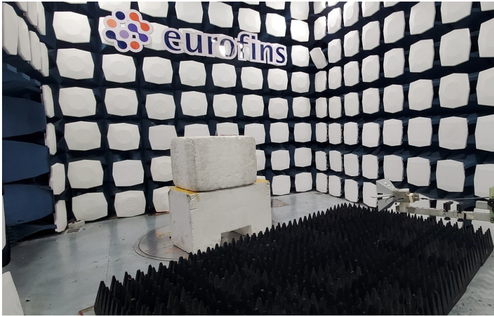
Picture 1: Radiated Spurious Emissions Test setup
