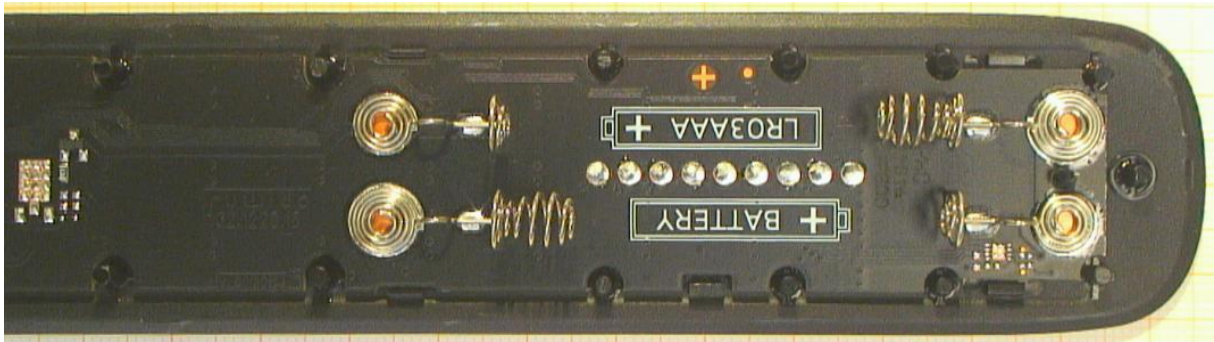
fig. 10 – PCB detail 2
