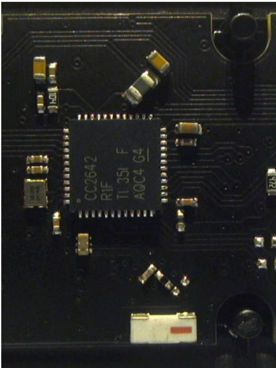
fig. 11 – PCB detail 3 (antenna position)
