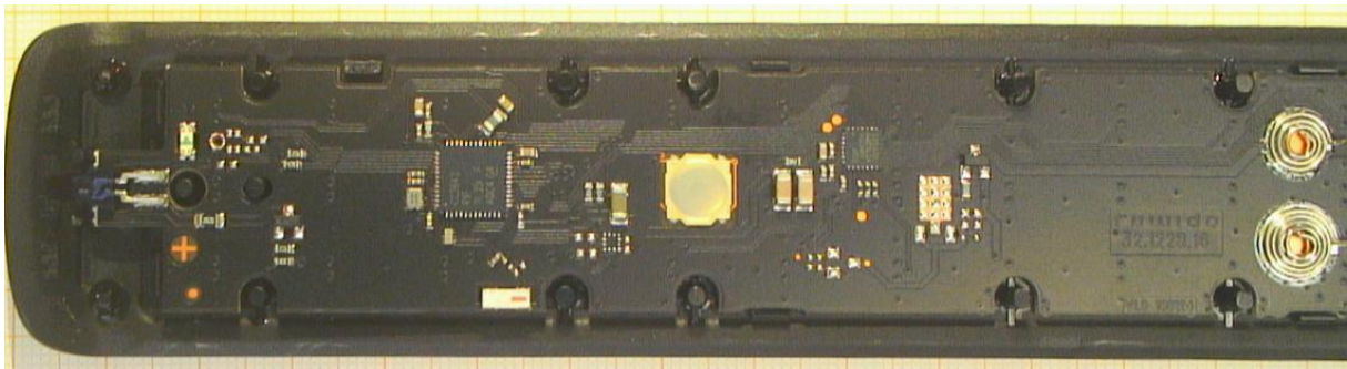
fig. 9 – PCB detail 1
