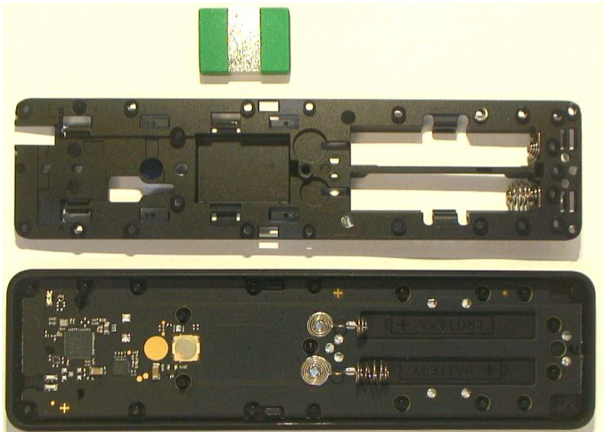
pic. 8 – wheight removed
