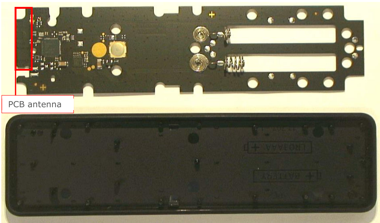
pic. 9 – PCB removed
