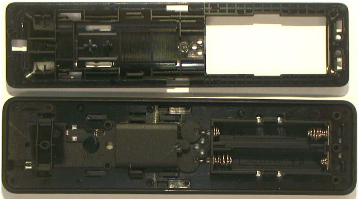
pic. 6 – bottom part removed
