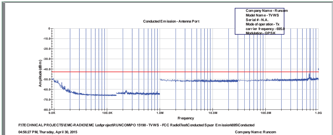
Figure 247 Conducted Emission 695.0 MHz – Port 2
