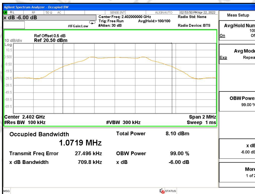
6dB Bandwidth Mode1 CH37
