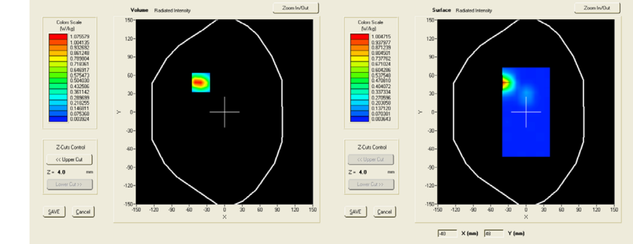
SAR, Z Axis Scan (X = -40, Y = 48)
