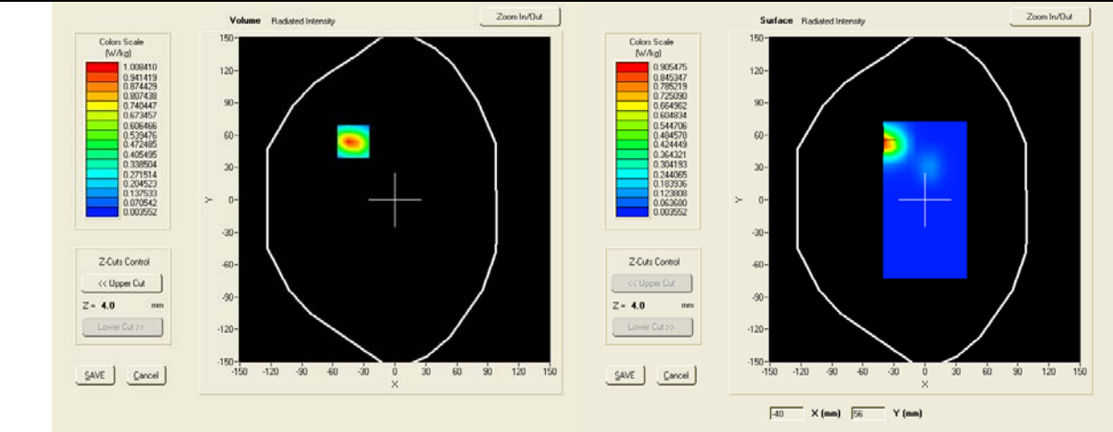
SAR, Z Axis Scan (X = -40, Y = 54)
