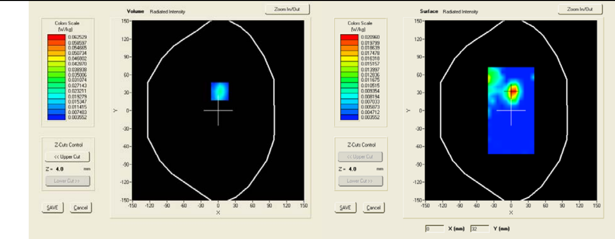
SAR, Z Axis Scan (X = 3, Y = 32)
