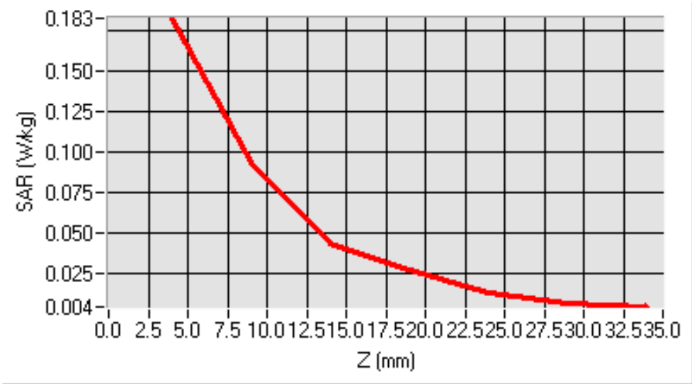
SAR, Z Axis Scan (X = 9, Y = 72)
