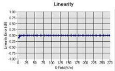
Linearity:±1-2.25% (±1-0.10dB)
