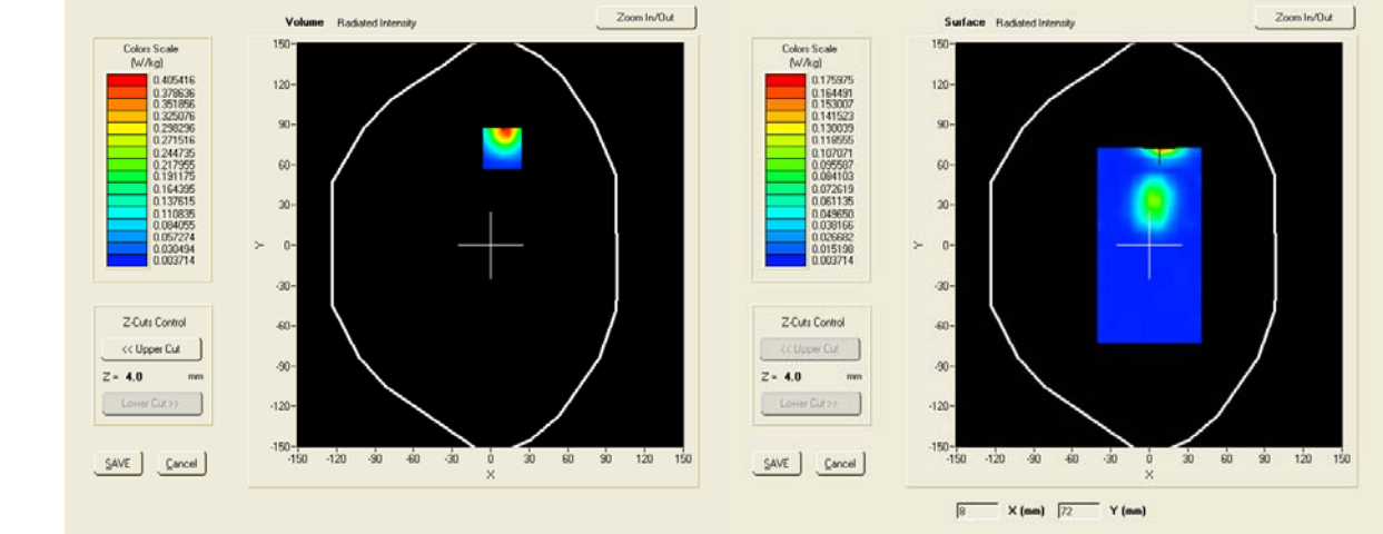
SAR, Z Axis Scan (X = 9, Y = 72)
