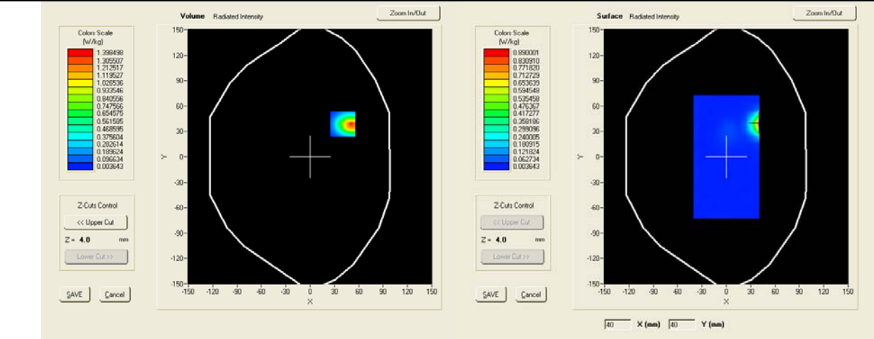
SAR, Z Axis Scan (X = 40, Y = 39)
