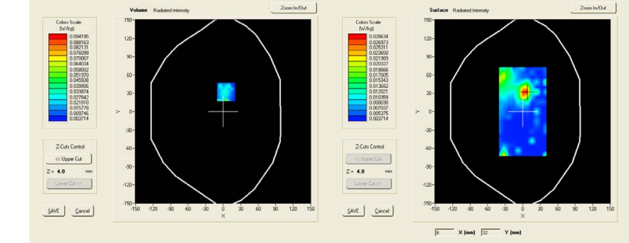
SAR, Z Axis Scan (X = 5, Y = 32)
