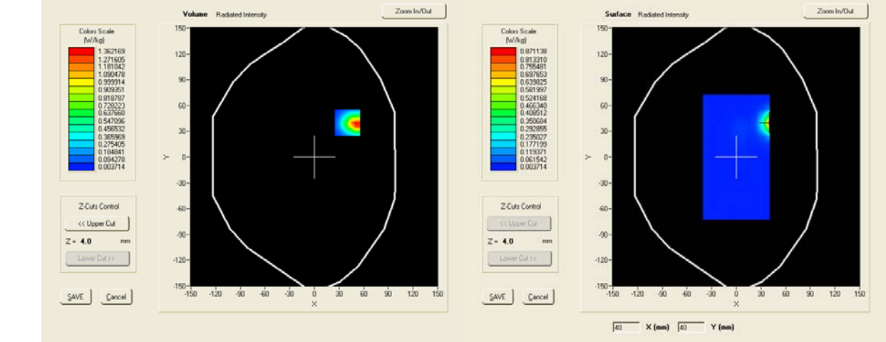
SAR, Z Axis Scan (X = 40, Y = 40)
