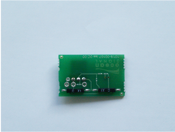
Figure 4: S100 SART PCB – Switch Board.
