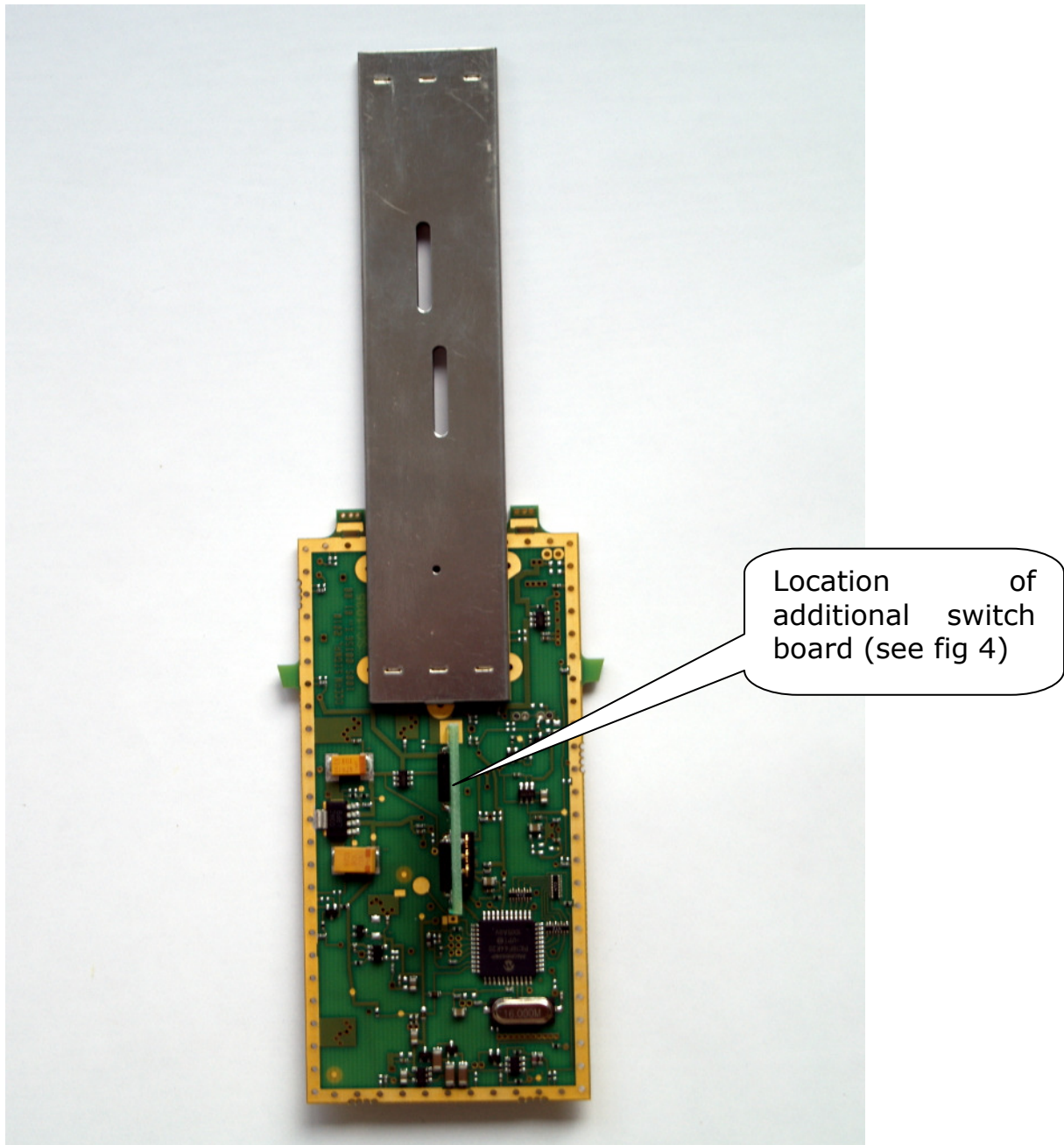
Figure 1: S100 SART PCB – Front Side
