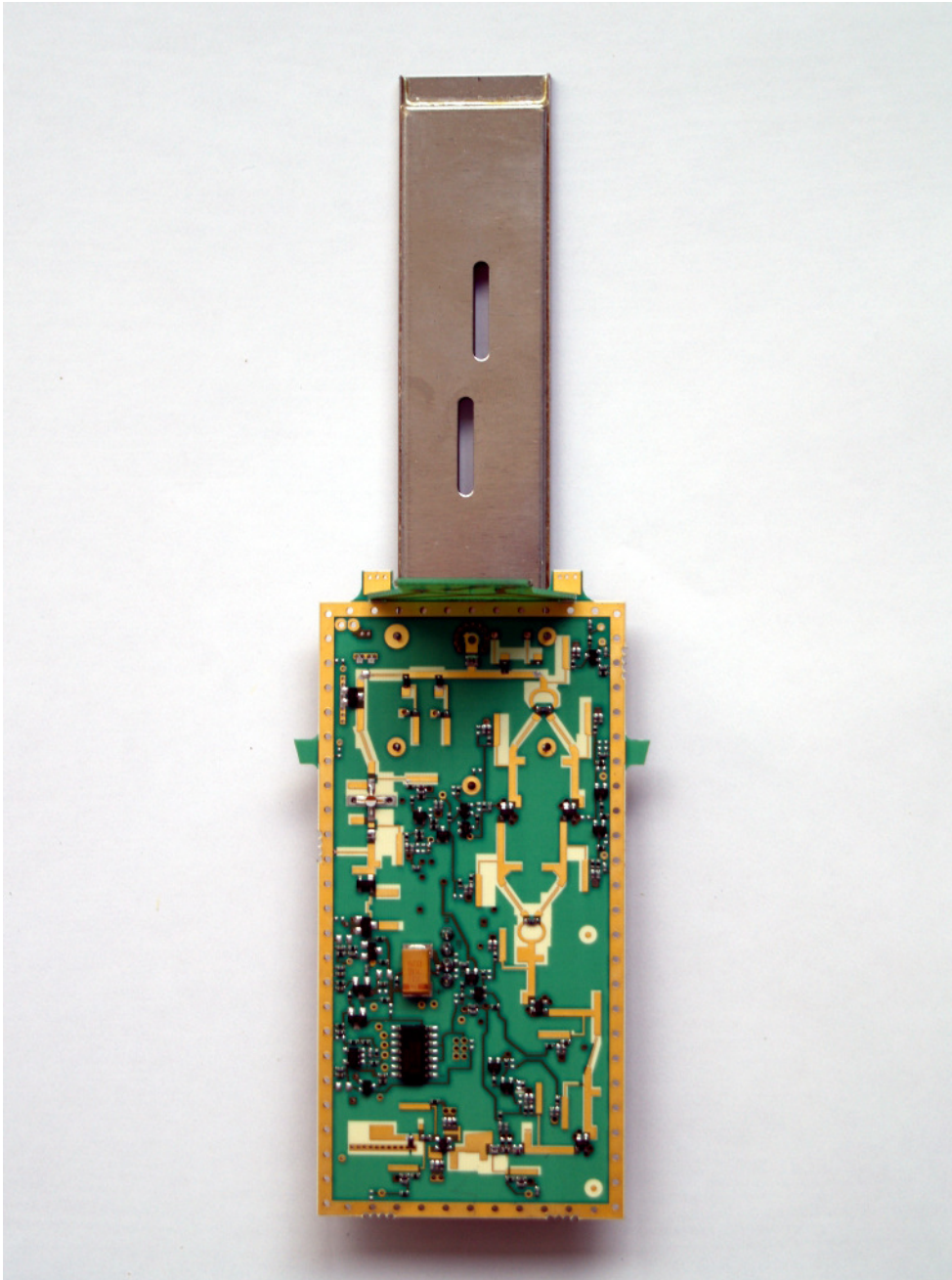
Figure 3: S100 SART PCB – Rear Side with screening can removed
