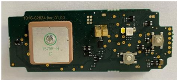
Upper PCB - Top
