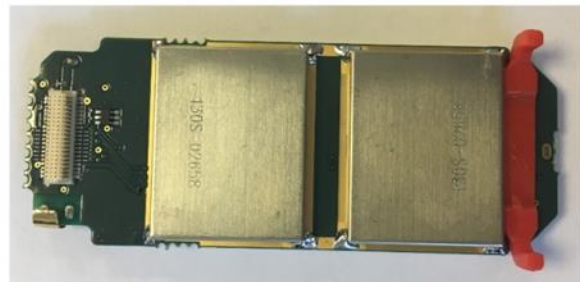
Lower PCB - Top - with Screening Cans
