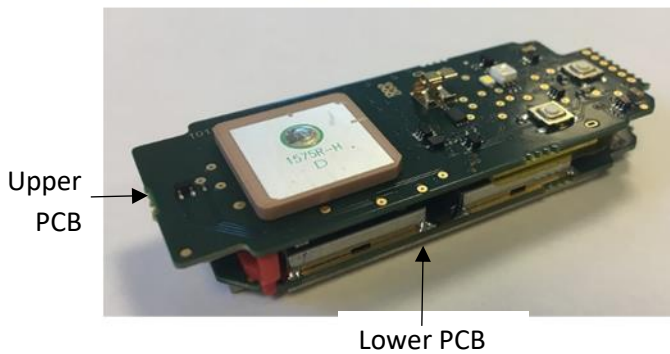
PCB Assembly - Top
