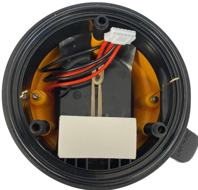
Figure 2: EPIRB2/EPIRB2 Pro – Top view, PCB removed showing battery carrier in-situ.
