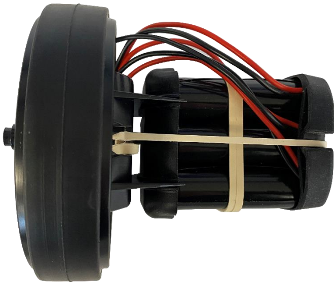
Figure 6: EPIRB2/EPIRB2 Pro – Battery pack in carrier.
