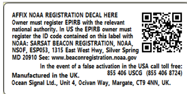
rescueME EPIRB2 PRO - Left Hand Side Label (NOAA / U.S. Coast Guard) (Antenna Not Shown for Clarity)
