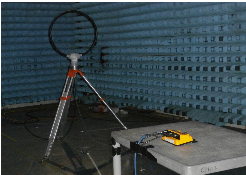
Figure 7 - Test Setup - Radiated Emissions 150 kHz to 30 MHz
