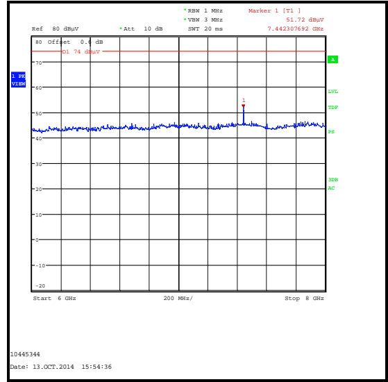
Peak Detector
