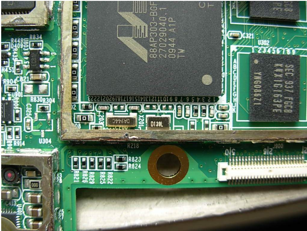
FIGURE 11 ALEX™ READER(M/N: DS-10) CRYSTAL #2 & #3
