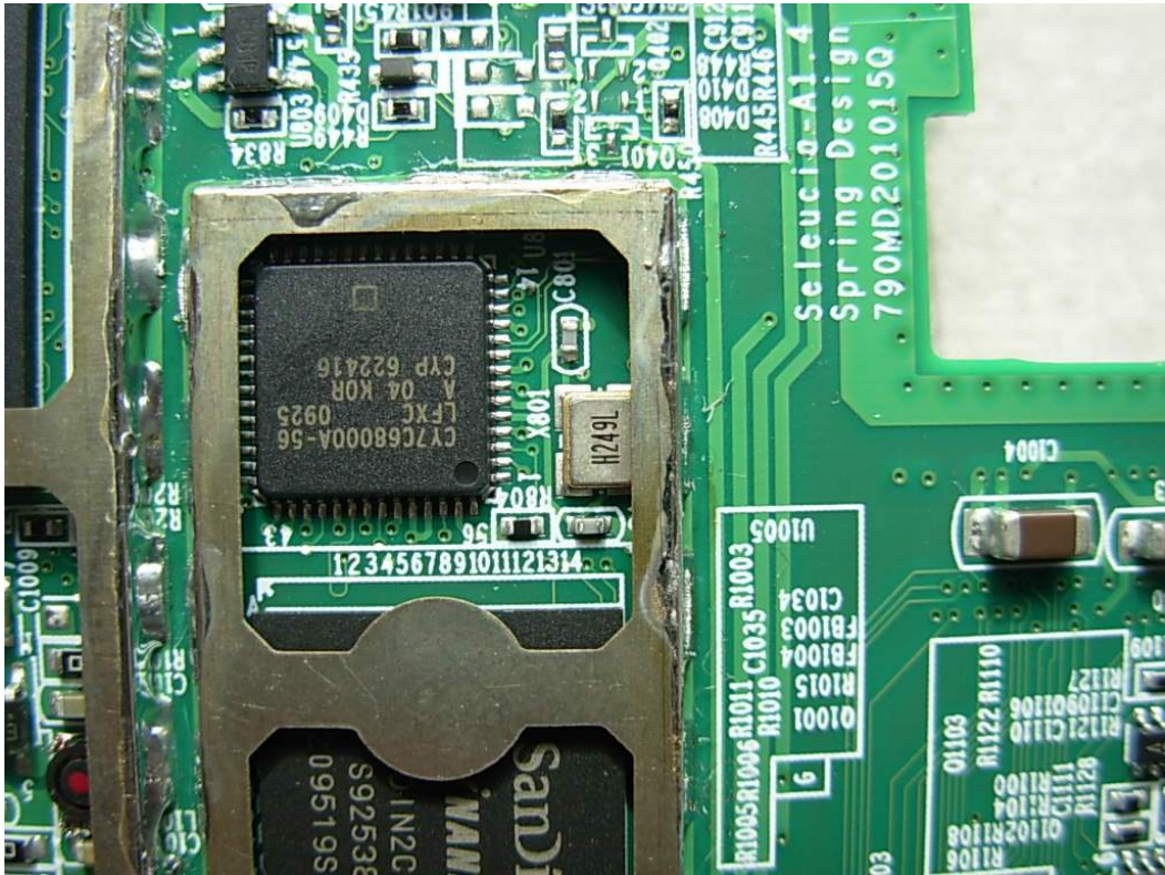
FIGURE 9 ALEX™ READER(M/N: DS-10) CRYSTAL #1
