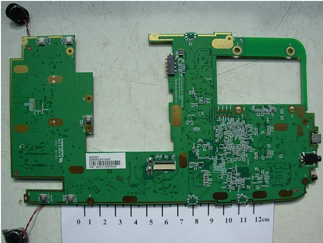
FIGURE 6 ALEX™ READER(M/N: DS-10) MAIN BOARD (SOLDERED SIDE)
