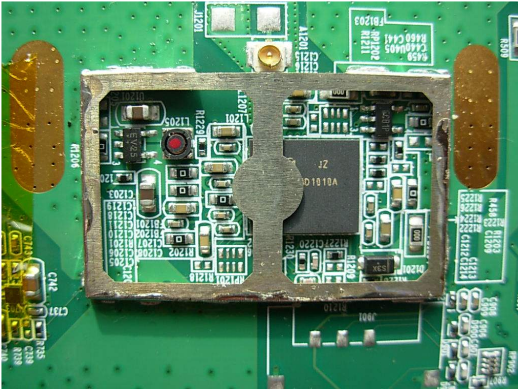
FIGURE 7 ALEX™ READER(M/N: DS-10) MAIN BOARD (INSIDE VIEW#1)
