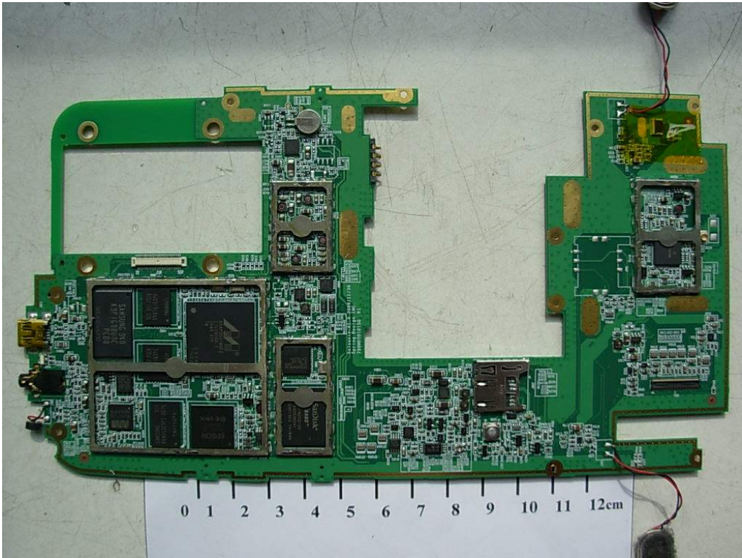
FIGURE 5 ALEX™ READER(M/N: DS-10) MAIN BOARD (COMPONENT SIDE)
