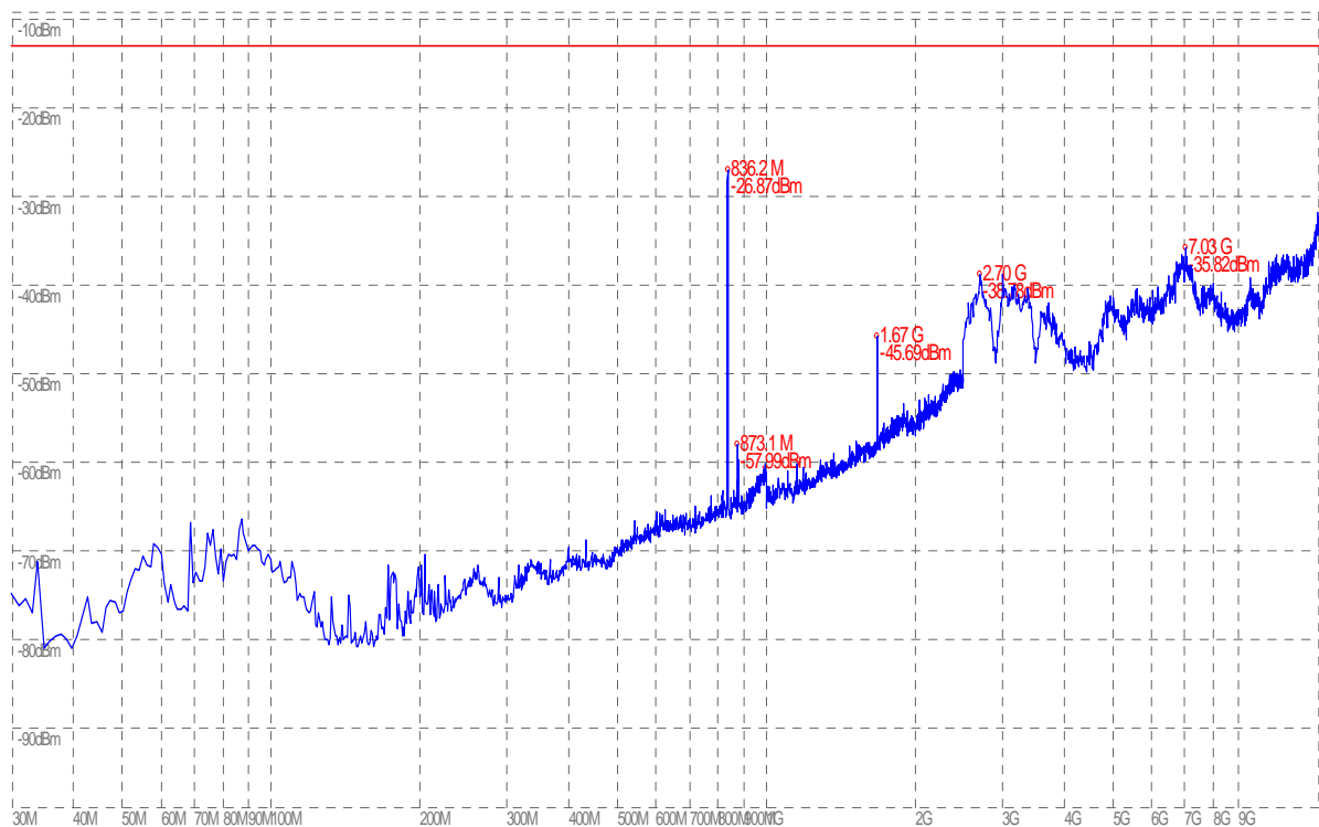
(Plot B.1: GSM 850MHz Channel = 190, Test Antenna Horizontal)
