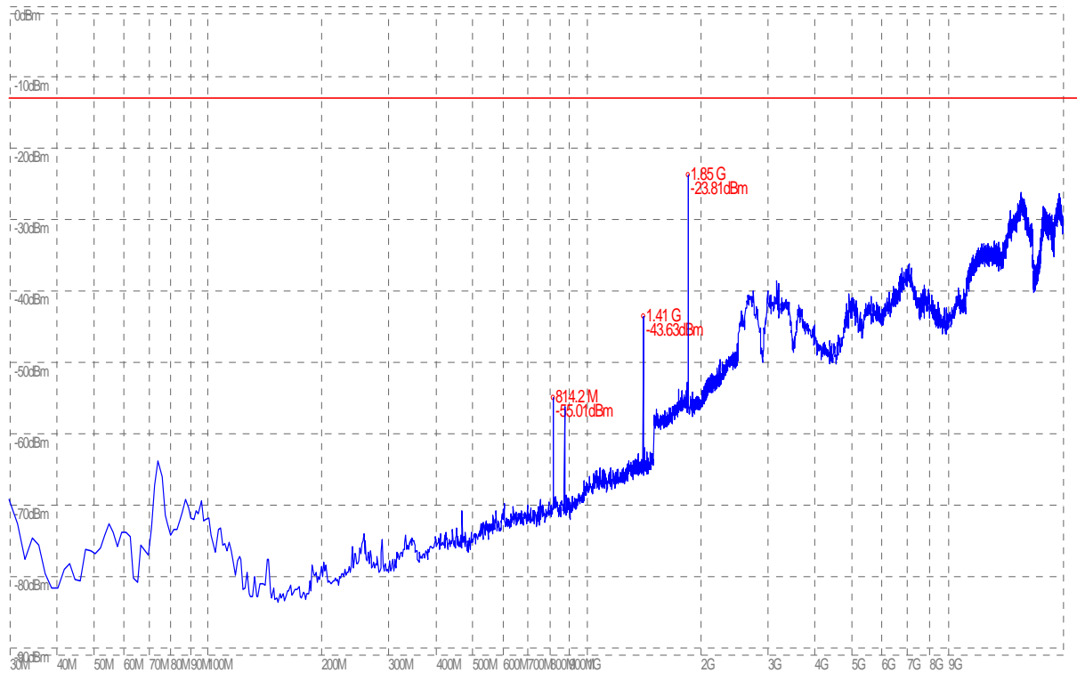
(Plot D.2: GSM 1900MHz Channel = 512, Test Antenna Vertical)
