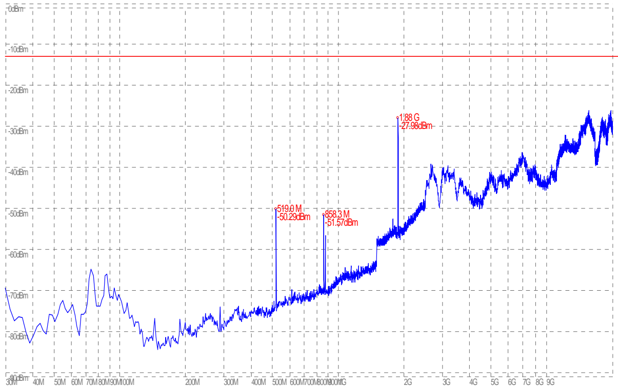
(Plot E.2: GSM 1900MHz Channel = 661, Test Antenna Vertical)
