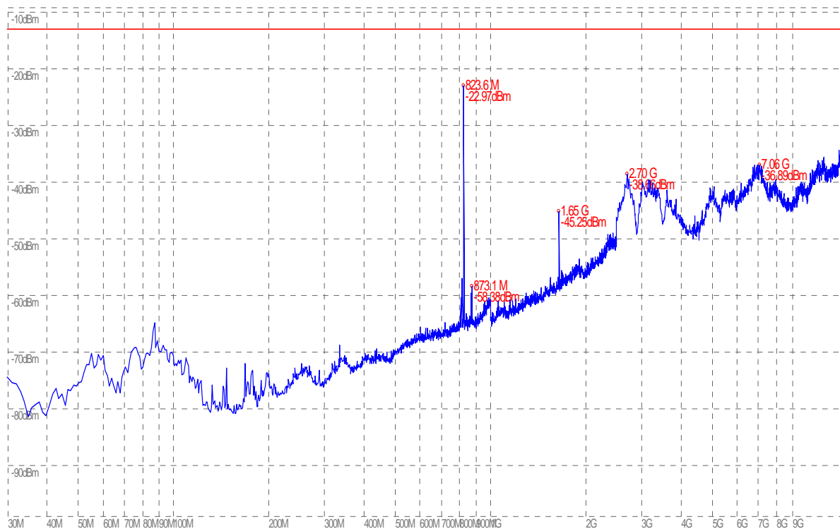
(Plot A.1: GSM 850MHz Channel = 128, Test Antenna Horizontal)
