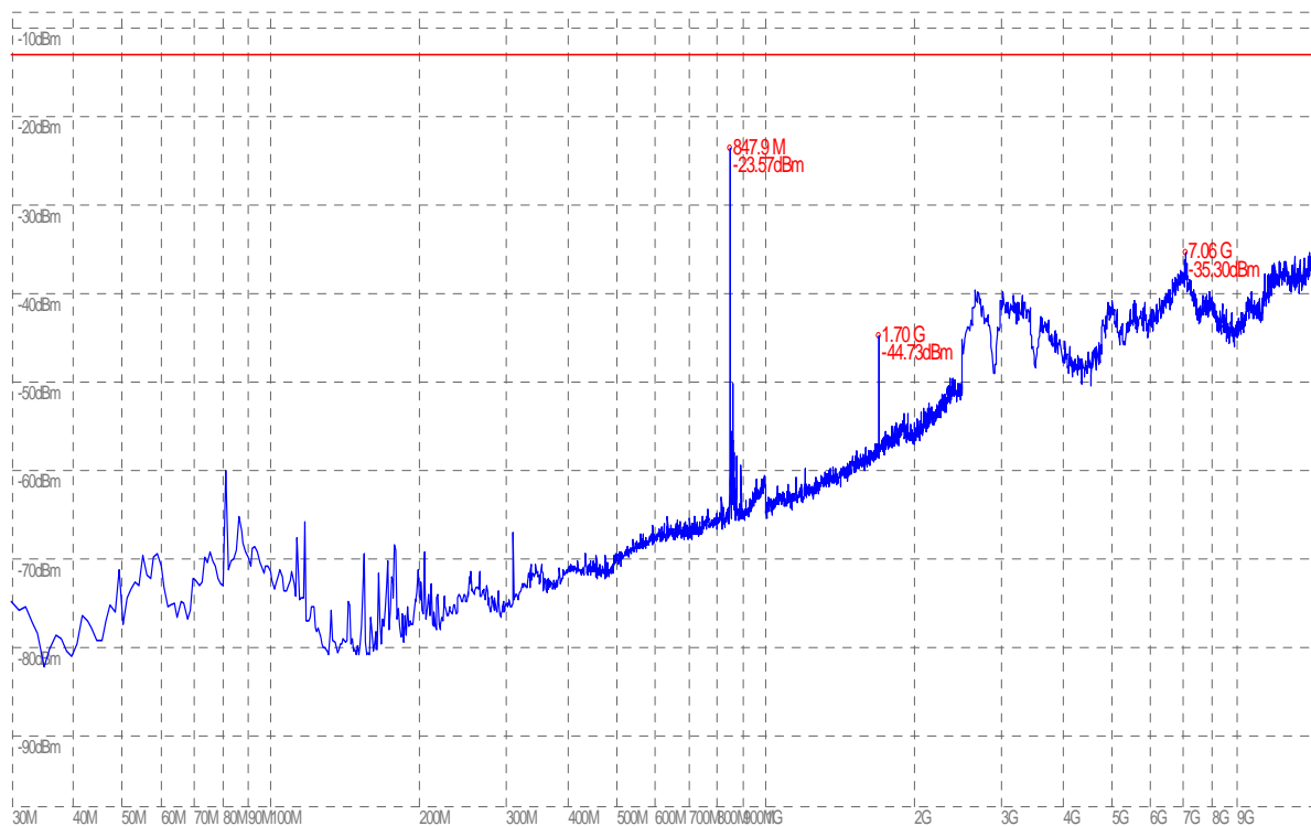
(Plot C.1: GSM 850MHz Channel = 251, Test Antenna Horizontal)
