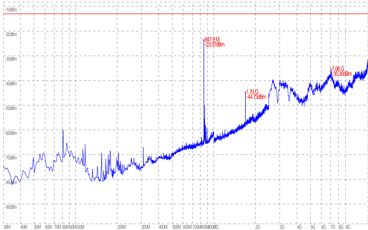
(Plot C.2: GSM 850MHz Channel = 251, Test Antenna Vertical)
