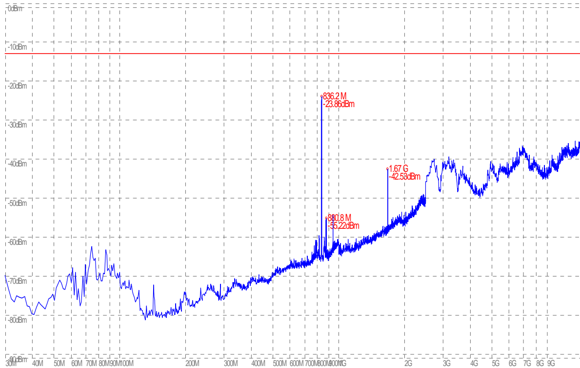
(Plot B.2: GSM 850MHz Channel = 190, Test Antenna Vertical)
