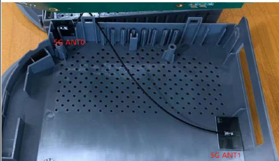
5G WIFI Antenna Location
