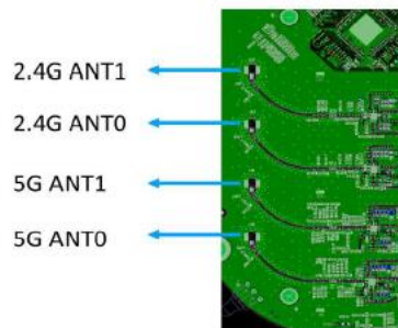
Antenna connection diagram
