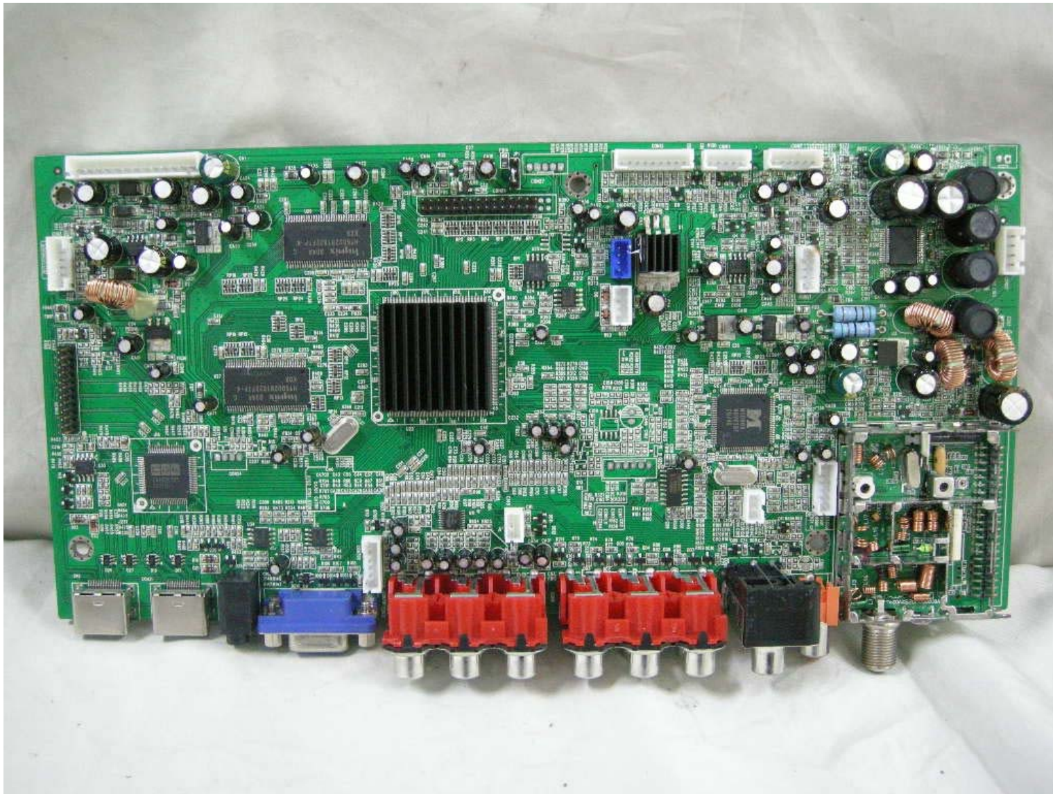
Main Board 1
