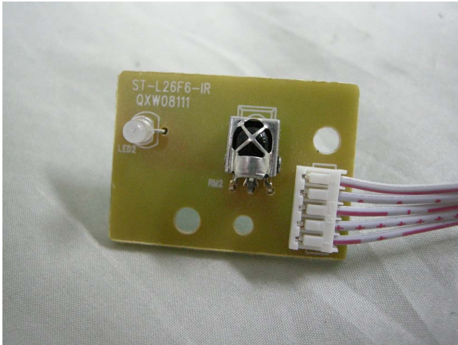
IR board 1
