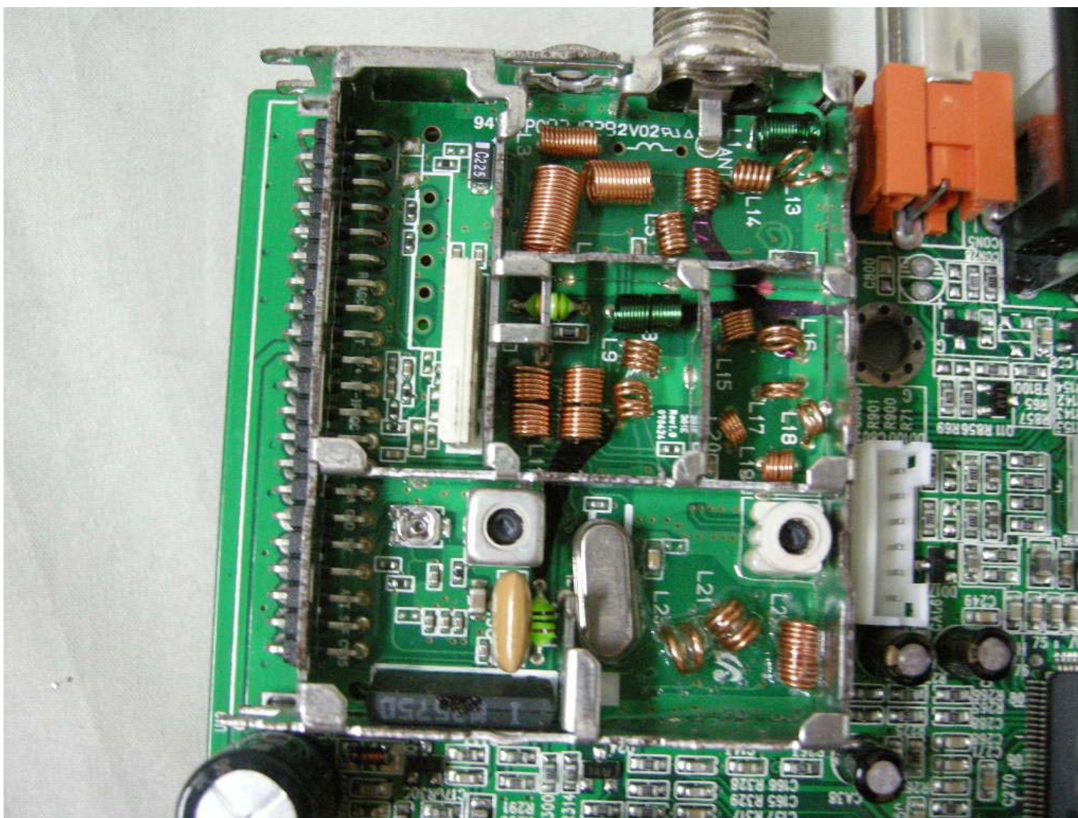
Tuner inside
