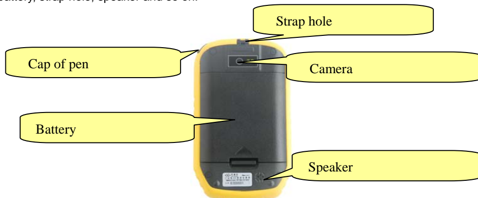
Figure 3-2 Reverse of Qmini Series Industrial GIS Data Collector
