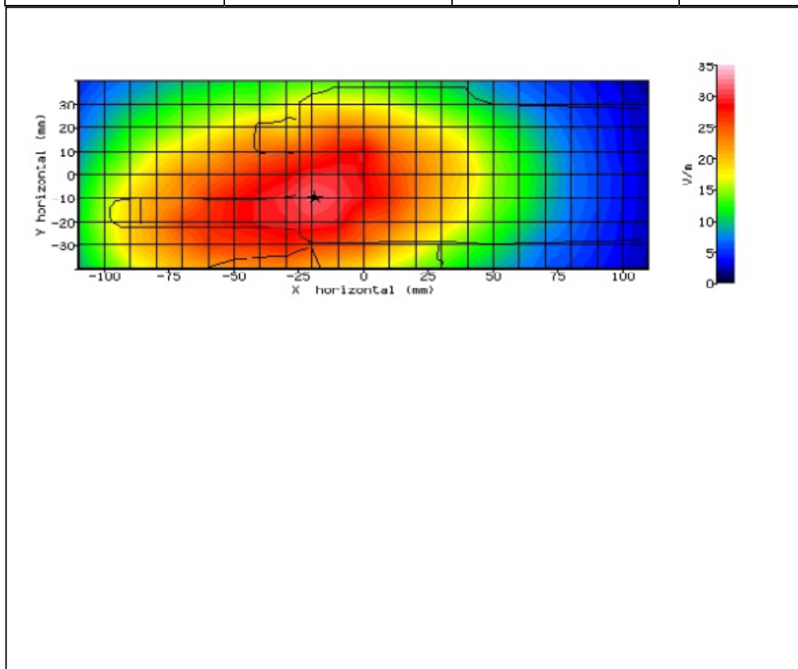
Figure 13: SAR Body Testing Results for the STP9240 TETRA Portable at 470MHz.
