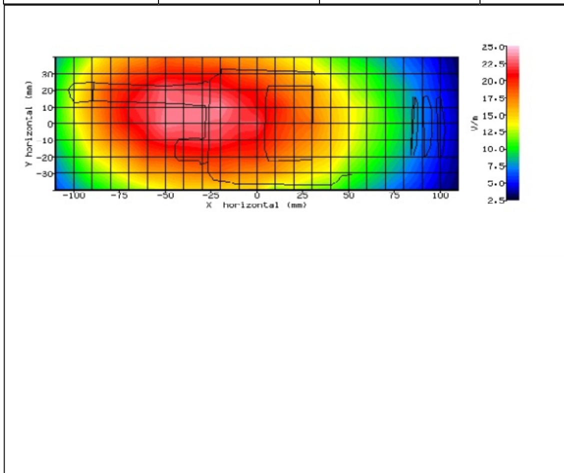
Figure 9: SAR Body Testing Results for the STP9240 TETRA Portable at 430MHz.
