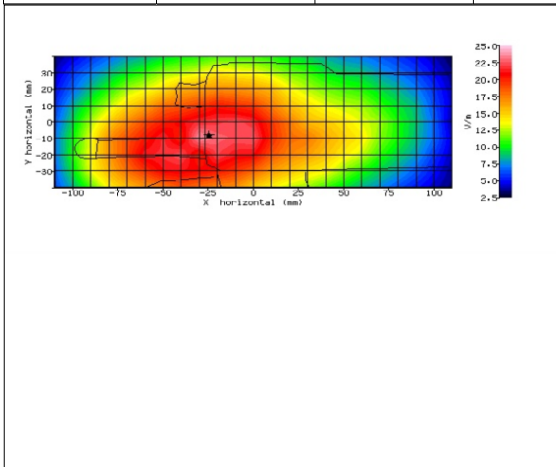
Figure 6: SAR Body Testing Results for the STP9240 TETRA Portable at 430MHz.
