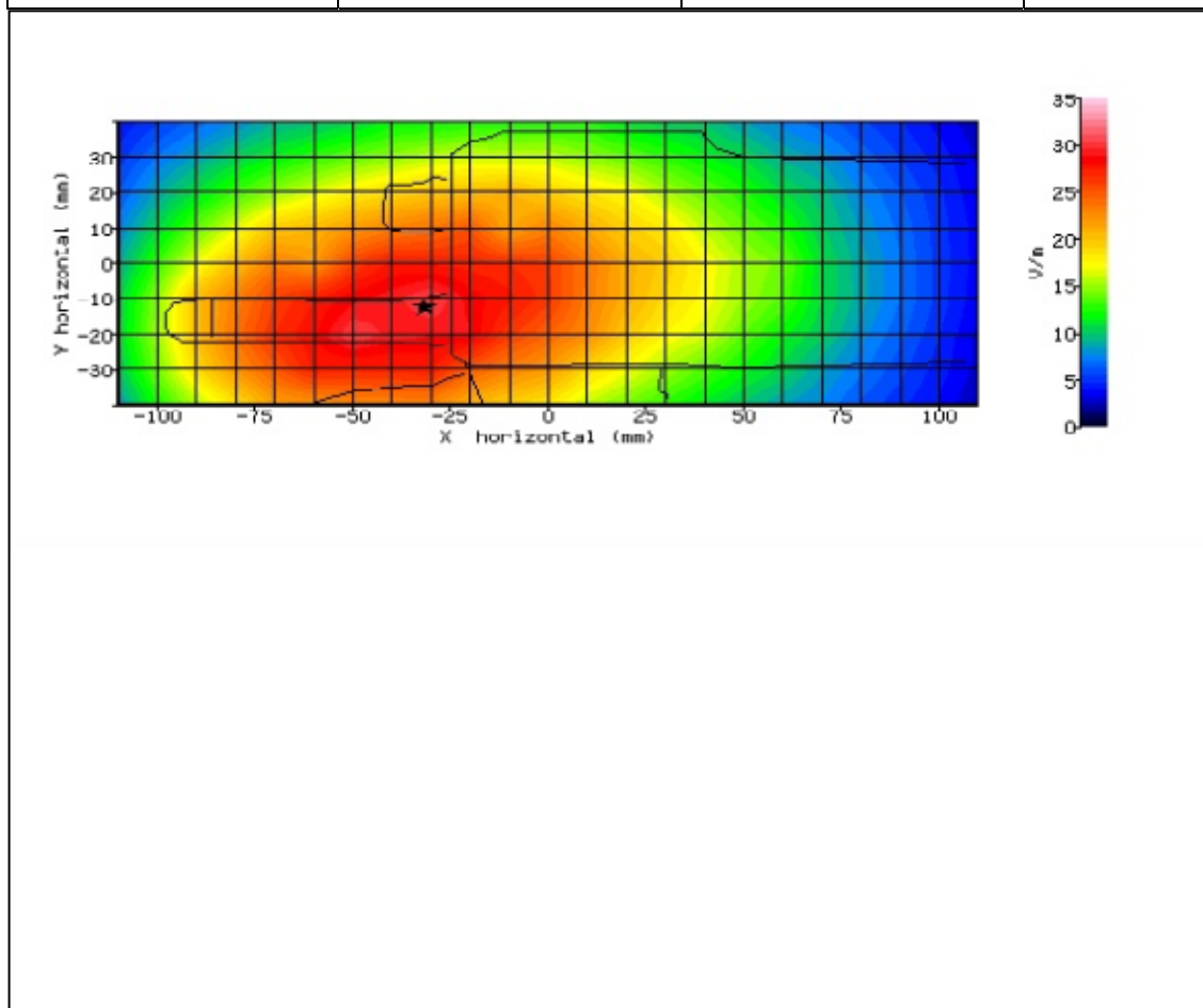
Figure 11: SAR Body Testing Results for the STP9240 TETRA Portable at 470MHz.
