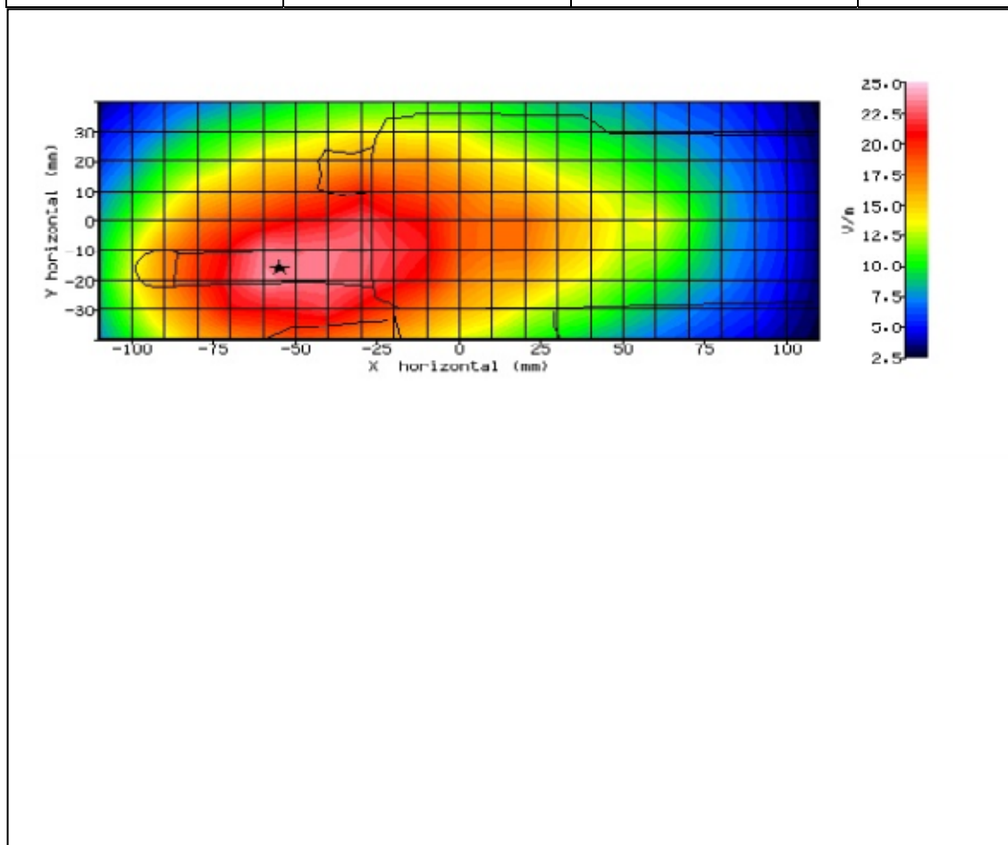
Figure 8: SAR Body Testing Results for the STP9240 TETRA Portable at 430MHz.
