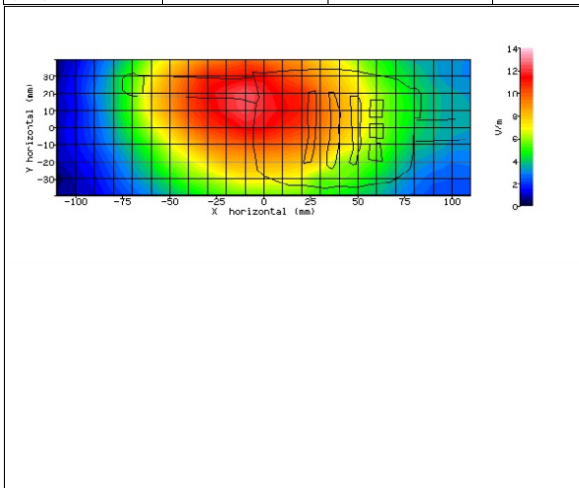
Figure 18: SAR Body Testing Results for the STP9240 TETRA Portable at 470MHz.
