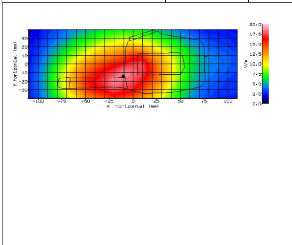
Figure 7: SAR Body Testing Results for the STP9240 TETRA Portable at 430MHz.
