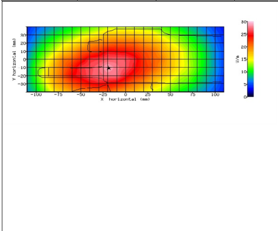
Figure 14: SAR Body Testing Results for the STP9240 TETRA Portable at 470MHz.
