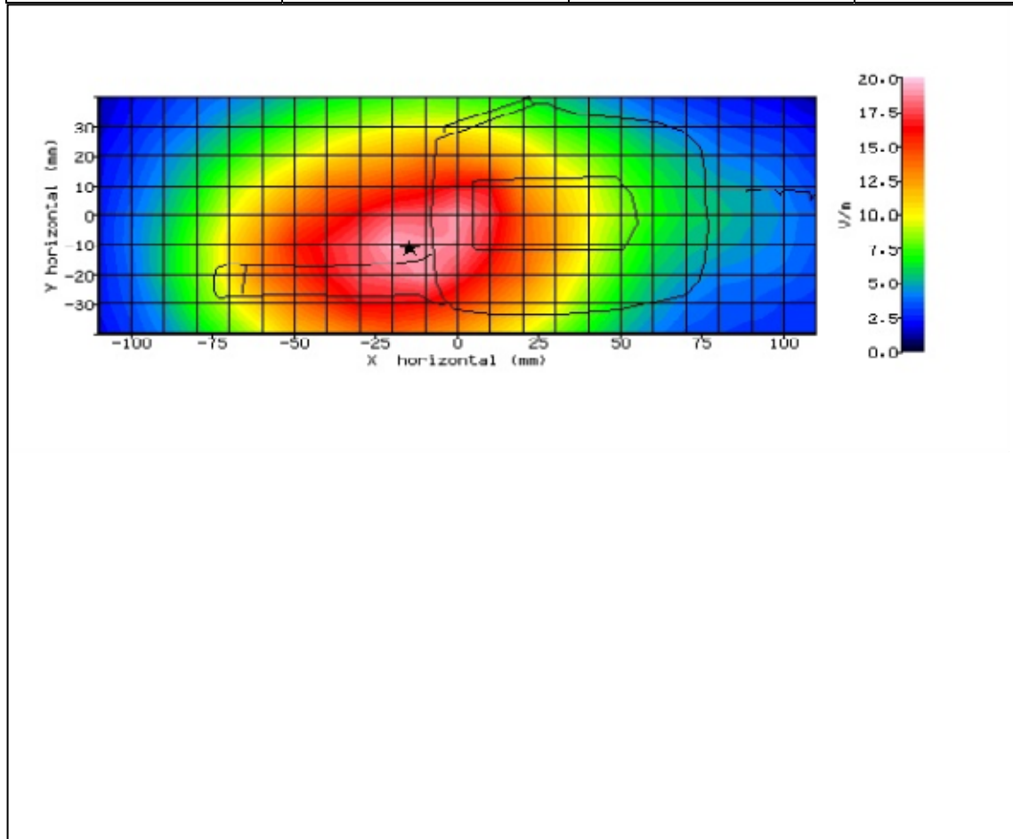
Figure 15: SAR Body Testing Results for the STP9240 TETRA Portable at 470MHz.
