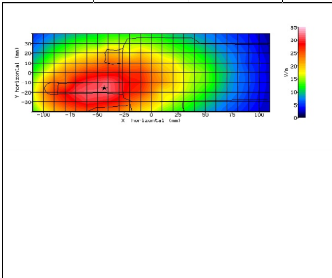
Figure 3: SAR Body Testing Results for the STP9240 TETRA Portable at 430MHz.
