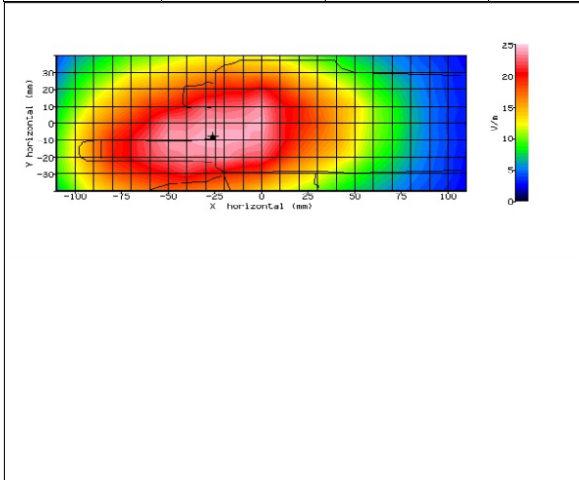
Figure 16: SAR Body Testing Results for the STP9240 TETRA Portable at 470MHz.
