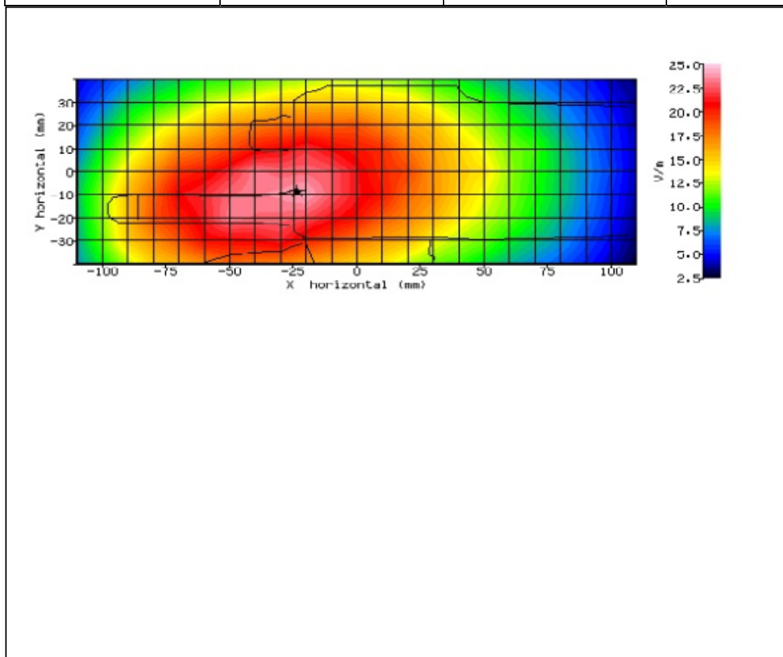
Figure 12: SAR Body Testing Results for the STP9240 TETRA Portable at 470MHz.
