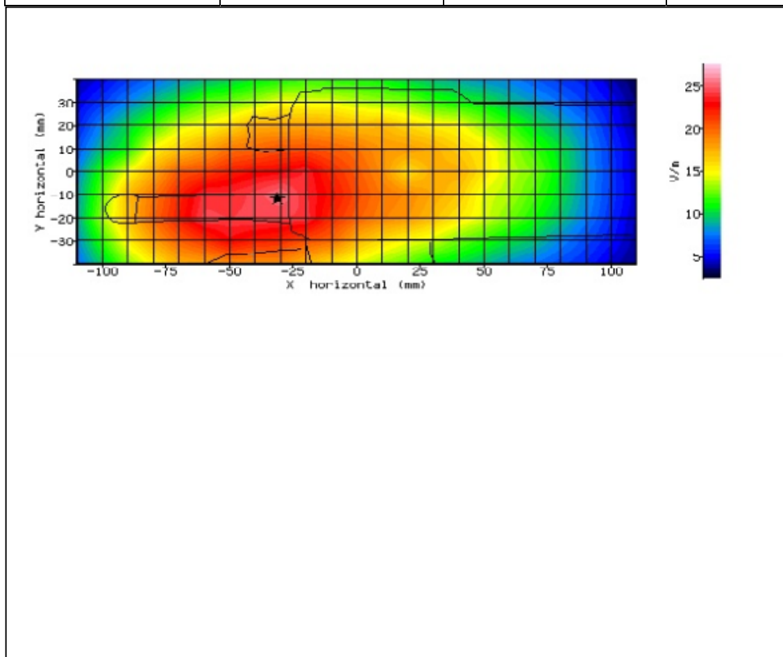
Figure 5: SAR Body Testing Results for the STP9240 TETRA Portable at 430MHz.
