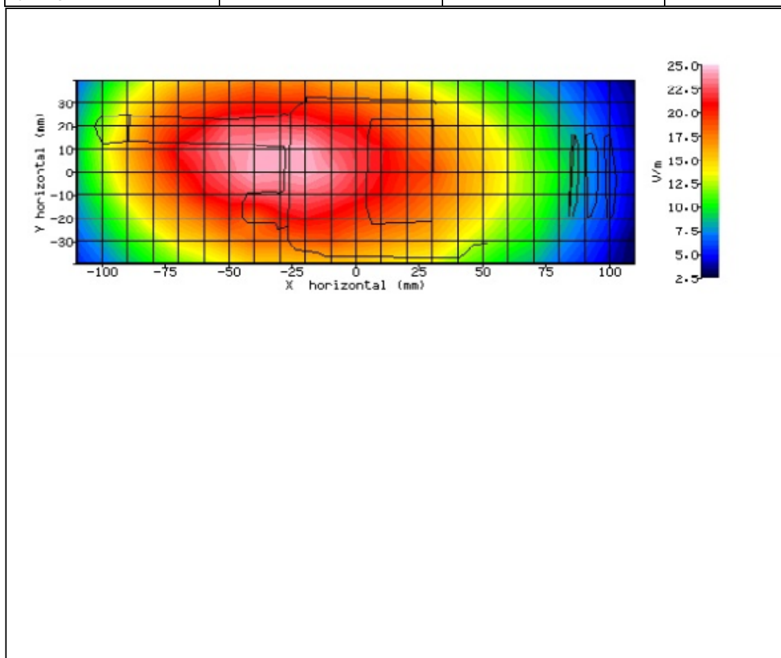
Figure 17: SAR Body Testing Results for the STP9240 TETRA Portable at 470MHz.
