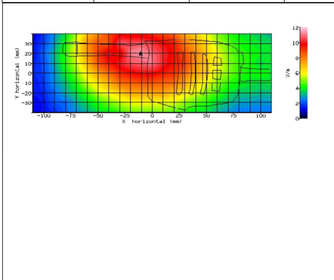
Figure 10: SAR Body Testing Results for the STP9240 TETRA Portable at 430MHz.
