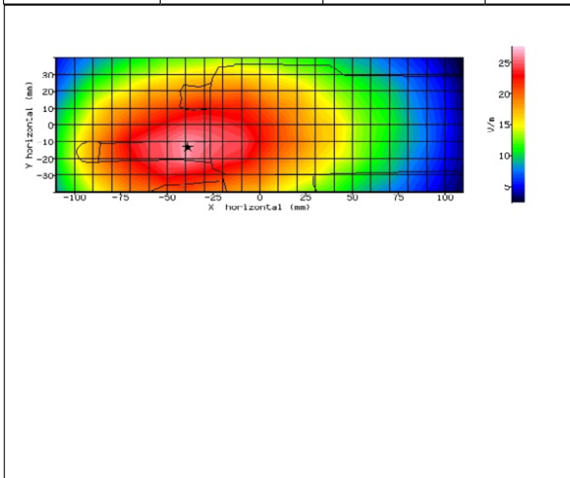
Figure 4: SAR Body Testing Results for the STP9240 TETRA Portable at 430MHz.
