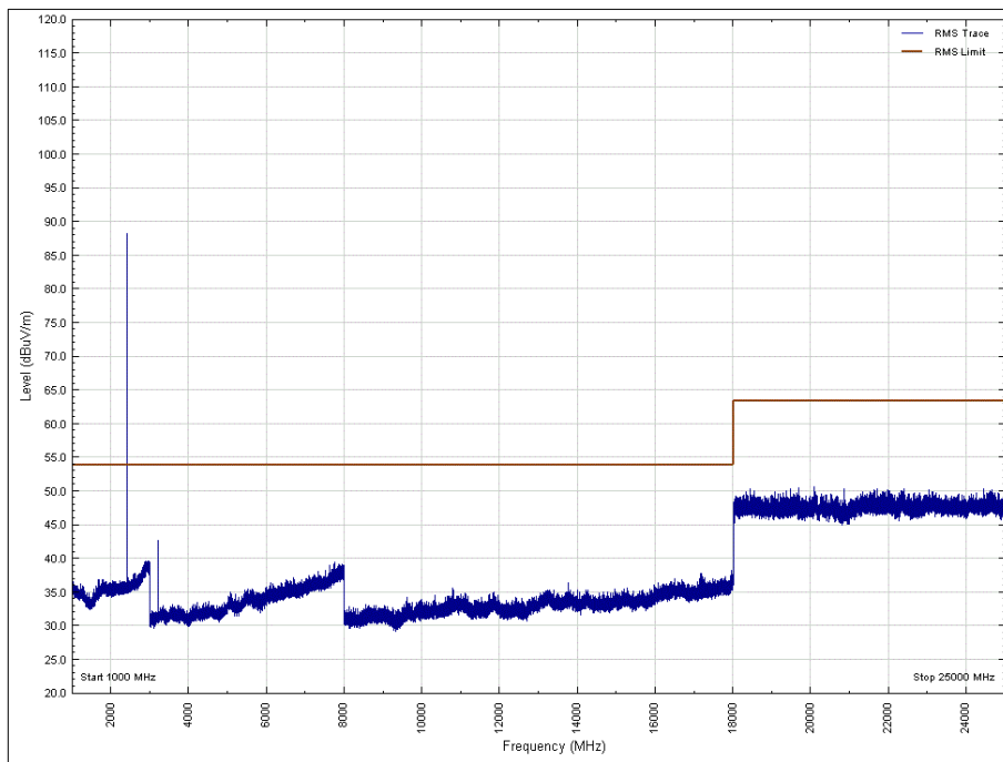
Figure 44 - 2402 MHz, 1 GHz to 25 GHz, Horizontal, X Orientation - Average
