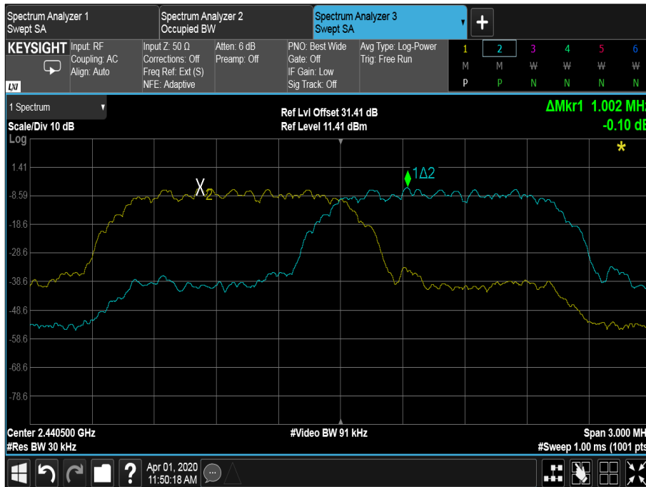
Figure 21 - \pi/4 DQPSK
