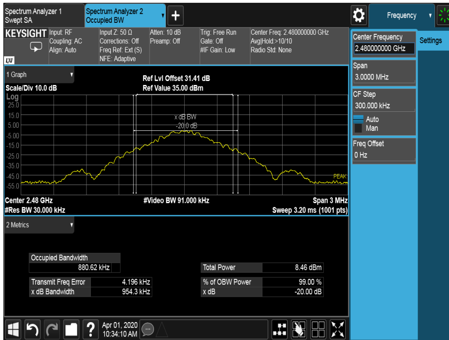
Figure 29 - 2480 MHz - GFSK
