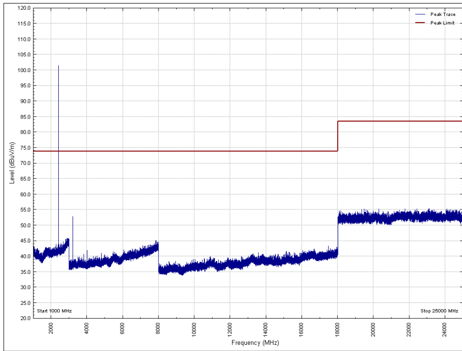
Figure 41 - 2402 MHz, 1 GHz to 25 GHz, Vertical, X Orientation - Peak
