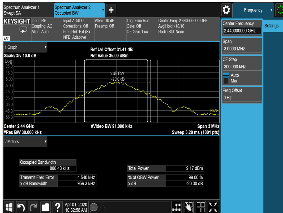
Figure 26 - 2440 MHz - GFSK
