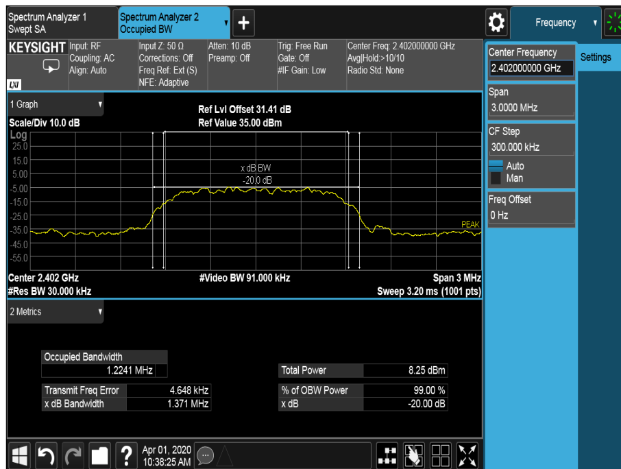
Figure 24 - 2402 MHz - \pi/4 DQPSK
