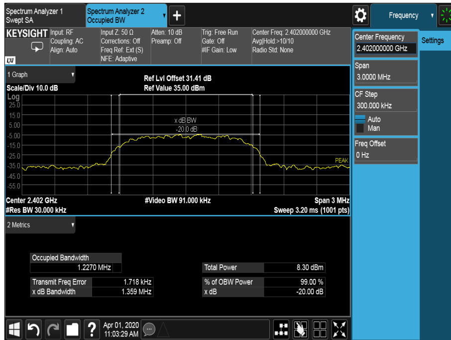
Figure 25 - 2402 MHz - 8-DPSK
