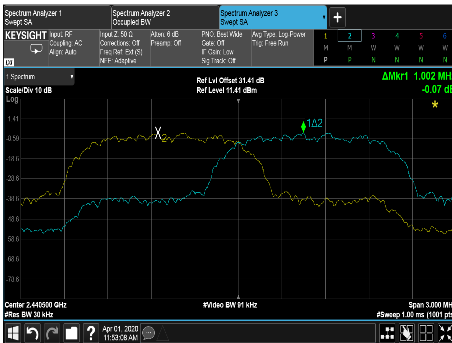
Figure 22 - 8-DPSK
