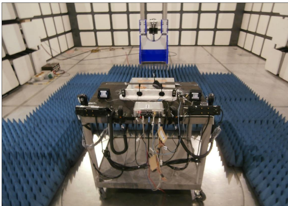
Figure 9 - Test Setup - 1 GHz to 8 GHz
