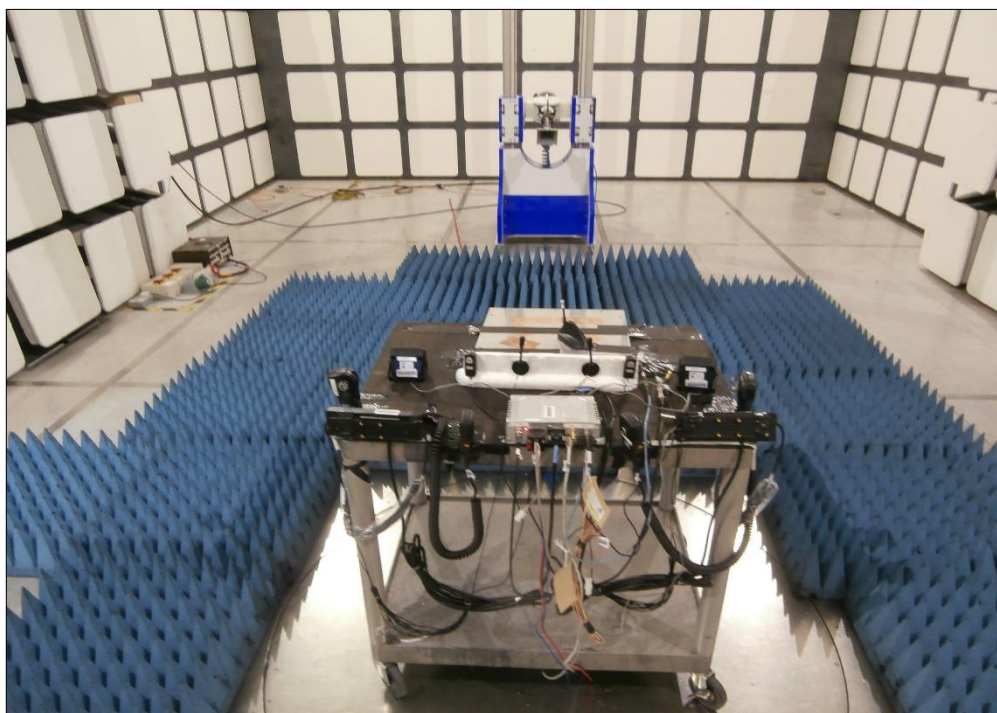
Figure 10 - Test Setup - 8 GHz to 13 GHz
