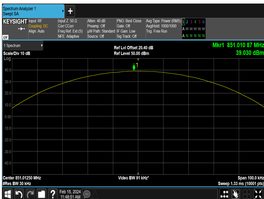
Figure 4 - 851.0125 MHz
