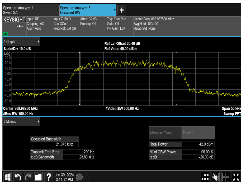
Figure 18- 868.9875 MHz FCC 47 CFR Part 90, Limit Clause 90.209
