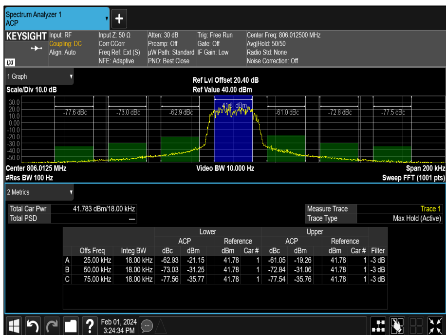
Figure 80 - 806.0125 MHz
