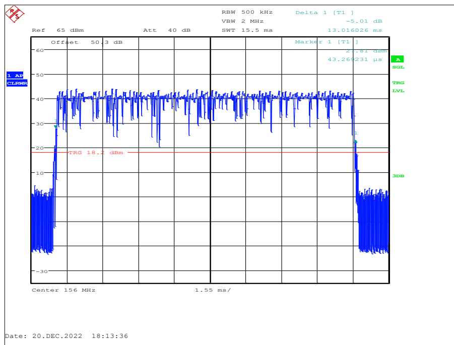
Figure 51 Burst Length
