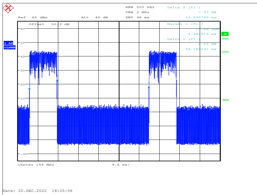
Figure 52 Transmission Characteristics
