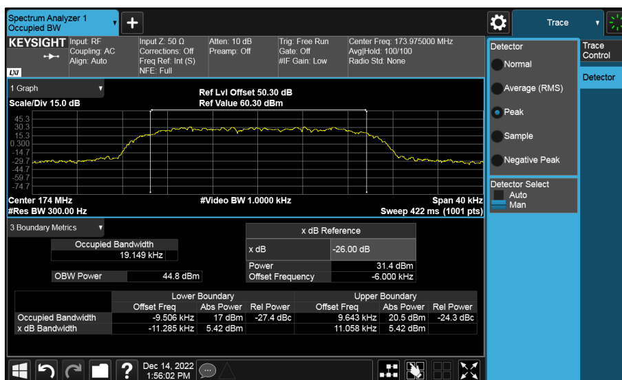
Figure 6 - 173.975 MHz Occupied Bandwidth
