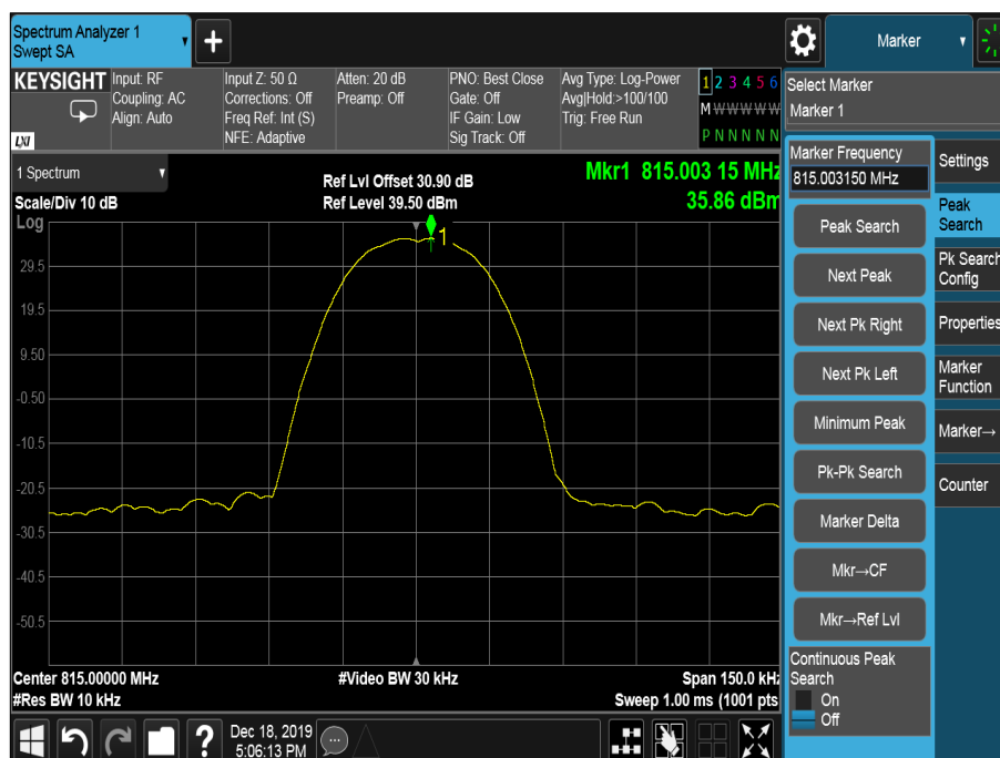
Figure 57 - Frequency Spectrum
