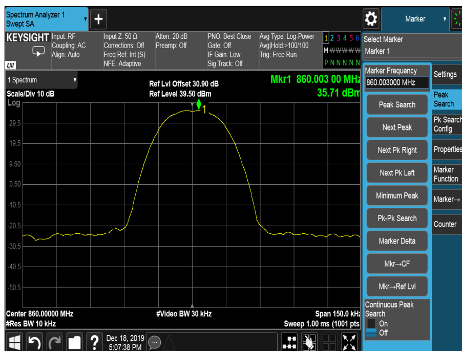
Figure 60 - Frequency Spectrum
