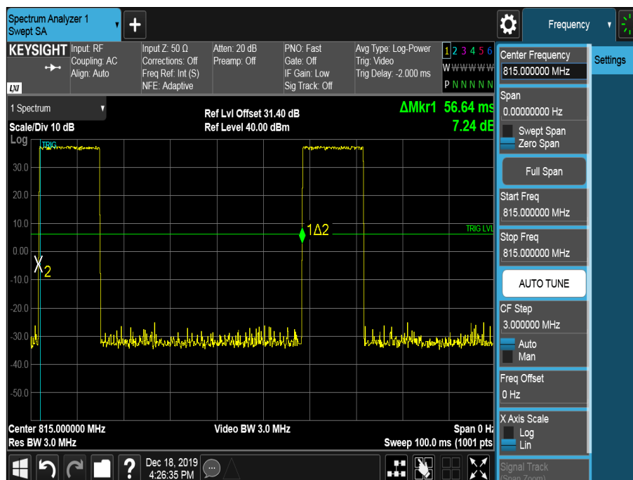
Figure 56 - Burst Period
