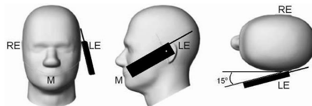
Figure 7: "Tilted" position of DUT
