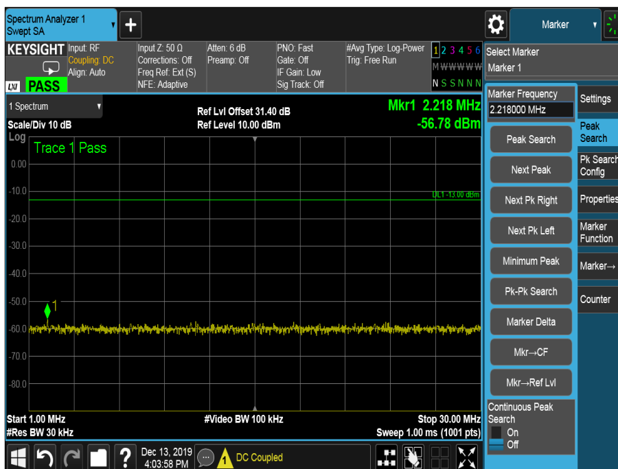
Figure 36 - 429.975 MHz - 1 MHz to 30 MHz
