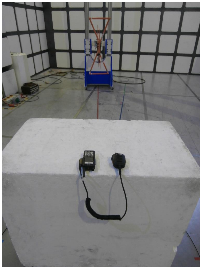
Figure 103 – 30 MHz to 1 GHz, EUT Orientation: X
