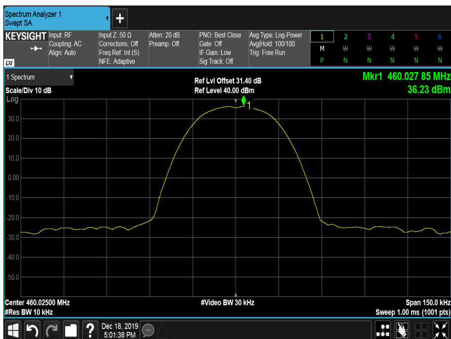
Figure 63 - Frequency Spectrum
