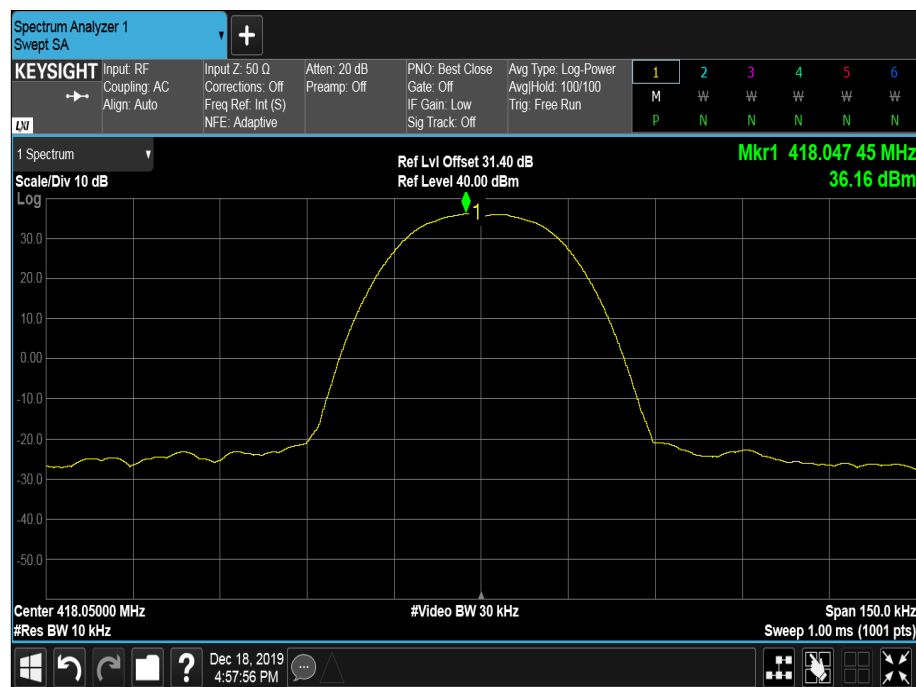
Figure 66 - Frequency Spectrum
