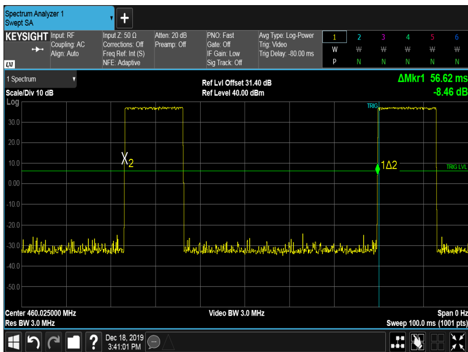
Figure 62 - Burst Period
