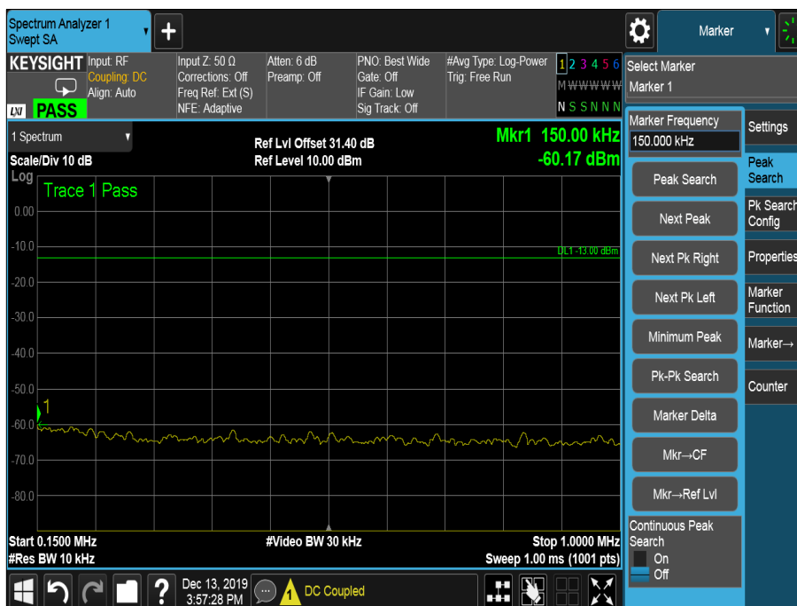
Figure 31 - 406.125 MHz, 150 kHz to 1 MHz
