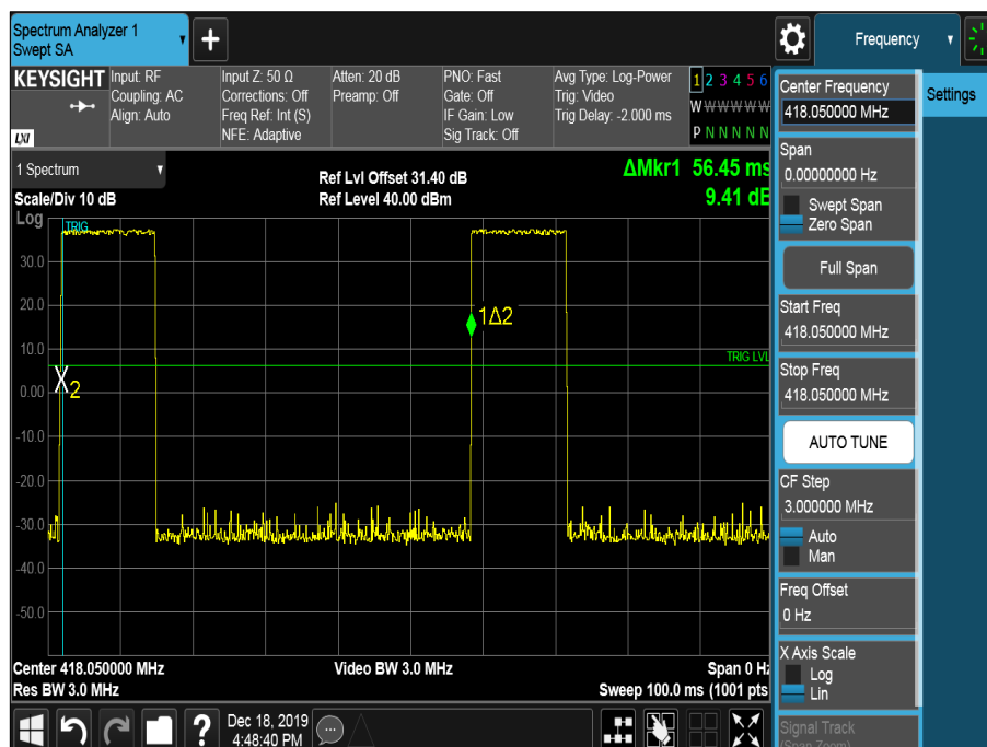
Figure 65 - Burst Period
