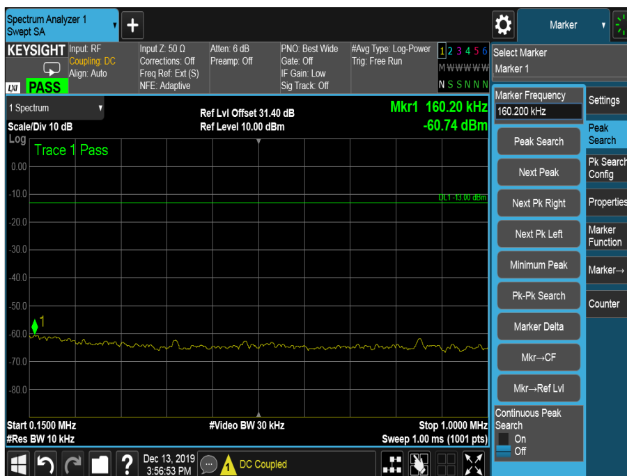
Figure 32 - 418.050 MHz, 150 kHz to 1 MHz
