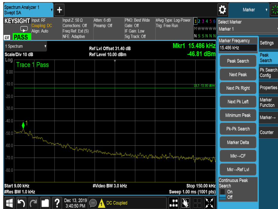
Figure 29 - 418.050 MHz, 9 kHz to 150 kHz
