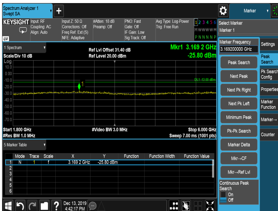
Figure 41 - 418.050 MHz, 1.8 GHz to 6 GHz
