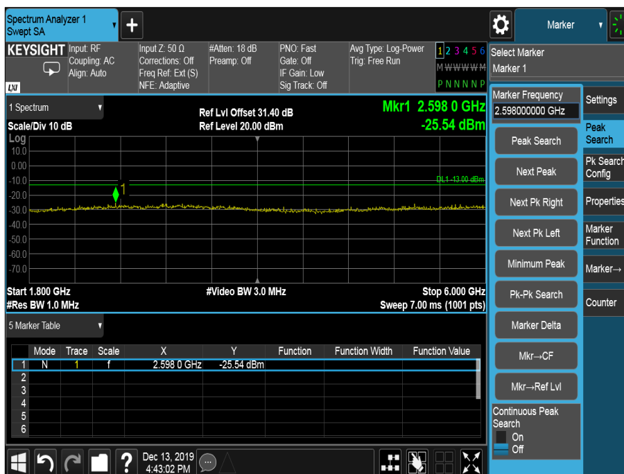
Figure 40 - 406.125 MHz, 1.8 GHz to 6 GHz
