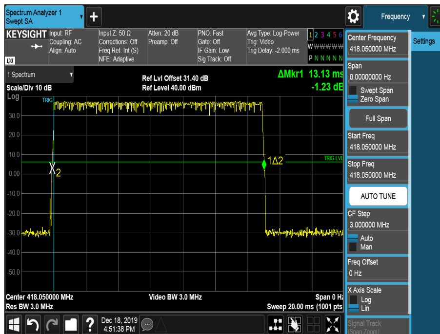
Figure 64 - Burst Length
